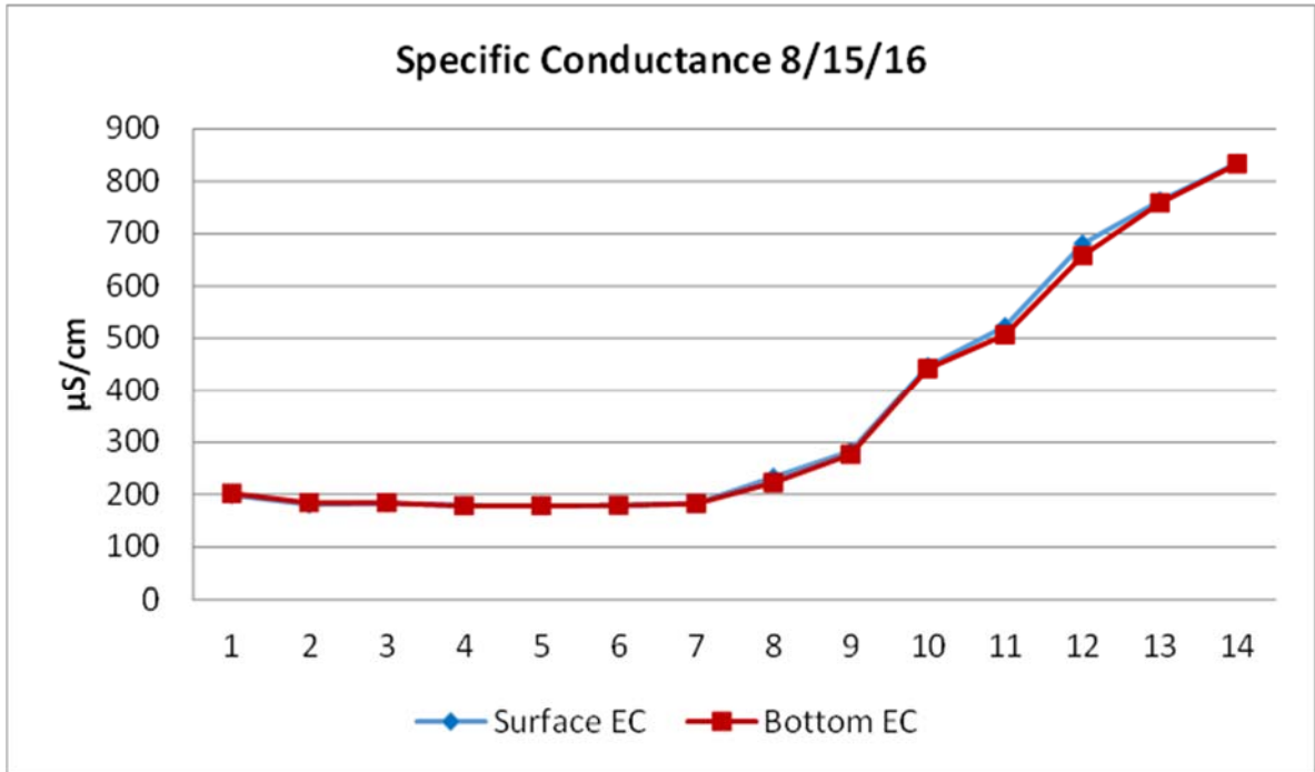
Figure 3. Specific Conductance of the DWSC on 8/15/16 [from: jenna.rinde@water.ca.gov]
