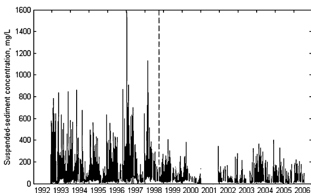
Fig. 4 Suspended-sediment concentration, mid-depth, Point San Pablo. The vertical dashed line indicates when the step decrease occurred
