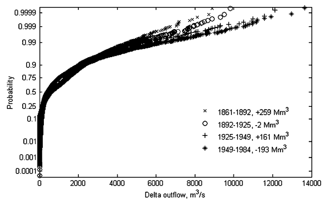
Fig. 7 Probability of flow exceedance for Delta outflow for the periods between the midpoints of San Francisco Bay bathymetric surveys. Daily flow data are from Ganju et al. (2008). Bay sediment volume change is given in the legend. The probability that a given extremely large freshwater inflow will be exceeded has increased with time. Changes in freshwater inflow cannot explain the variation in bay sediment volume
