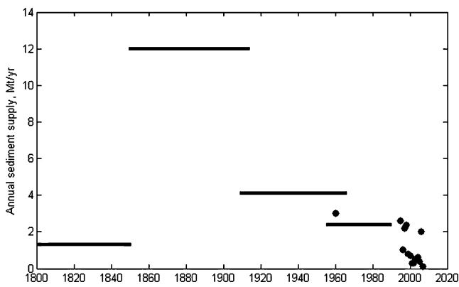
Fig. 3 Estimated annual sediment supply from the Central Valley to San Francisco Bay. Estimates from Gilbert (1917), Krone (1979), Porterfield (1980), Ogden Beeman and Associates (1992), McKee et al. (2006), and David et al. (2009). Bars indicate estimates over entire period, and points indicate yearly estimates. A bulk density of 850 \text{ kg/m}^3 was assumed (Porterfield 1980)
