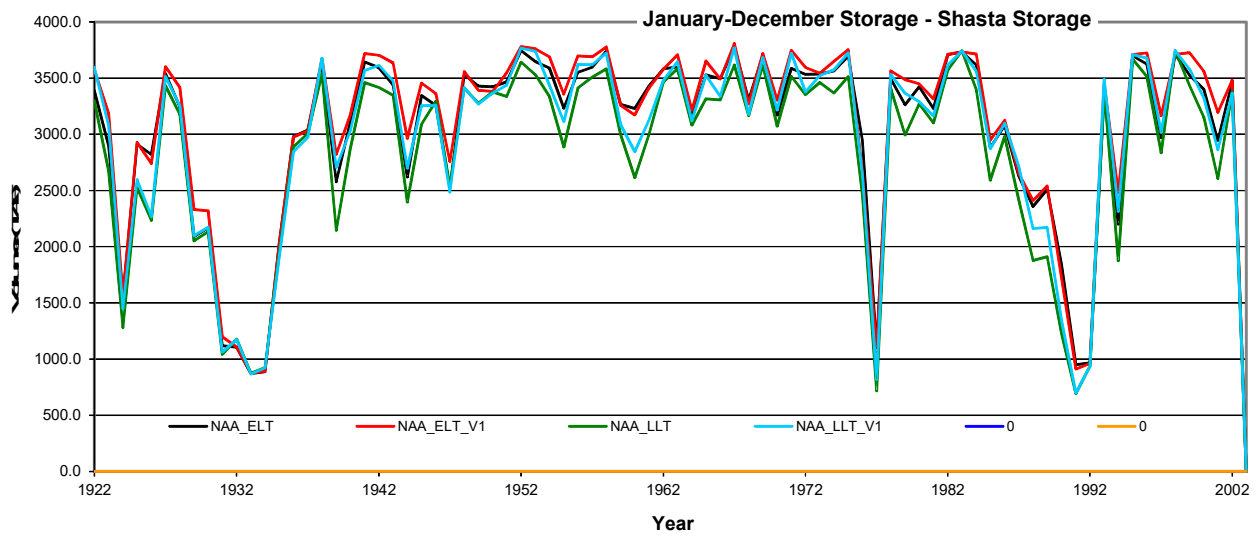
Time series
