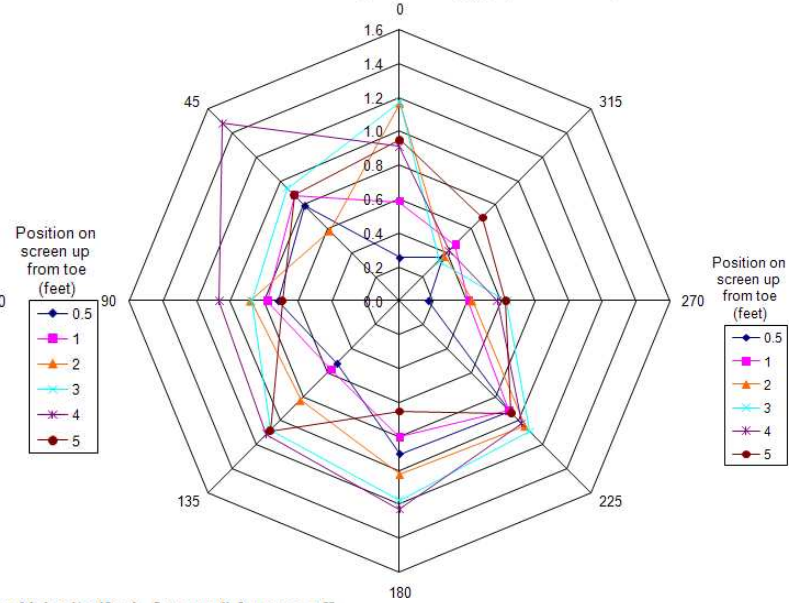
Sweeping Velocity (fps), Screen # 9 pump off
