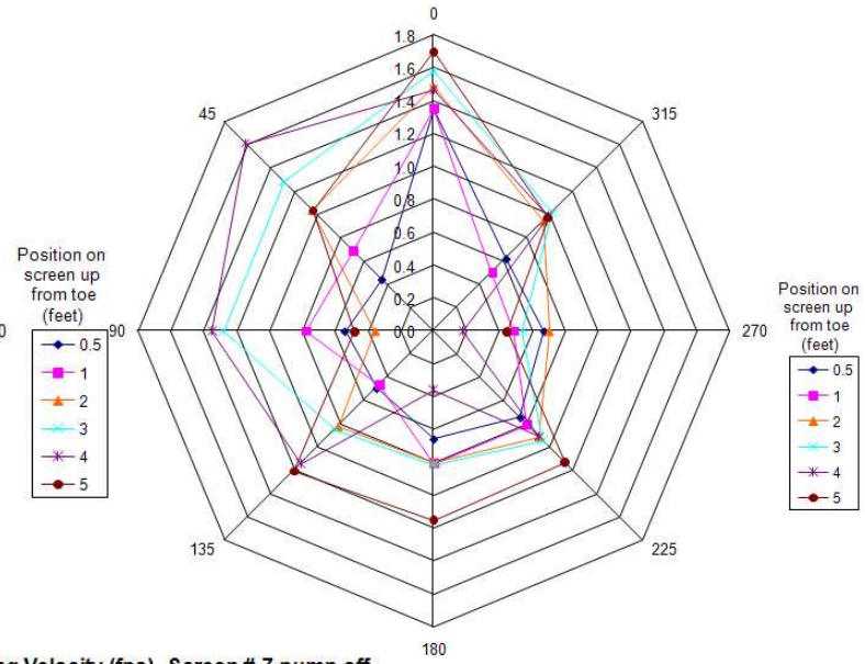
Sweeping Velocity (fps), Screen # 7 pump off
