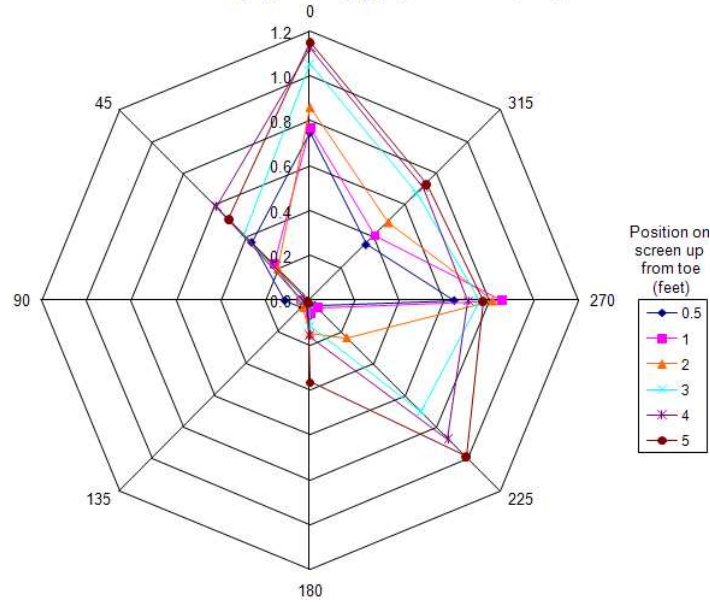
Sweeping Velocity (fps), Screen # 9 pump off
