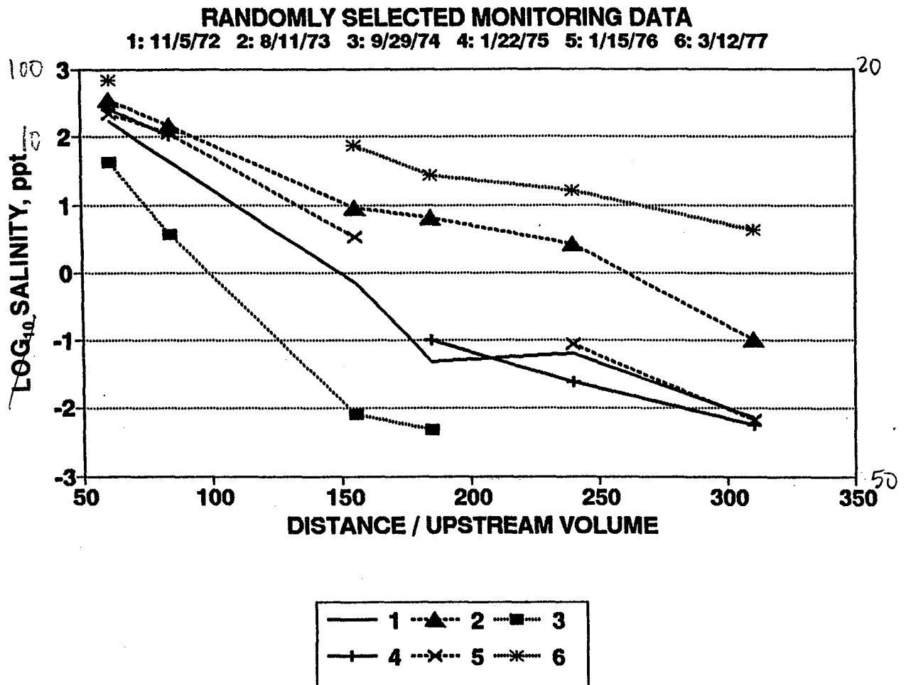
Figure 3. Representative continuous monitoring data used in interpolation. The data have been straightened out to the degree possible by log-transforming salinity and converting the distance measure to distance/upstream volume.
