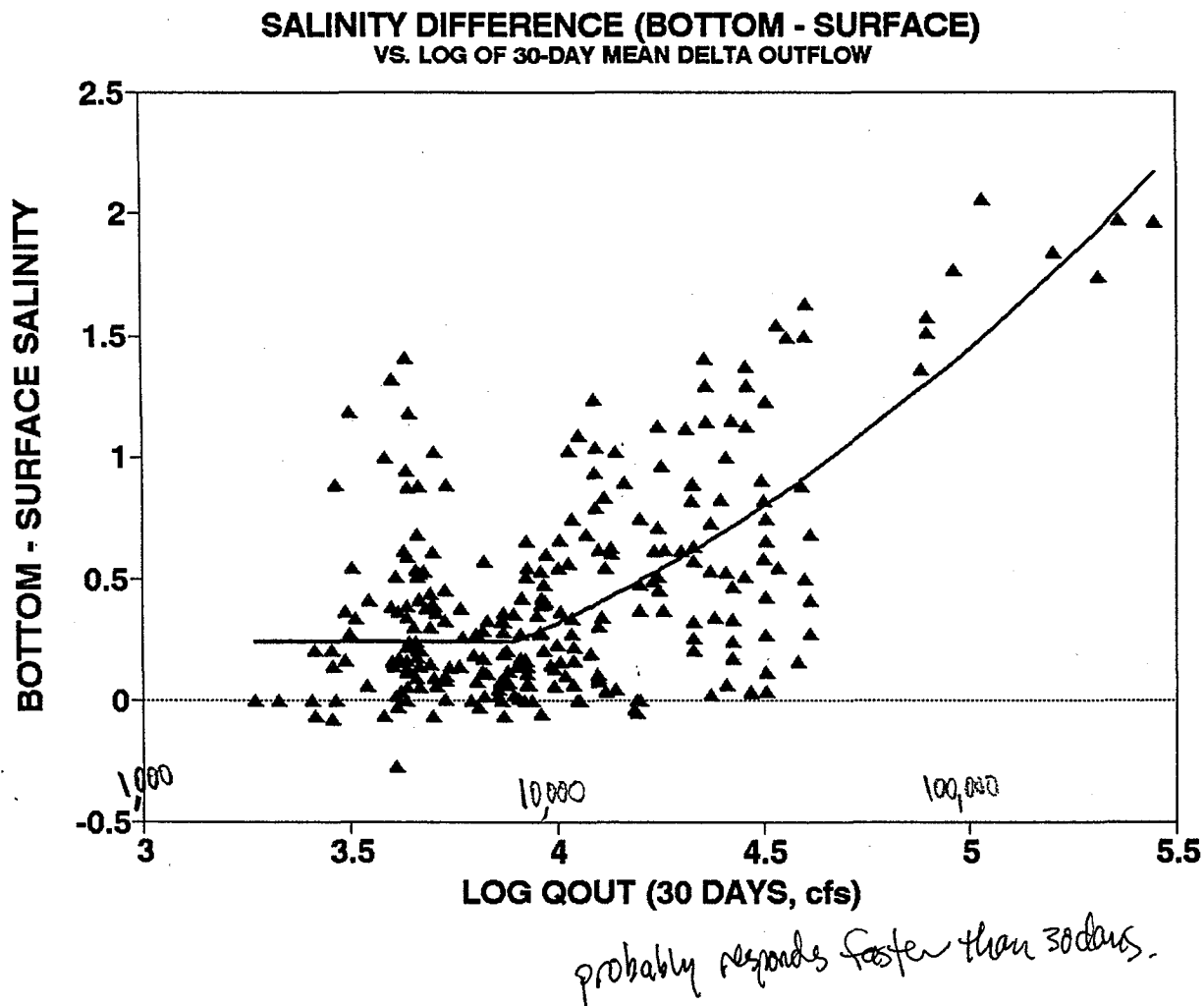
Figure 2. Difference between surface and bottom salinity for grab sample data for which bottom salinity was 1.5-2.5 ppt, vs. log net delta outflow averaged over previous 30 days. The regression line is a quadratic relationship with log Q_{out} constrained to a minimum of 0.24 ppt.
