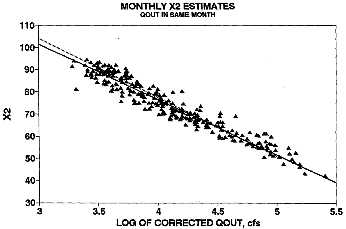
Figure 13. Monthly means of X_2 plotted against mean Q_{out} for the same month. Solid line, geometric mean regression; dashed line, equation of Williams and Hollibaugh (1987 Figure 23).
