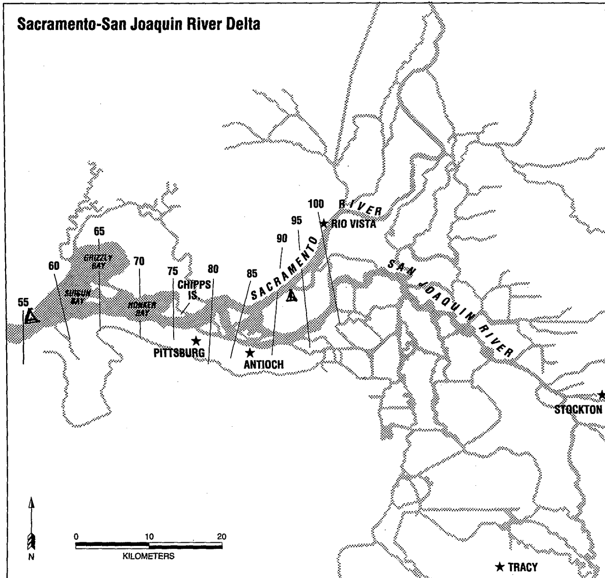
Figure 1. This map of the upper estuary displays sites of the continuous monitoring stations (triangles) within the study area, and indicates hypothetical positions of a 2ppt isohaline measured at 5 kilometer increments upstream from the Golden Gate Bridge.
