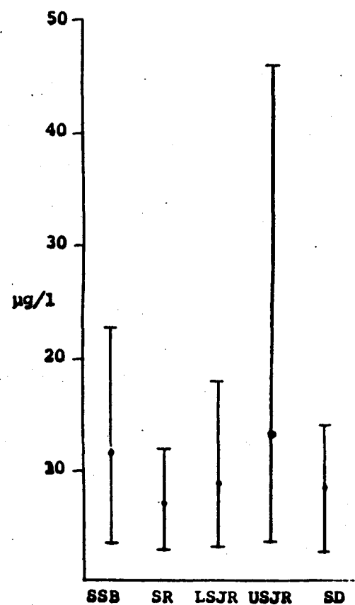
Fig. 3 . March-November means and ranges of chlorophyll a by area, 1969-1985. Areas are SSB - Suisun Bay, SR - Sacramento River, LSJR - lower San Joaquin River, USJR - upper San Joaquin River, SD - south delta.
