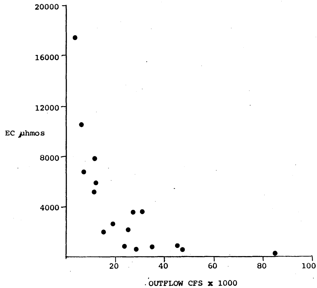
Fig. 10. Relationship between delta outflow as measured at Chipps Island from Dayflow Model and Chipps Island EC. The points are March to November means for 1969-1985.
