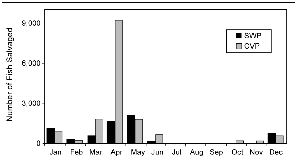
Figure 3-16. Monthly Salmon salvage at SWP and CVP, 2002 (Foss 2003).
