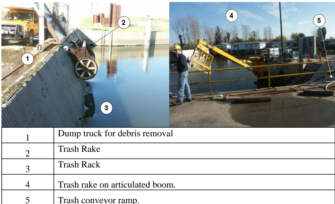
Figure 2-21 Trashrack
