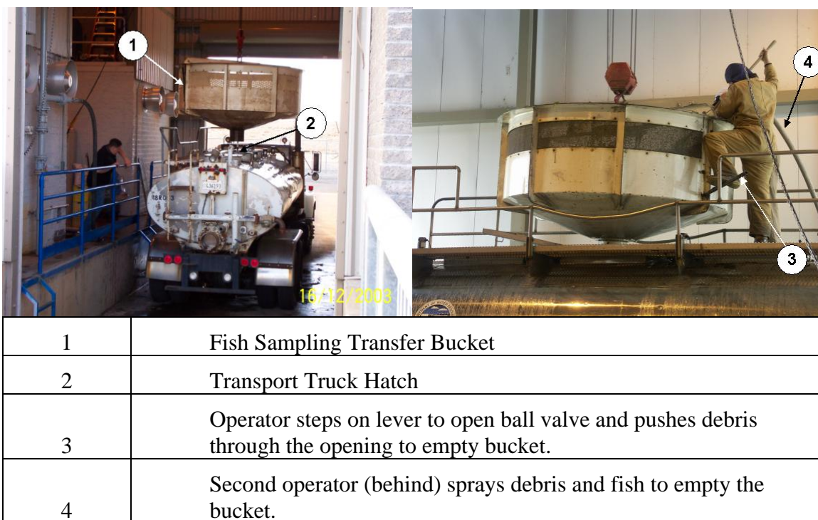
Figure 2-14 Fish are Transferred to Truck
