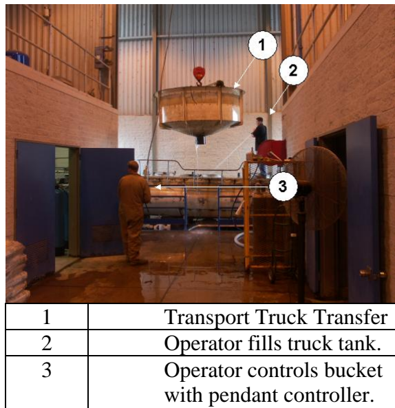
Figure 2-13 Transport Truck Bucket
