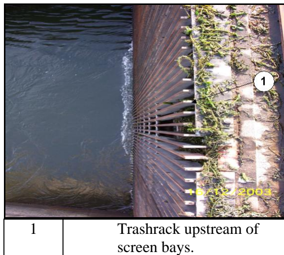
Figure 2-5 Trashrack
