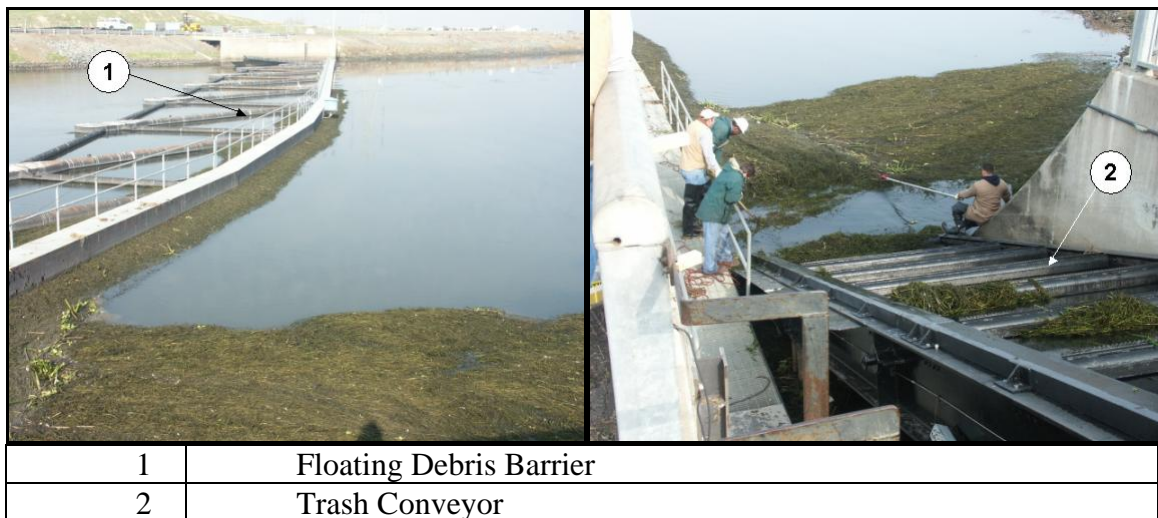
Figure 2-3 SWP Trash Boom and Conveyor
