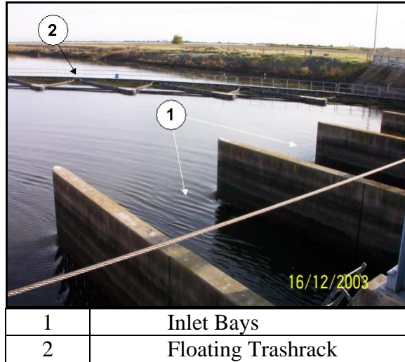
Figure 2-4 Inlet Bays
