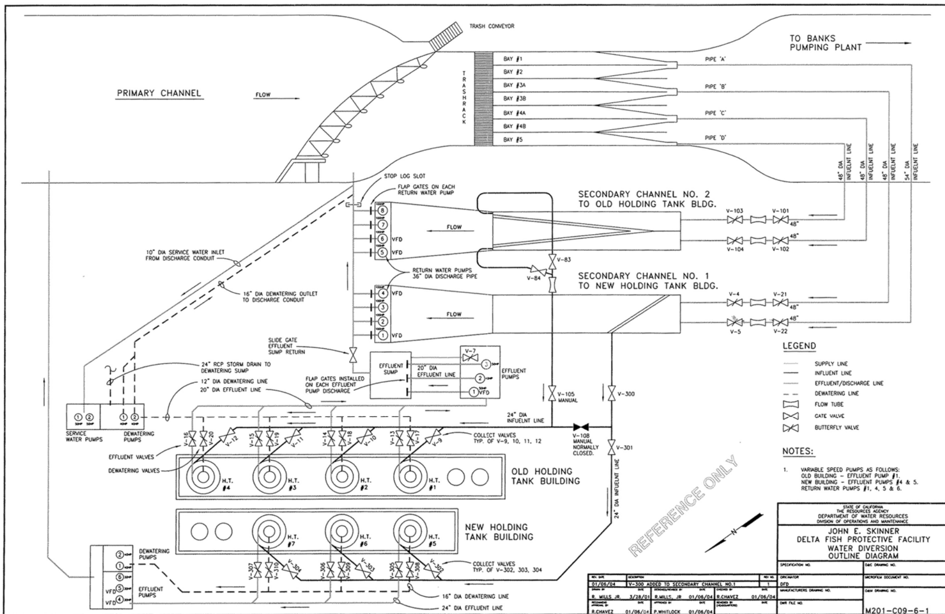
Figure 2-2 Skinner Fish Protection Facility Layout
