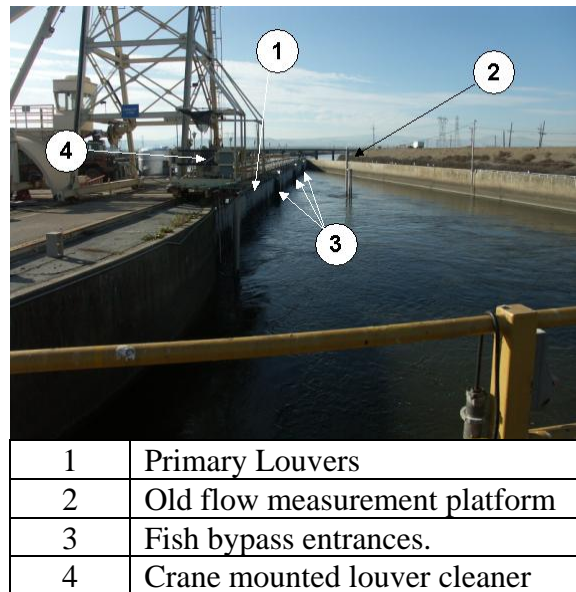
Figure 2-22 Primary Louvers
