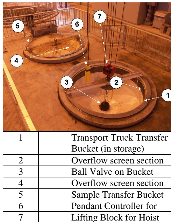
Figure 2-10 Fish Transfer Buckets
