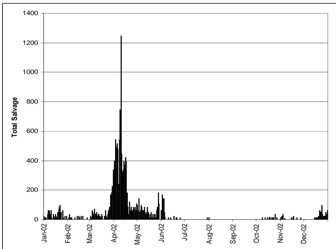
Figure 3-7. Seasonal distribution of Chinook salmon at CVP, 2002.
