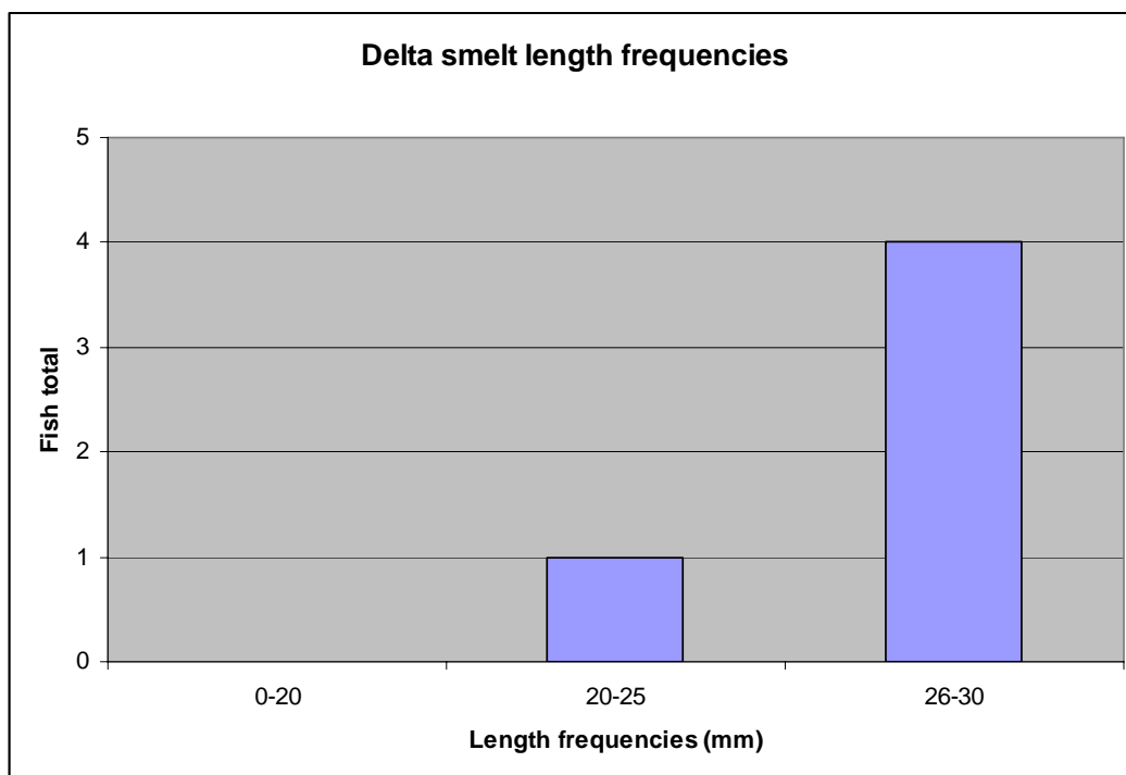
Figure 3-19. Length class frequencies for delta smelt caught in 10 minute count at CVP, 04:00 hrs 5/21/02.
