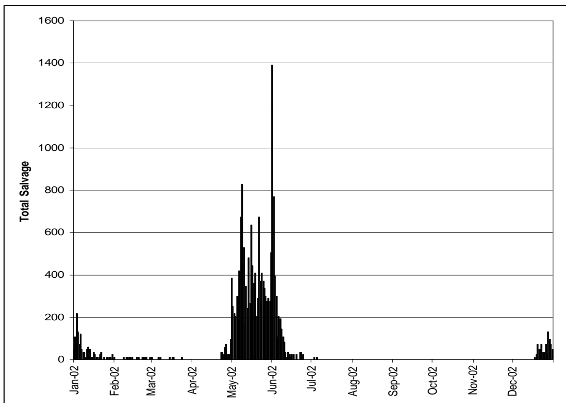
Figure 3-5. Seasonal distribution of delta smelt at CVP, 2002.
