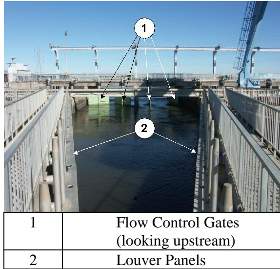
Figure 2-6 Flow Control Gates
