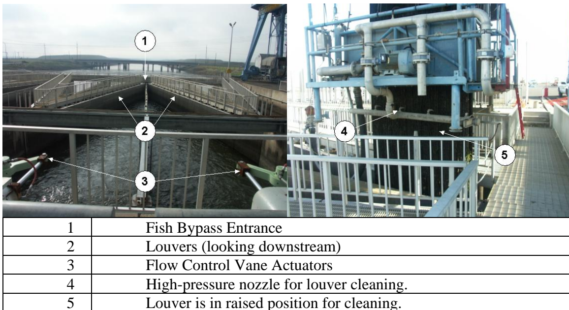
Figure 2-7 Louvers
