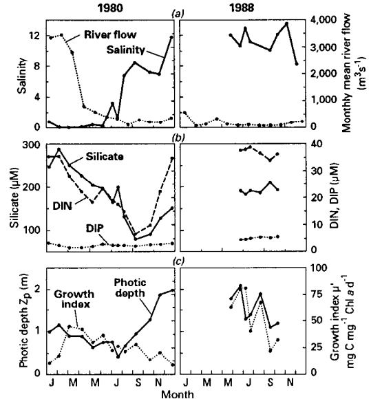
Fig. 6. Seasonal changes in selected physical-chemical measurements in Suisun Bay (USGS station 5), comparing 1980 and 1988. [a.] Monthly mean river flow and near-surface salinity. [b.] Near-surface concentrations of dissolved silicate, inorganic N ( \text{NO}_2^- + \text{NO}_3^- + \text{NH}_4^+ ) (DIN), and reactive P (DIP). [c.] Photic depth Z_p and the index of phytoplankton population growth rate \mu' . Nutrient data are from Ota et al. (1989) and S. W. Hager (unpubl. data).
