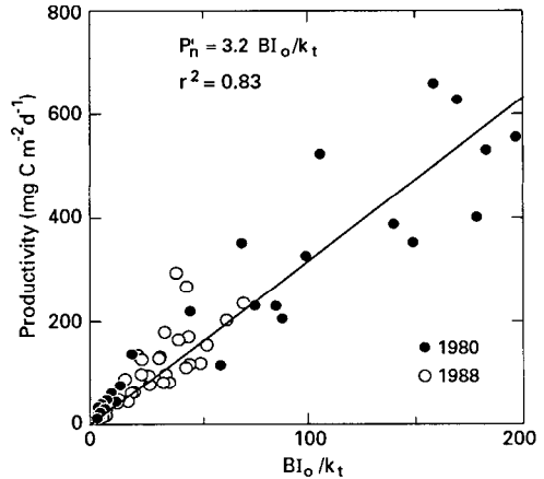
Fig. 7. Measured daily primary productivity vs. the composite parameter BI_0/k_t (1980 data from Cole and Cloern 1984). B is the phytoplankton biomass as Chl a concentration, I_0 is incident solar radiation ( \text{Einst m}^{-2} \text{ d}^{-1} ), and k_t is extinction coefficient ( \text{m}^{-1} ).
