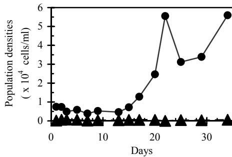
Figure 1. Competition between M. novacekii and S. quadricauda at 0.1 d -1 of dilution rate and 10 \mu M of ammonium
