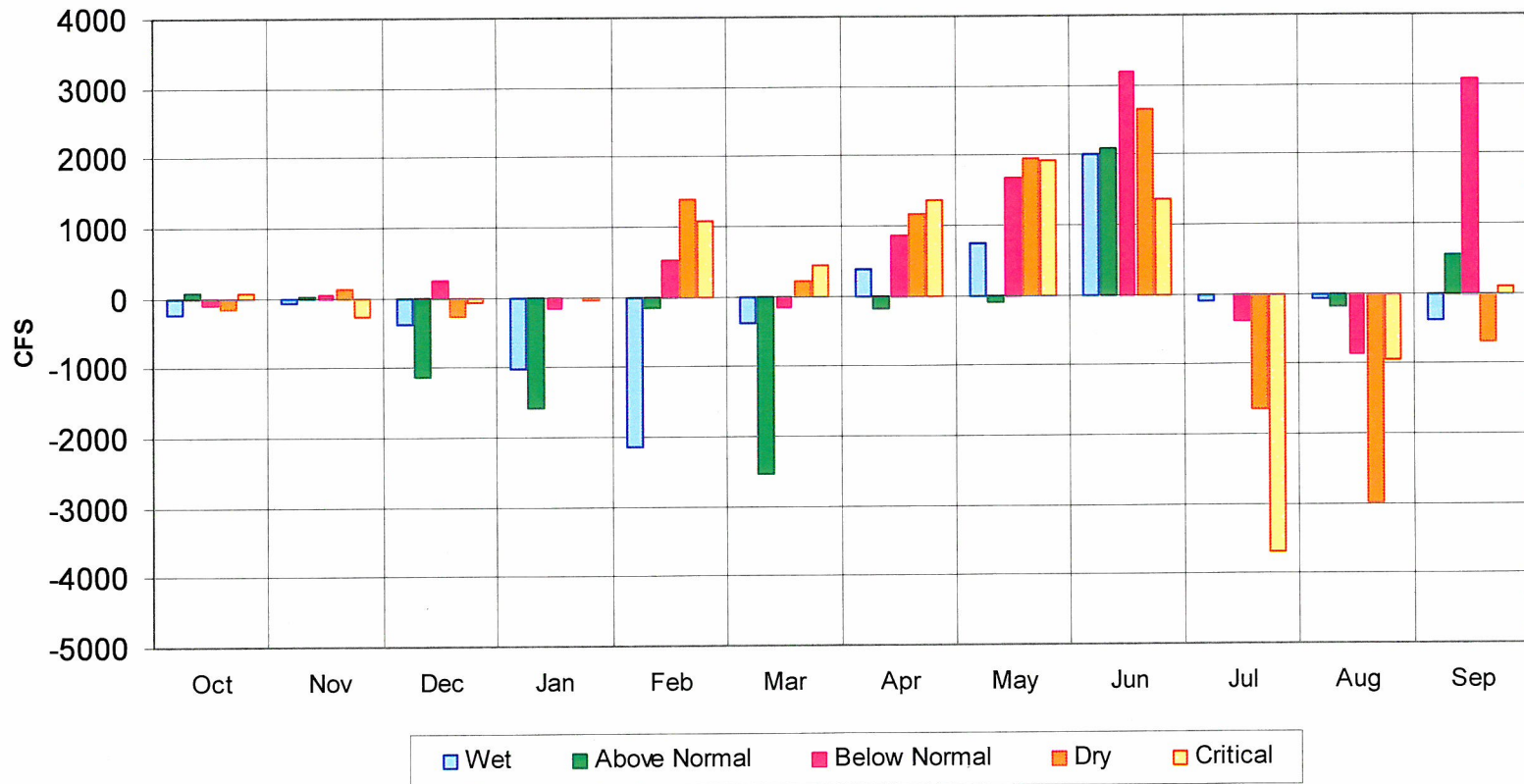
EXHIBIT SVWU-29 FEATHER RIVER BELOW THERMALITO AFTERBAY DIFFERENCE BETWEEN AND BAY INSTITUTE AND BIOLOGICAL OPINION'S AVERAGE MONTHLY DIFFERENCE BY WATER-YEAR TYPE FOR 1922-2003
