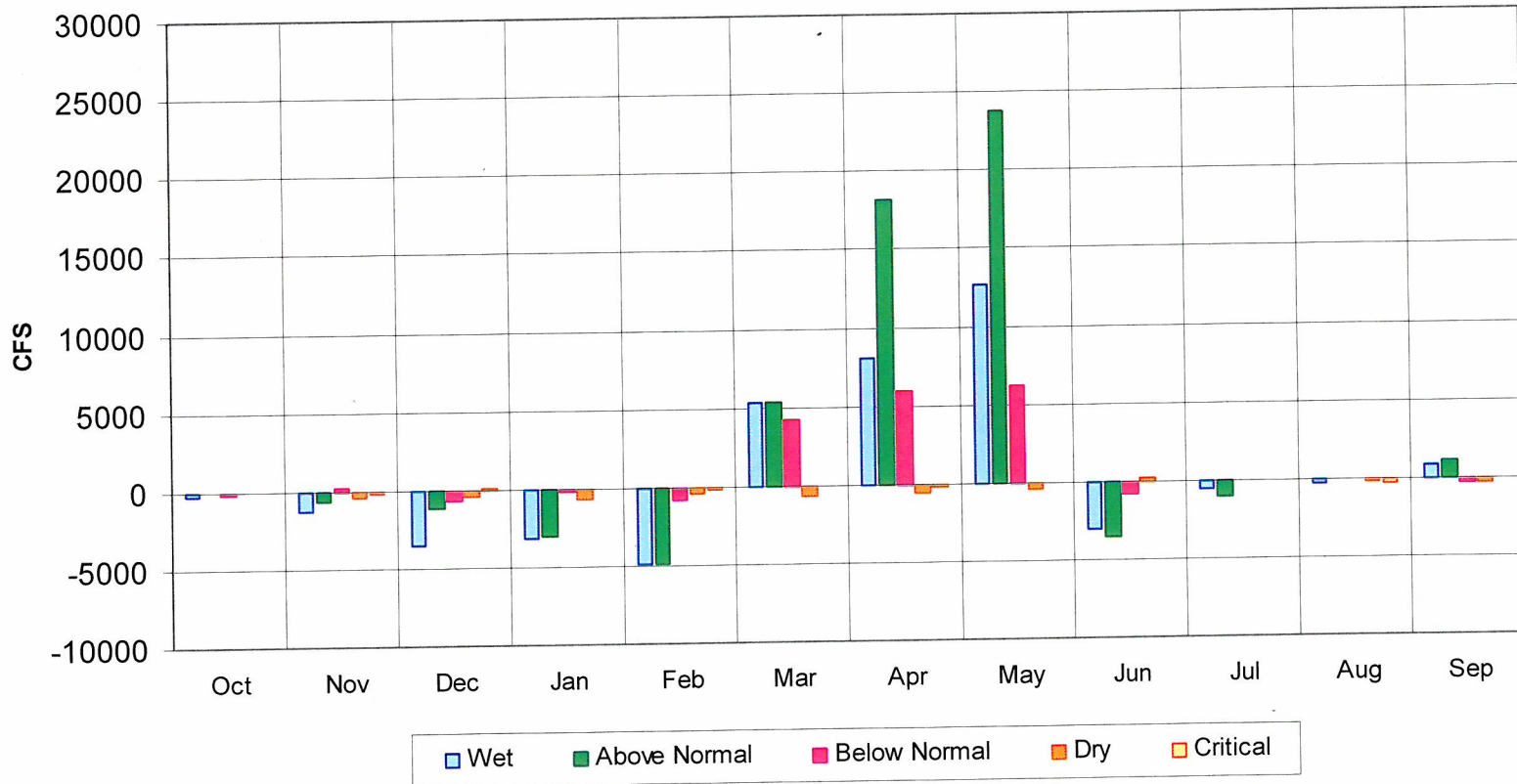
EXHIBIT SVWU- 32 DELTA OUTFLOW DIFFERENCE BETWEEN UCD1 (DELTA OUTFLOW TARGET) AND BIOLOGICAL OPINION'S AVERAGE MONTHLY DIFFERENCE BY WATER-YEAR TYPE FOR 1922-2003
