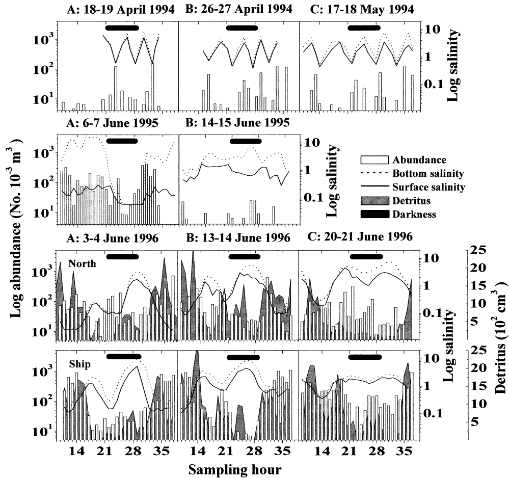
Fig. 3. Total fish abundance ( \text{No.} \times 10^{-3} \text{ m}^3 ) with surface and bottom salinity during each cruise 1994–1996. Also shown in 1996 are the volumes of detrital material in samples.
