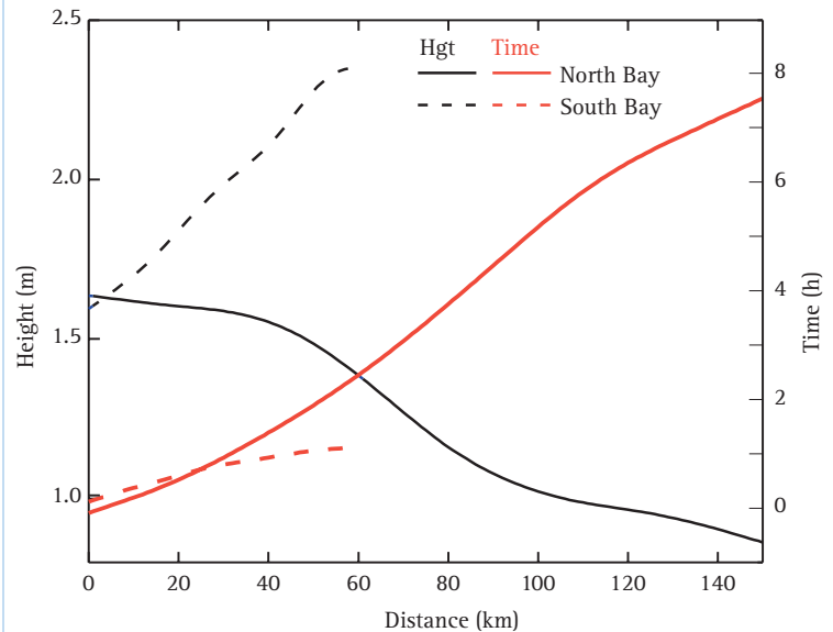
Figure 10. Timing and height of high tide as a function of location, expressed as distance along the channels from the Golden Gate north and east into the Delta (solid lines), or south through South Bay (dashed lines). Black lines, height of high tide. Red lines, lag in hours of high tide after the high tide at the Golden Gate. Lines are generalized additive models with smoothing function, fit to published timing of high tide by location.
