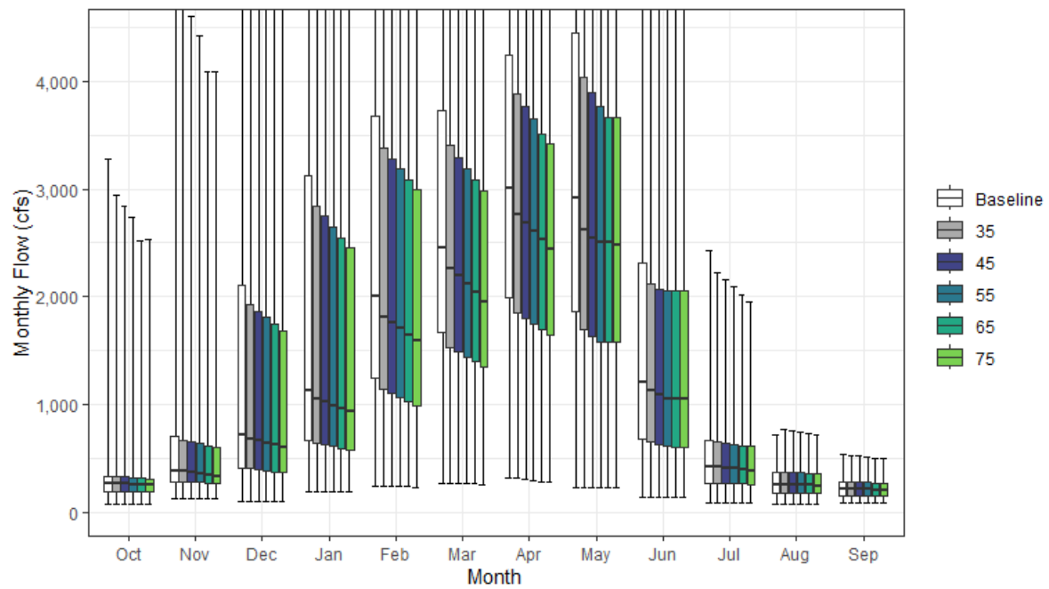
Figure A1-43. Yuba River, North Fork Streamflow above New Bullards Bar Reservoir Monthly Boxplot
