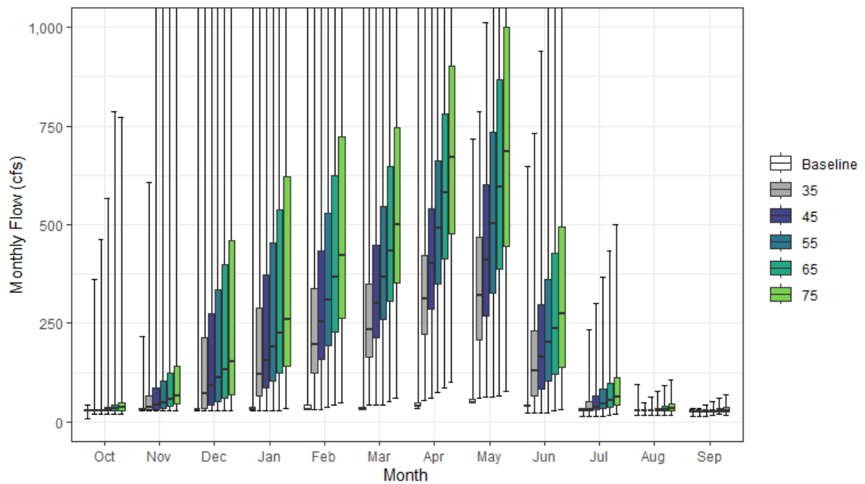
Figure A1-45a. Yuba River, Middle Fork above Confluence with North Fork Yuba (SWRCB M Yuba Inflow) Monthly Flow (cfs) Boxplot
