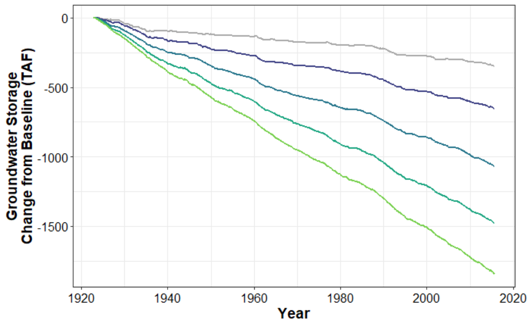
Figure A1-253. Eastern San Joaquin Groundwater Basin End-of-Year Storage – Change from Baseline (TAF)
