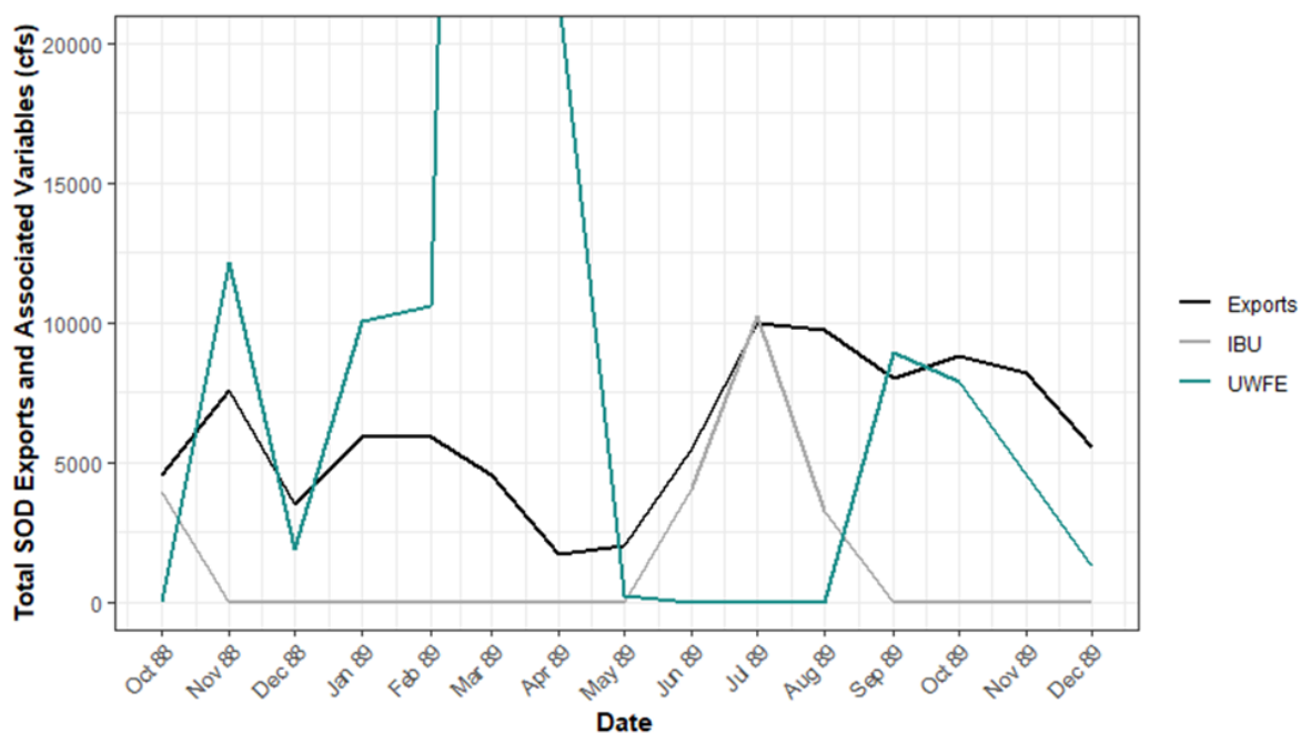
Figure A1-1. Total South-of-Delta (SOD) Exports, In-Basin Use (IBU), and Unstored Water for Export (UWFE) for water year 1989 and the following fall (dry year amid drought) for baseline
