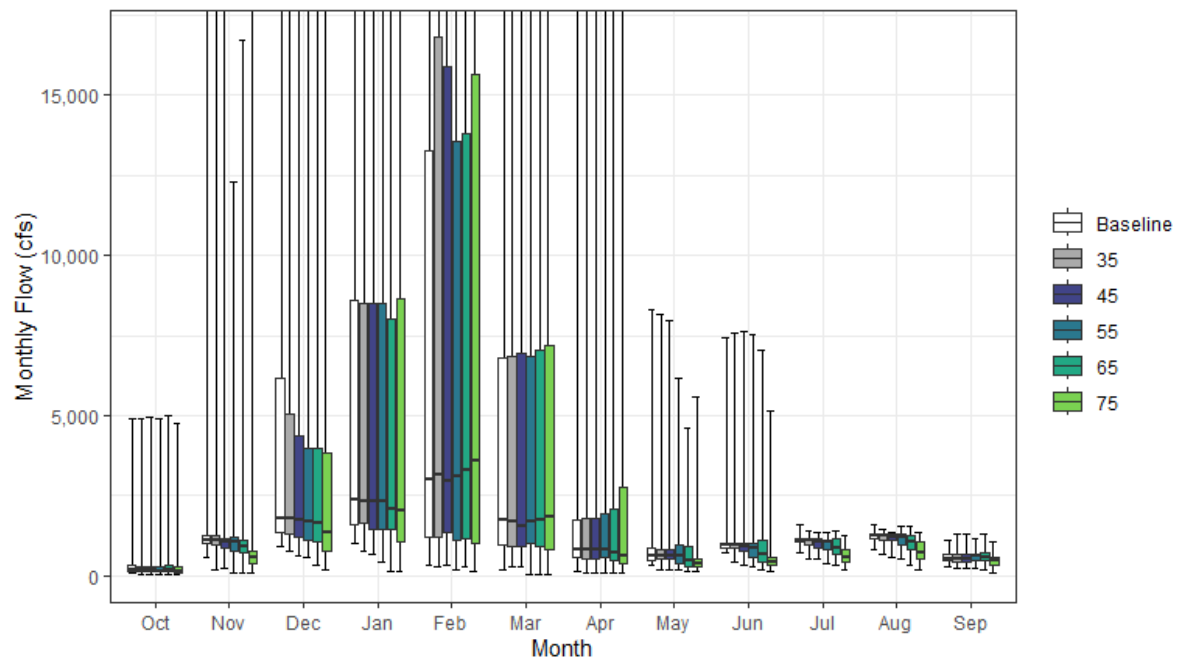
Figure A1-39. Sutter Bypass Streamflow Monthly Boxplot
