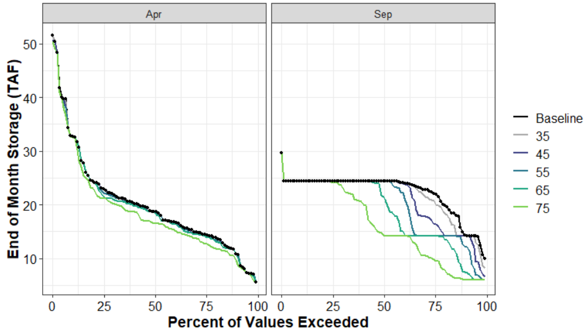
Figure A1-129. Lower Bear End-of-April and End-of-September Storage Percent Exceedance Plot
