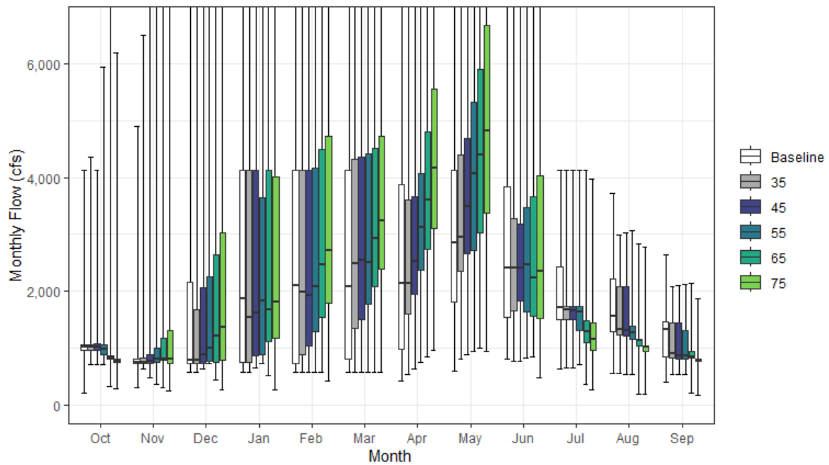
Figure A1-44. Yuba River Streamflow below Englebright Reservoir Monthly Boxplot
