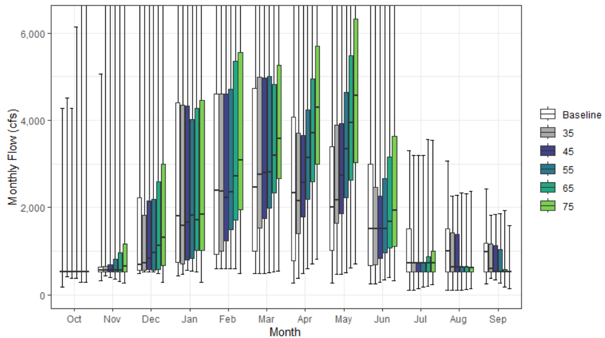
Figure A1-46. Yuba River Streamflow above Confluence with Feather River Monthly Boxplot
