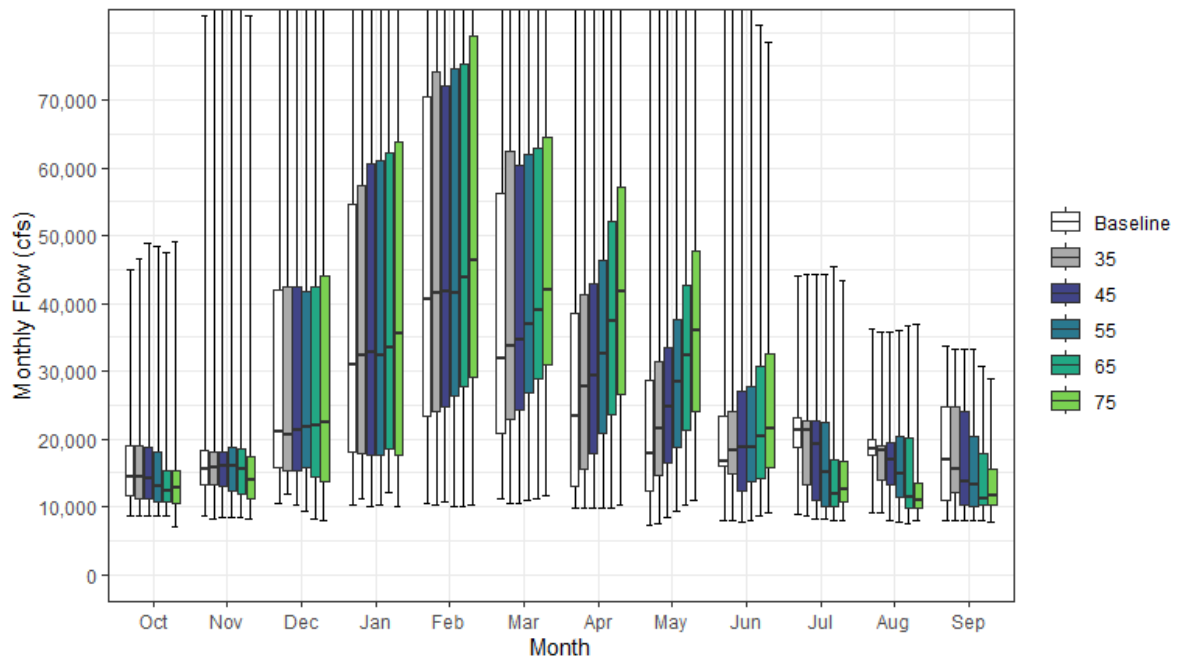
Figure A1-47. Total Delta Inflow Monthly Boxplot
