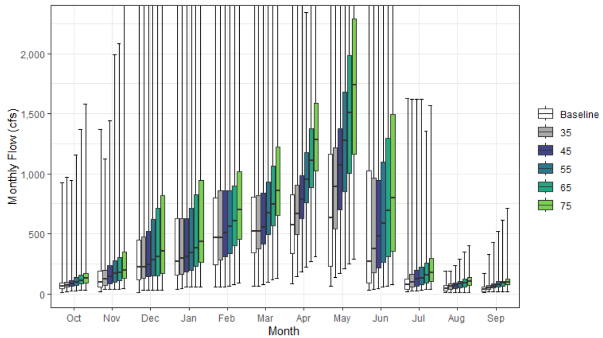
Figure A1-45. Yuba River, South Fork Streamflow above Englebright Reservoir Monthly Boxplot
