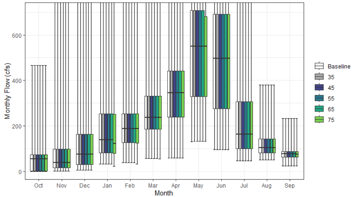
Figure A1-66. Robbs Peak Tunnel Monthly Boxplot
