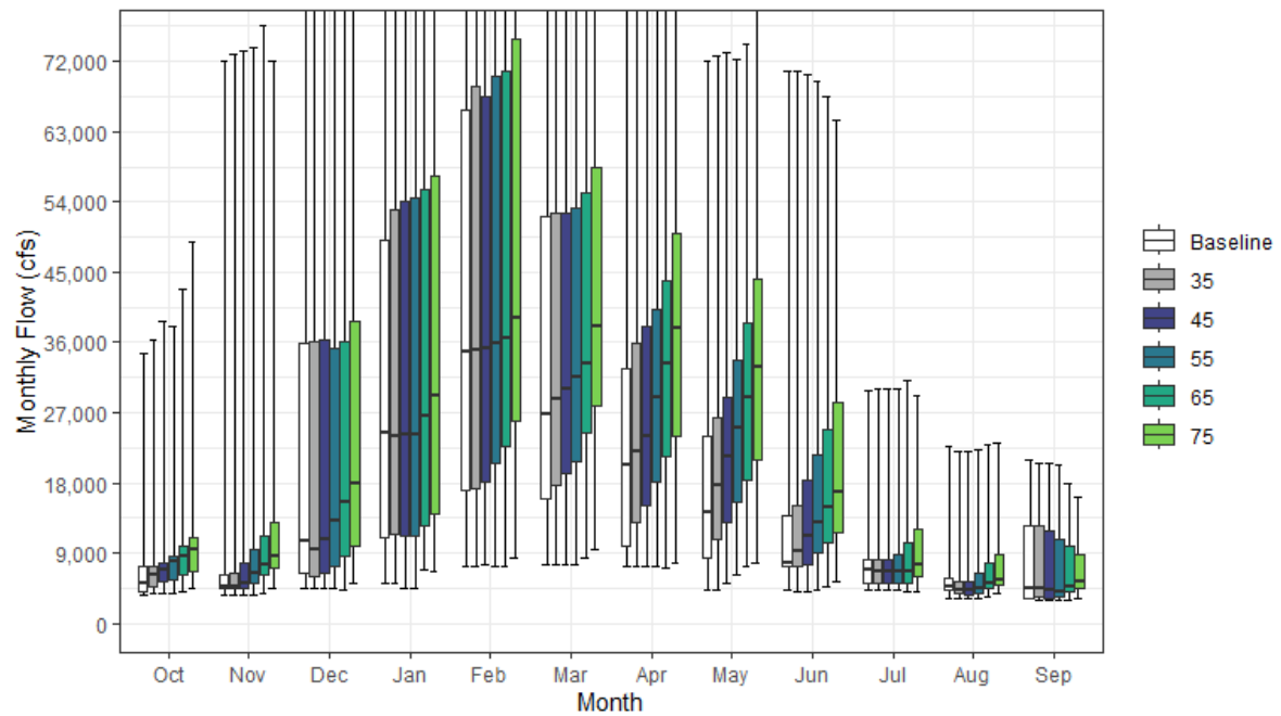
Figure A1-48. Delta Outflow Monthly Boxplot
