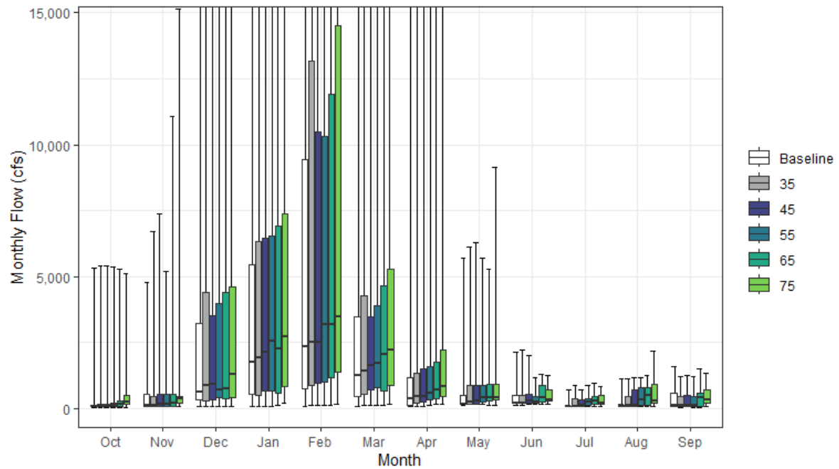
Figure A1-42. Yolo Bypass below Putah Creek Inflow Monthly Boxplot
