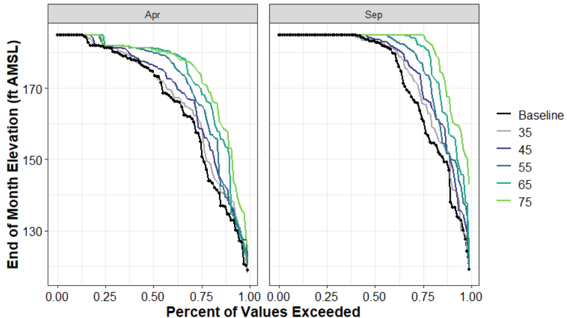
Figure A1-128. Los Vaqueros Reservoir End-of-April and End-of-September Elevation Percent Exceedance Plot
