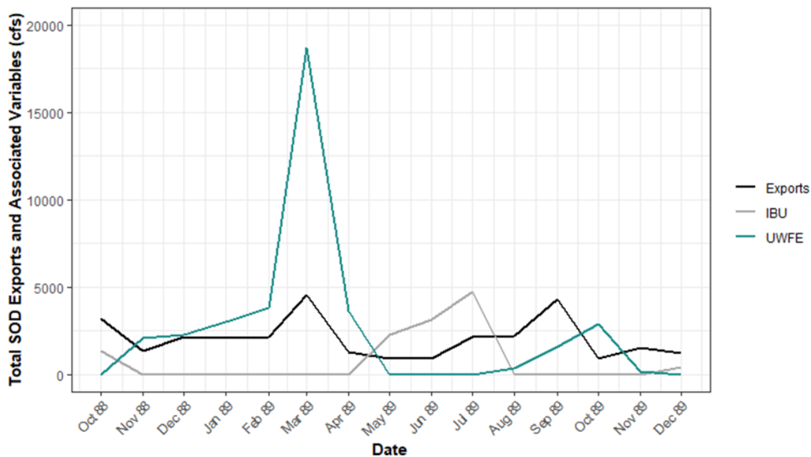
Figure A1-2. Total South-of-Delta (SOD) Exports, In-Basin Use (IBU), and Unstored Water for Export (UWFE) for Water Year 1989 and the following fall (dry year amid drought) for the 75 Scenario
