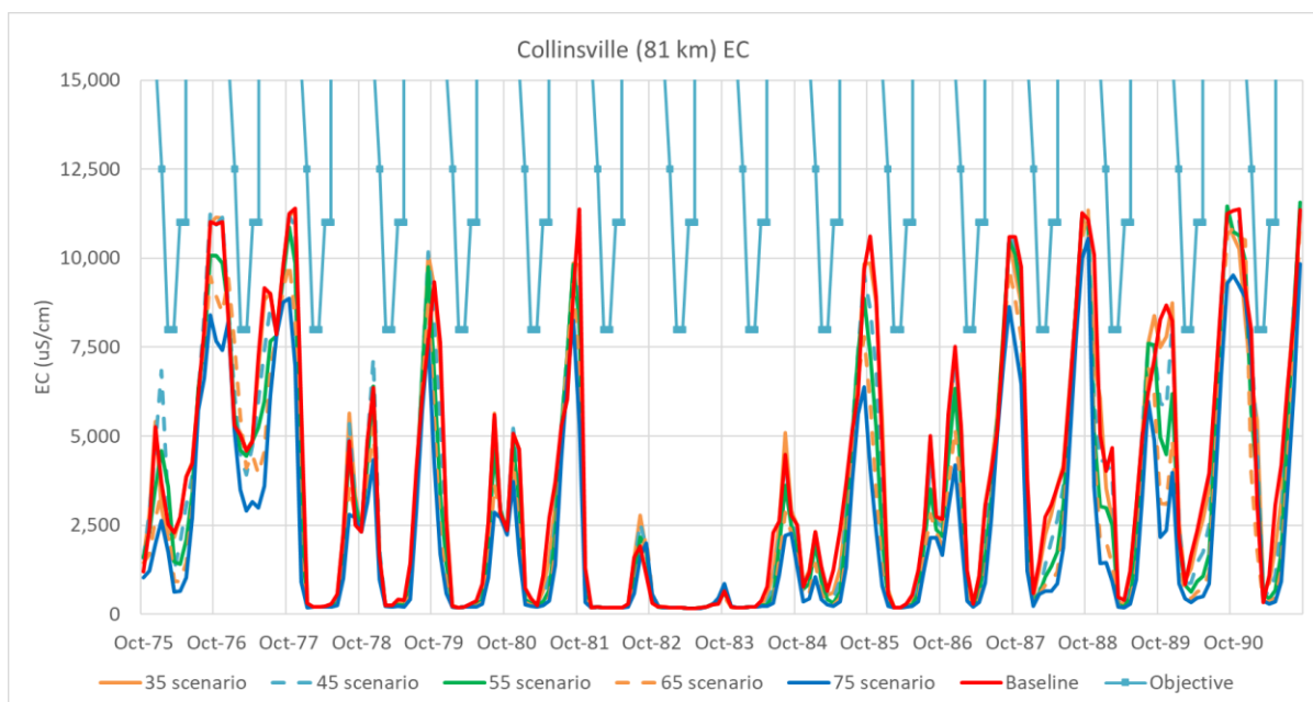
Figure A2-19. Time Series of DSM2 EC Values for Collinsville – Baseline and Flow Scenarios for WY 1976–1991 with EC Objectives for Reference
