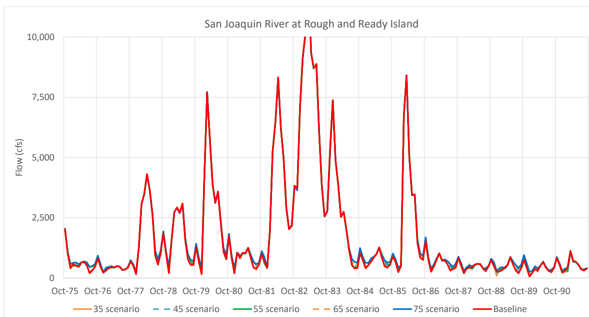
Figure A2-14. DSM2 Flow in the San Joaquin River near Stockton – Baseline and Flow Scenarios for WY 1976–1991
