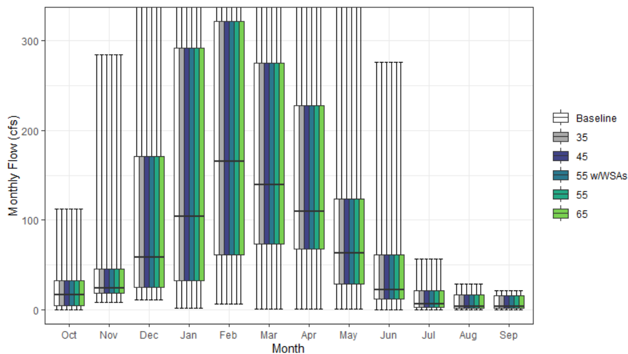
Figure H1a3-18. Elder Creek Streamflow above Confluence with Sacramento River Monthly Boxplot (cfs)
