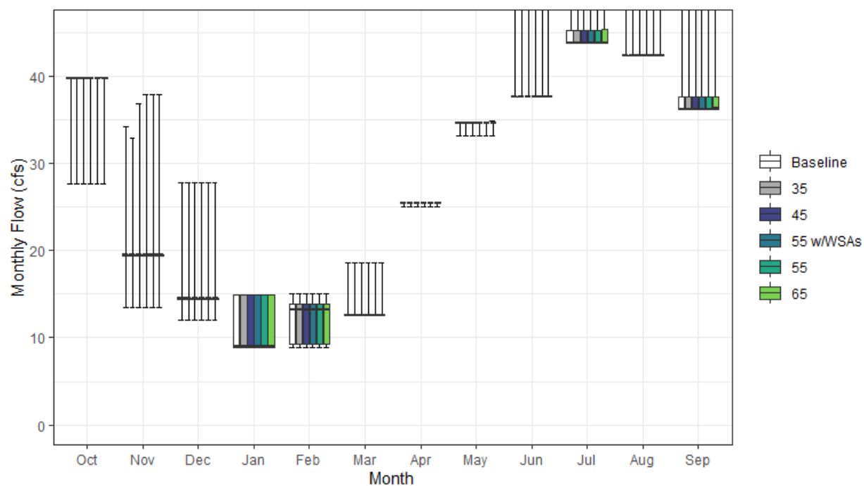
Figure H1a3-56. Jenkinson Lake Camino Conduit Monthly Boxplot (cfs)
