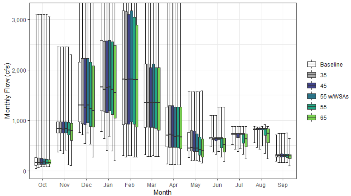
Figure H1a3-8. Butte Creek Streamflow above Butte Slough Monthly Boxplot (cfs)
