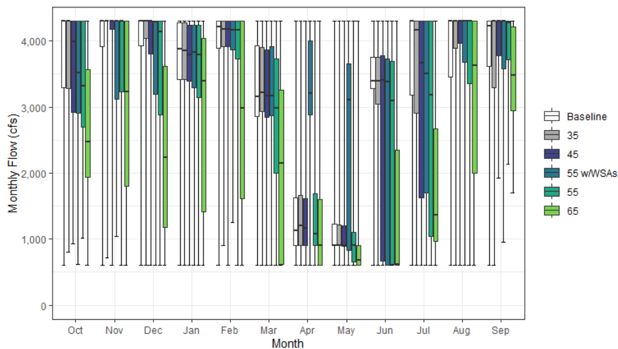
Figure H1a3-51. Jones Pumping Plant (CVP) Monthly Boxplot (cfs)
