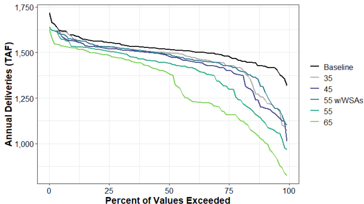
Figure H1a3-168. Total Water Supplied to Water Budget Area 8 (Agricultural) Annual Percent Exceedance Plot.
