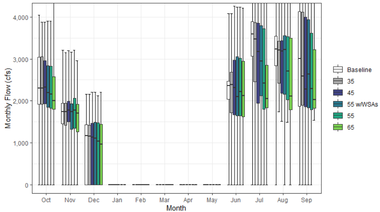
Figure H1a3-47. Delta Cross Channel Monthly Boxplot (cfs)
