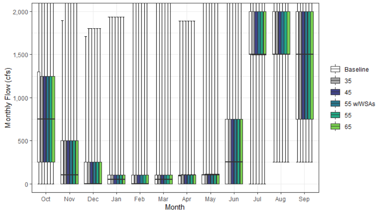
Figure H1a3-63. Clear Creek Tunnel Monthly Boxplot (cfs)
