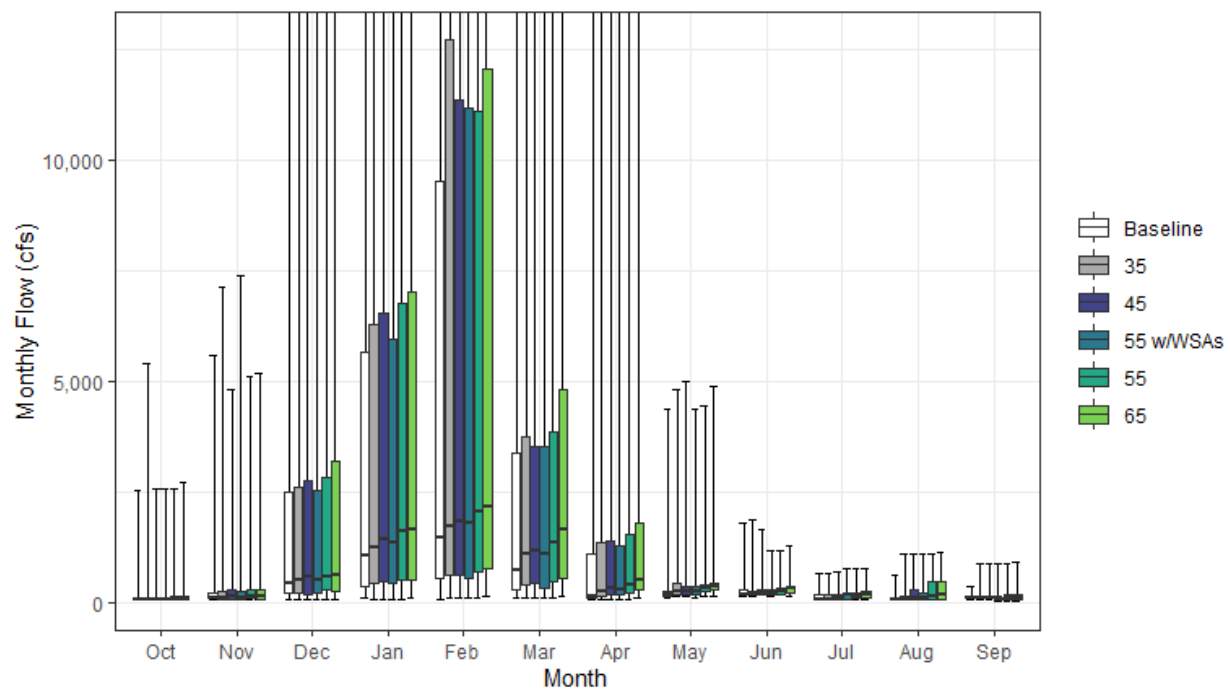
Figure H1a3-39. Yolo Bypass Streamflow below Putah Creek Inflow Monthly Boxplot (cfs)
