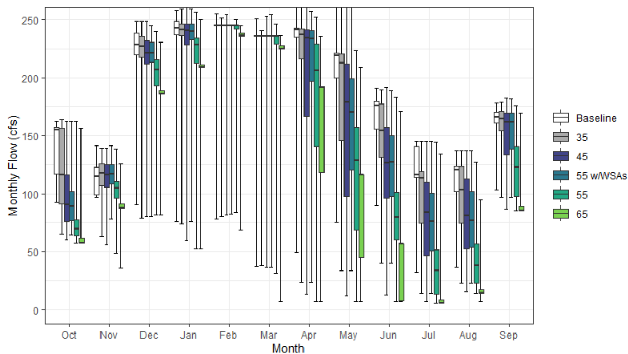
Figure H1a3-60. South Canal Monthly Boxplot (cfs)
