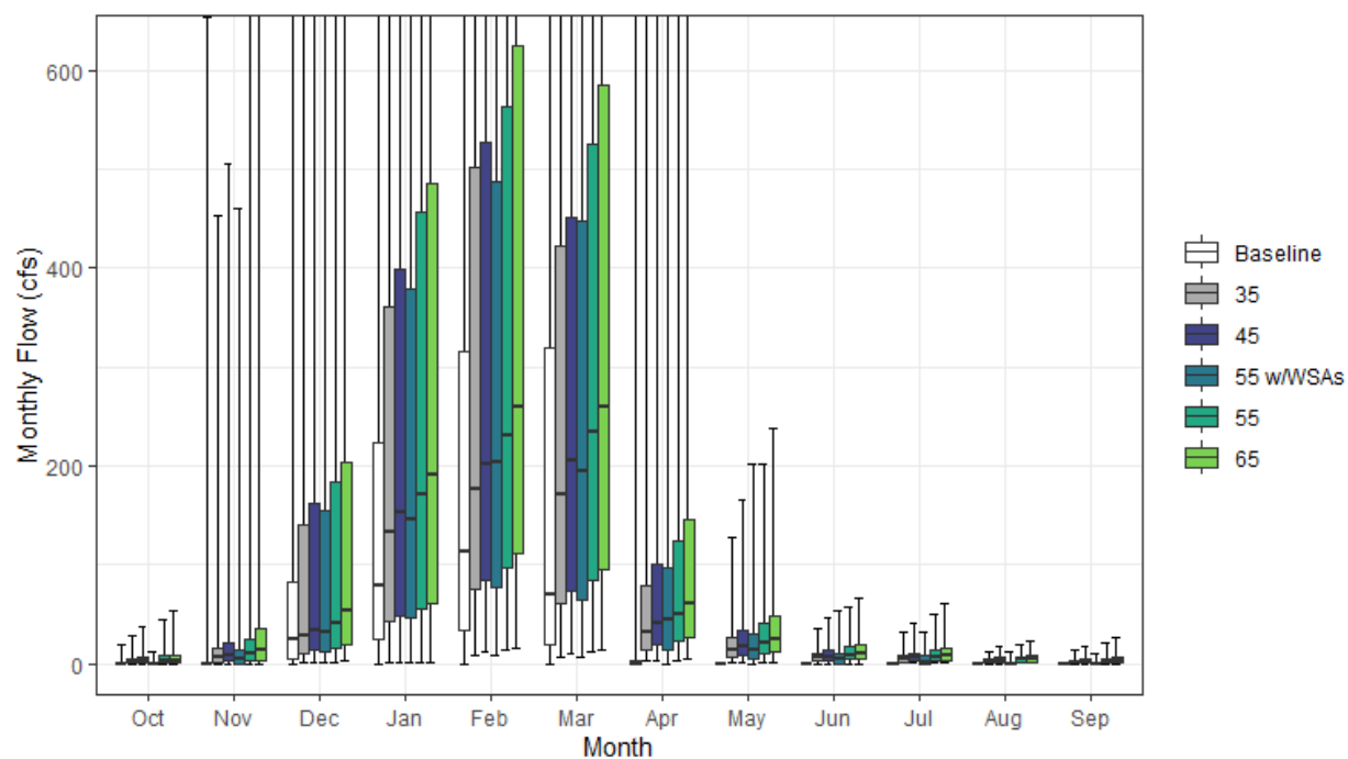
Figure H1a3-12. Calaveras River Streamflow above Delta Monthly Boxplot (cfs)
