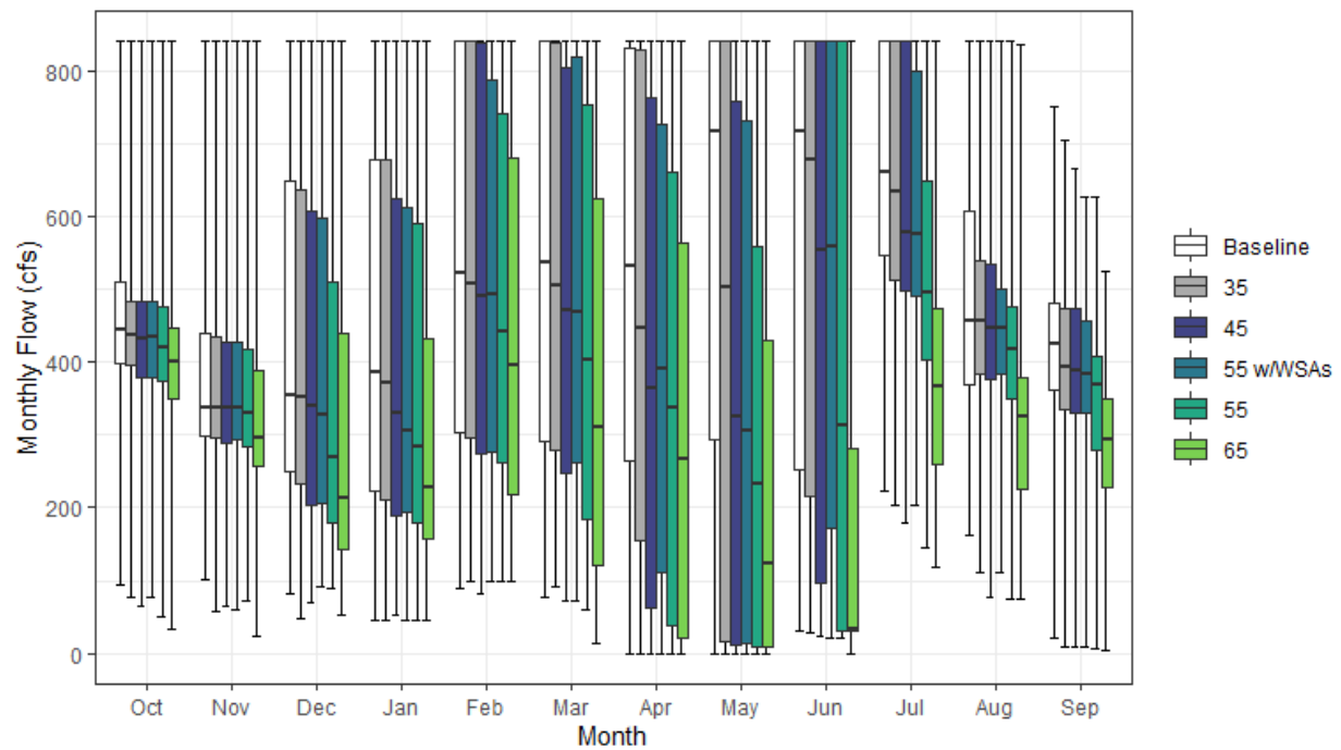
Figure H1a3-54. Drum Canal Monthly Boxplot (cfs)
