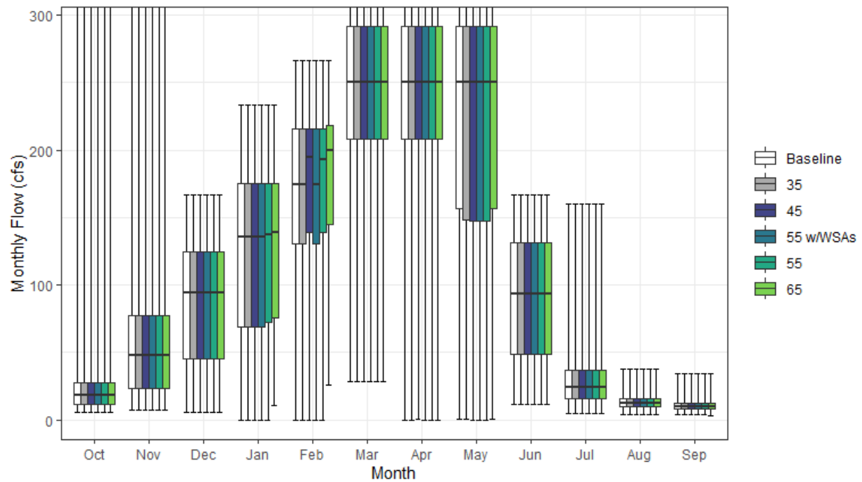
Figure H1a3-59. Slate Creek Tunnel Monthly Boxplot (cfs)
