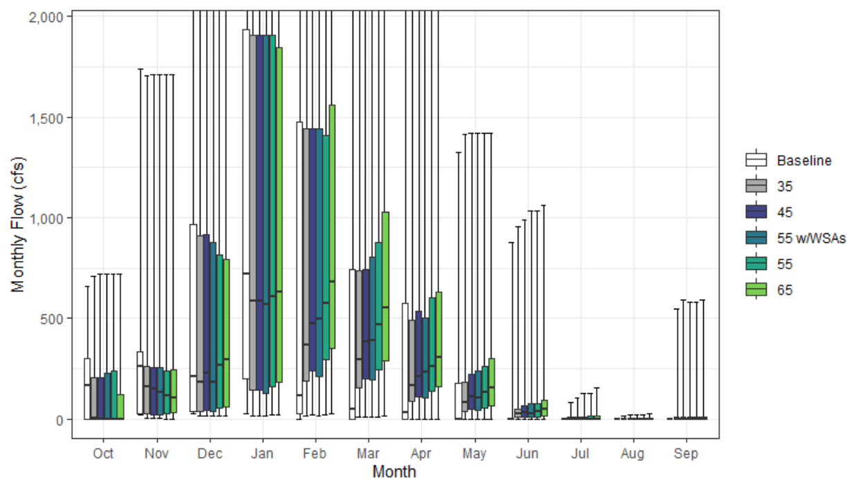
Figure H1a3-35. Stony Creek Streamflow above Confluence with Sacramento River Monthly Boxplot (cfs)
