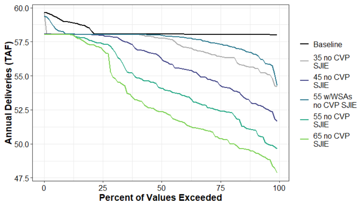
Figure H1a4-187. Total Water Supplied to Water Budget Areas 20 and 25 (Urban) Annual Percent Exceedance Plot.
