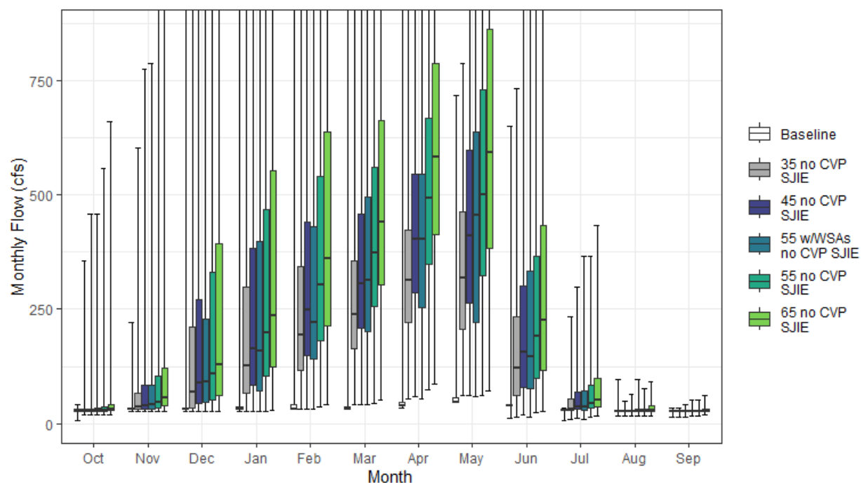
Figure H1a4-41. Yuba River, Middle Fork Streamflow above Confluence with North Fork Yuba Monthly Boxplot (cfs)
