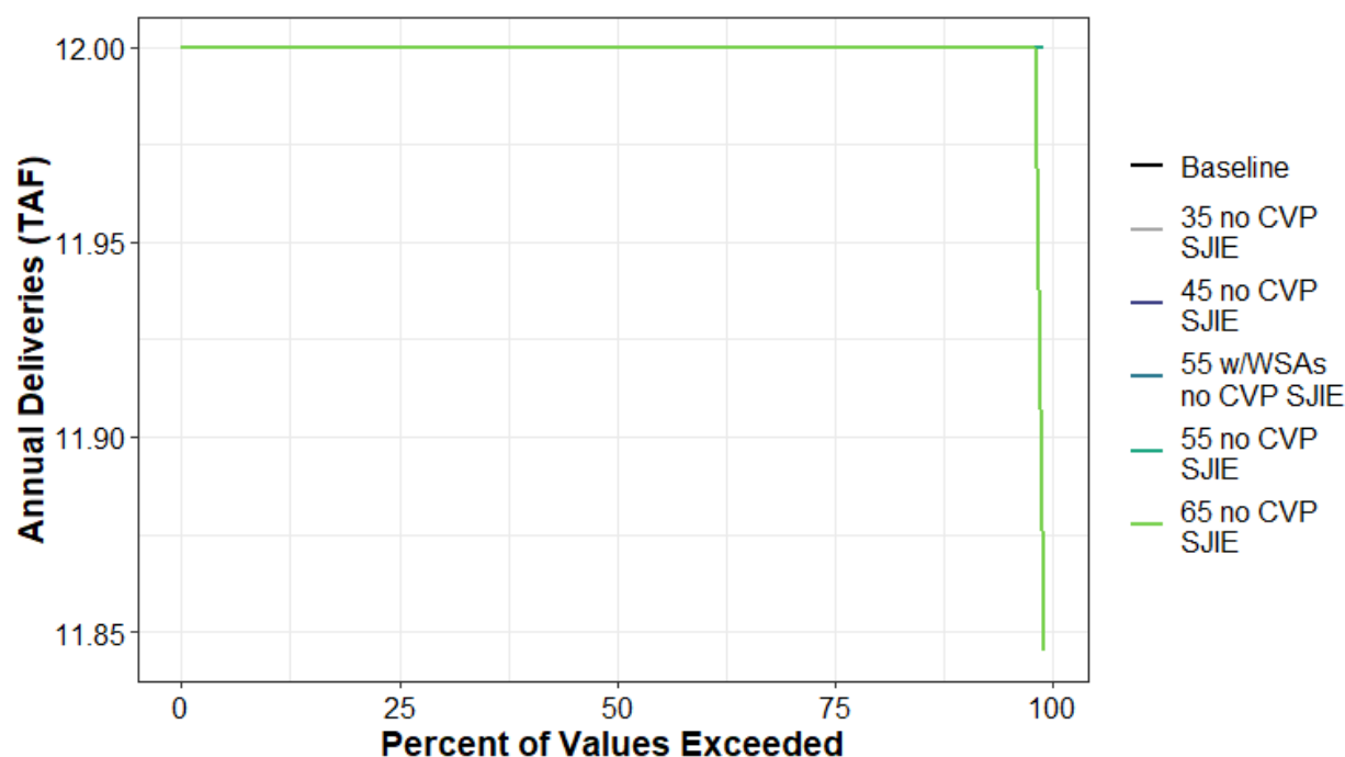
Figure H1a4-175. Total Water Supplied to Water Budget Area 11 (Urban) Annual Percent Exceedance Plot.
