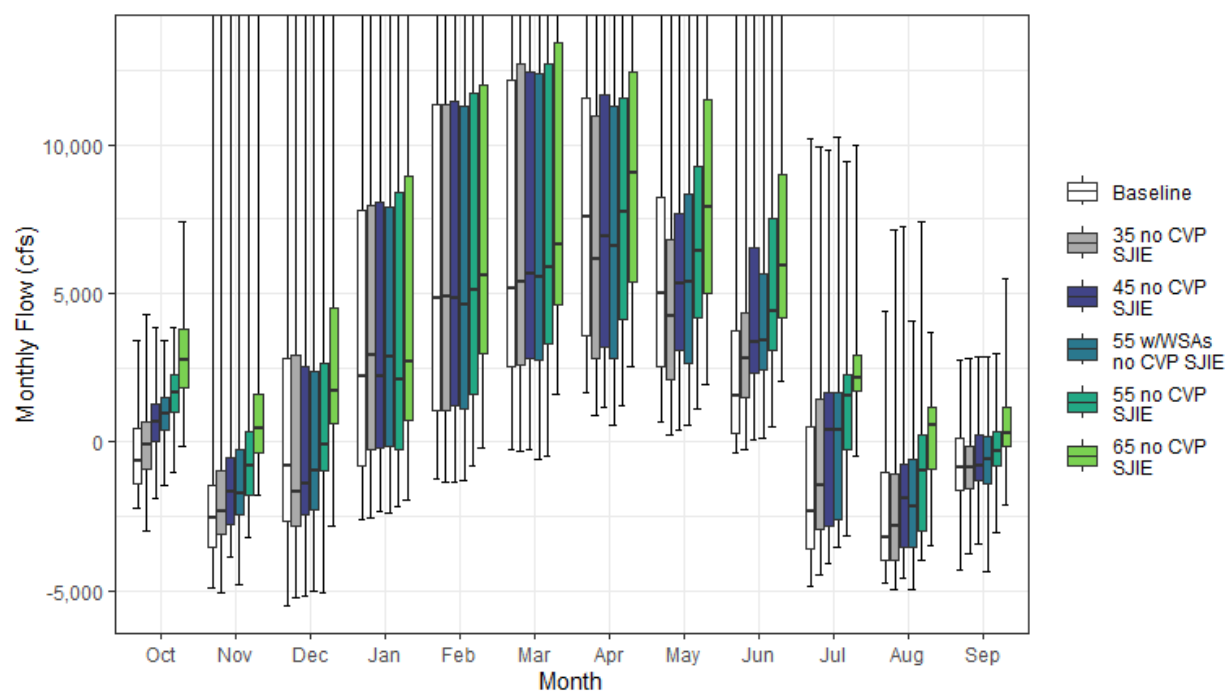
Figure H1a4-49. San Joaquin River at Jersey Point (QWEST) Monthly Boxplot (cfs)
