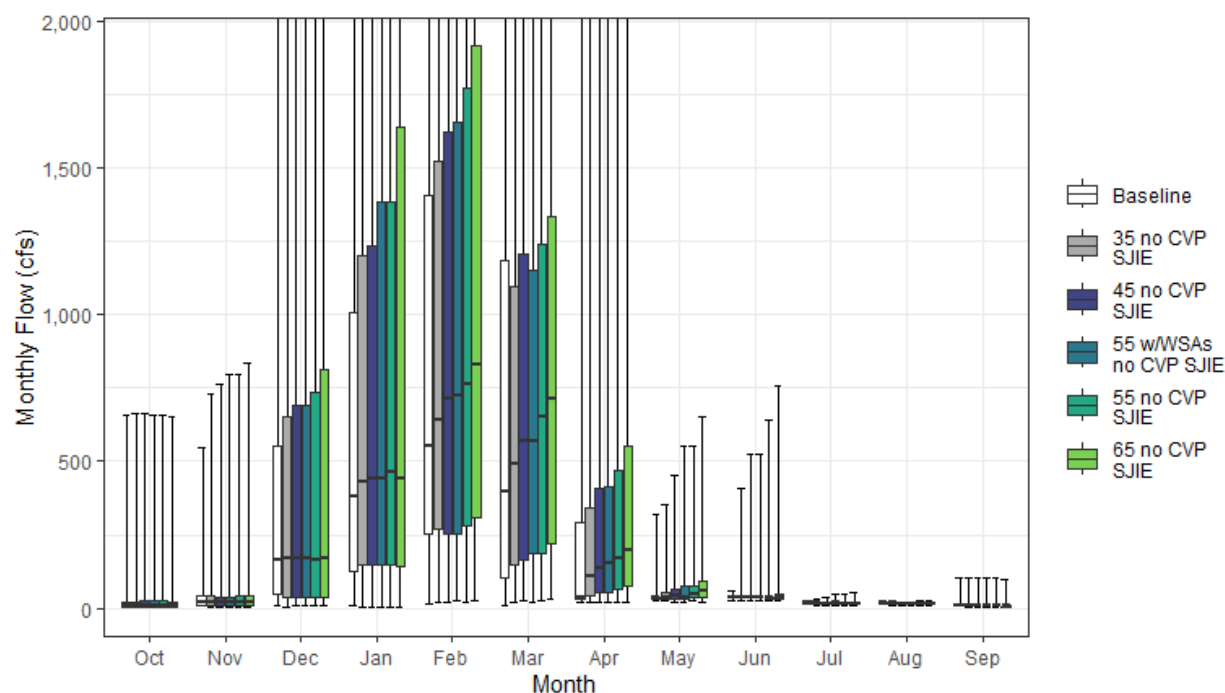
Figure H1a4-10. Cache Creek Streamflow above Yolo Bypass Monthly Boxplot (cfs)
