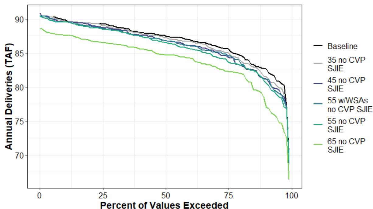
Figure H1a4-204. Surface Water Supplied to Upper Watershed and Foothill (Urban) Annual Percent Exceedance Plot.
