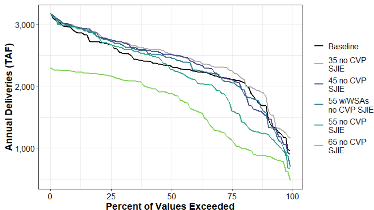
Figure H1a4-214. Surface Water Supplied to Total CVP South of Delta Annual Percent Exceedance Plot.
