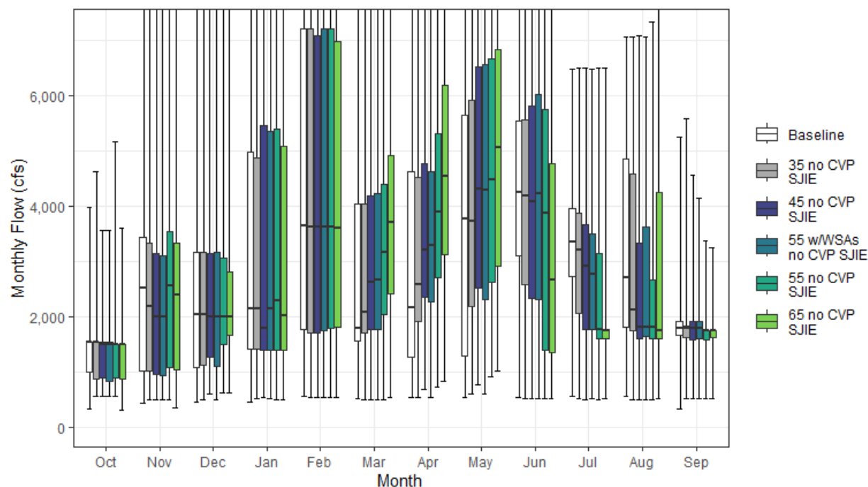
Figure H1a4-1. American River Streamflow below Folsom Reservoir Monthly Boxplot (cfs)
