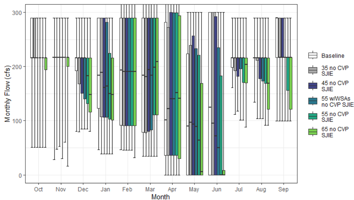
Figure H1a4-53. Bowman-Spaulding Conduit Monthly Boxplot (cfs)
