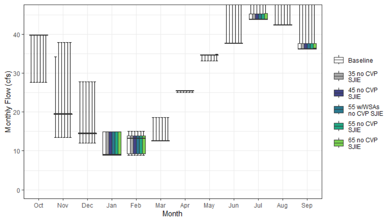
Figure H1a4-56. Jenkinson Lake Camino Conduit Monthly Boxplot (cfs)
