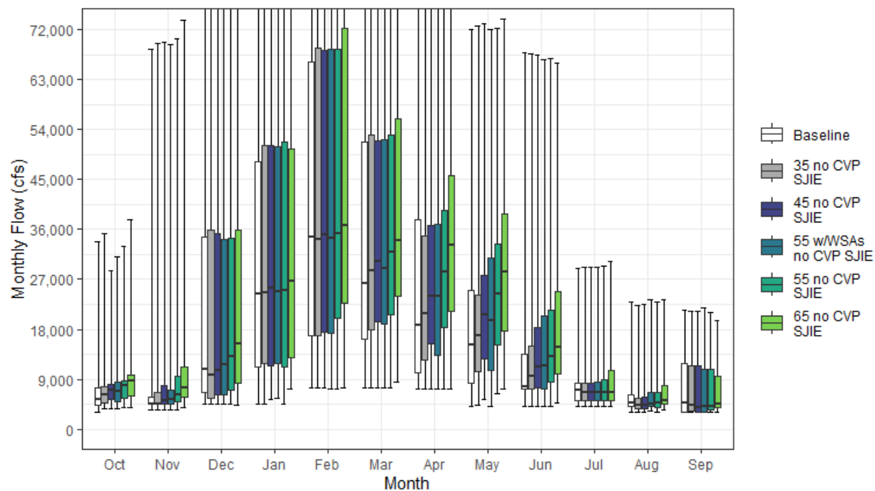
Figure H1a4-46. Delta Outflow Monthly Boxplot (cfs)
