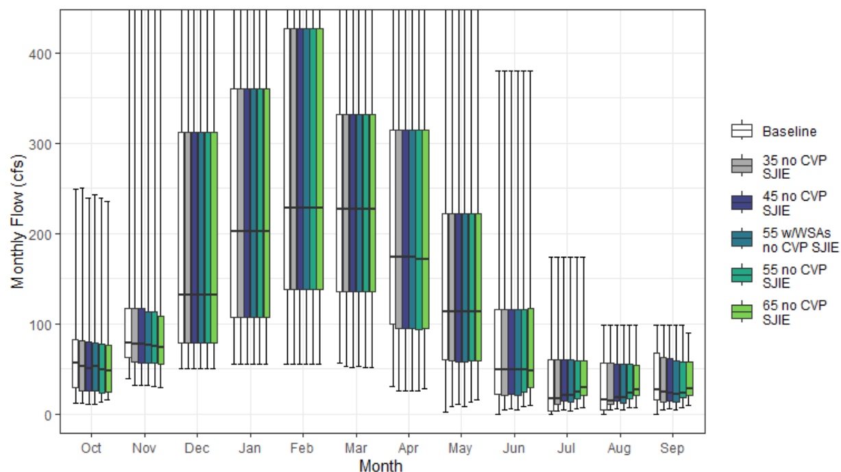
Figure H1a4-3. Antelope Creek Streamflow above Confluence with Sacramento River Monthly Boxplot (cfs)
