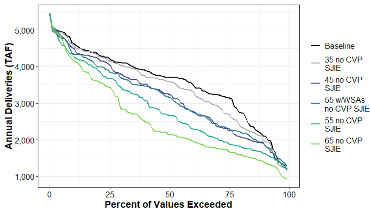
Figure H1a4-219. Surface Water Supplied to Total SWP Deliveries Annual Percent Exceedance Plot.
