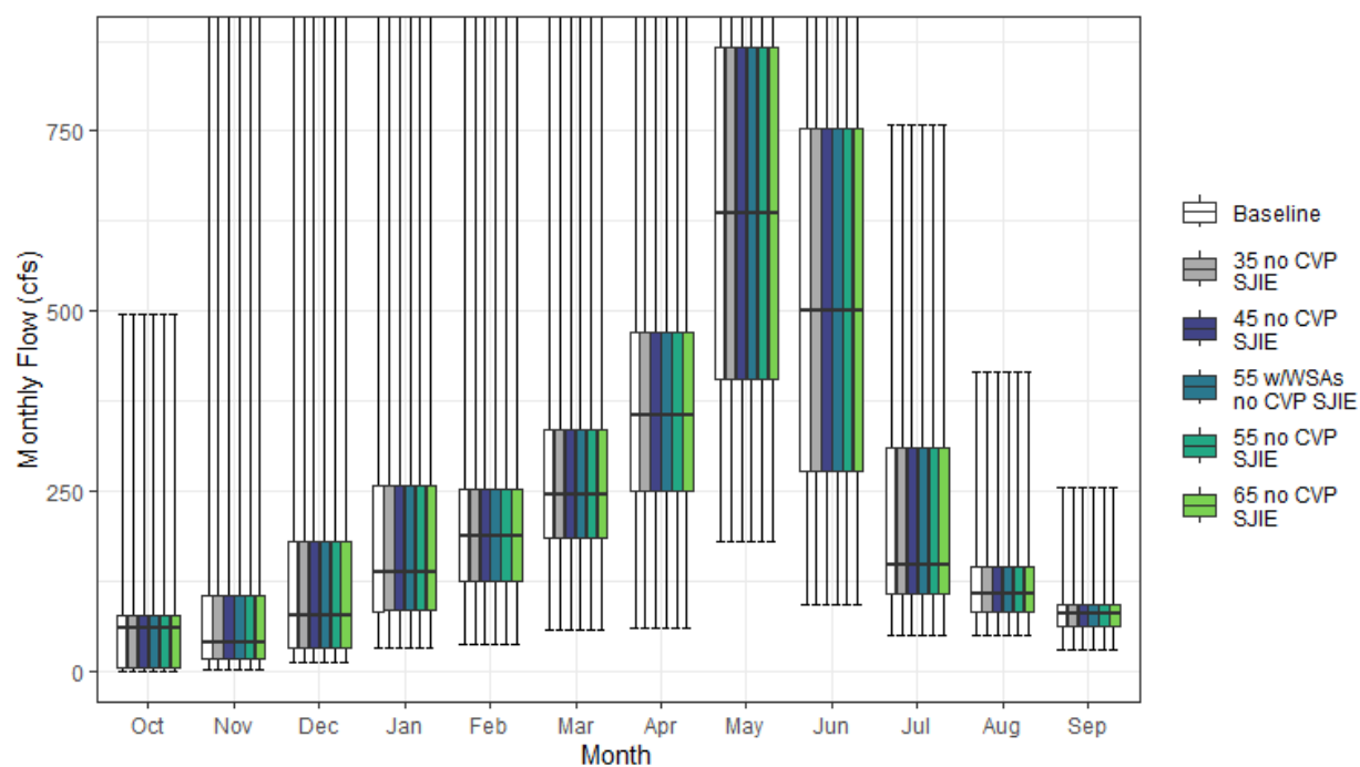
Figure H1a4-65. Robbs Peak Tunnel Monthly Boxplot (cfs)
