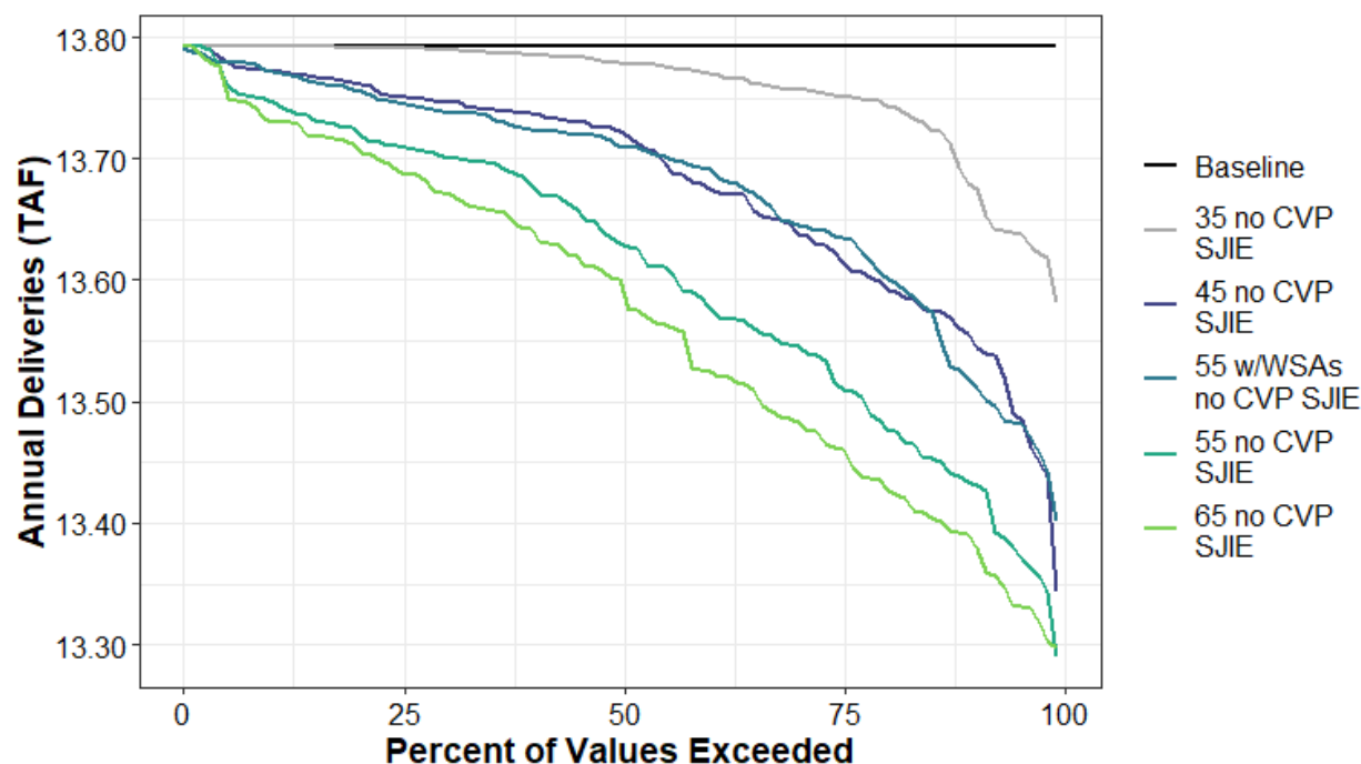
Figure H1a4-177. Total Water Supplied to Water Budget Areas 12 and 13 (Urban) Annual Percent Exceedance Plot.
