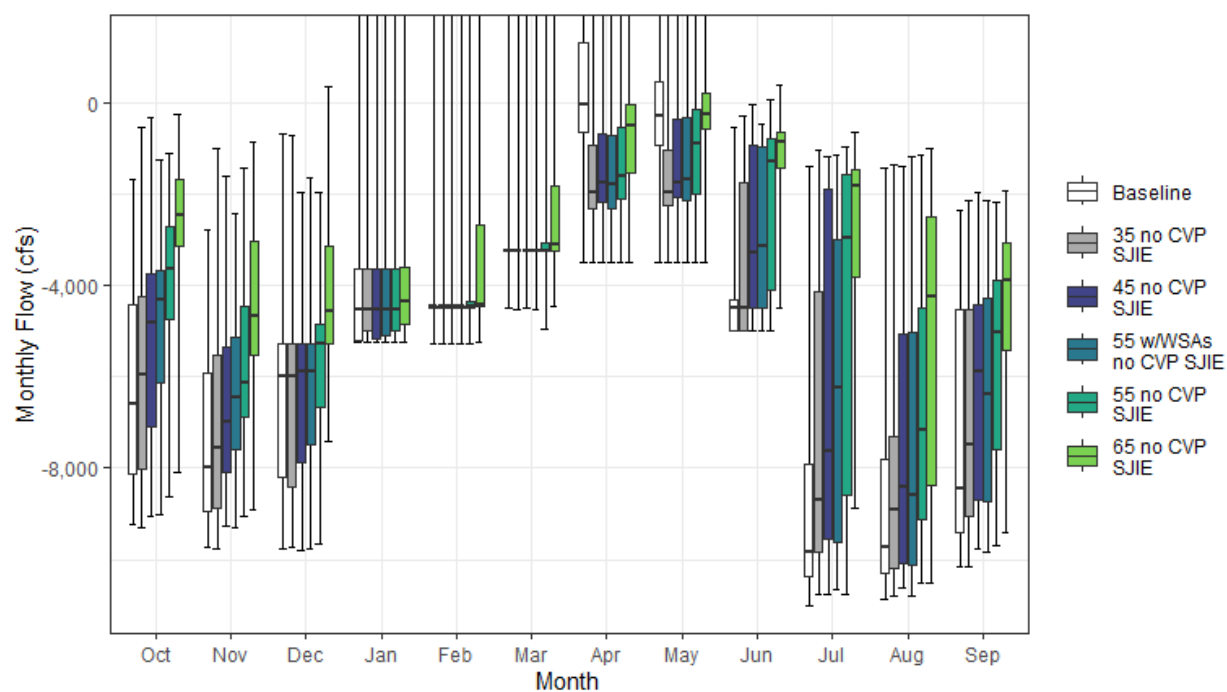
Figure H1a4-50. Old and Middle Rivers Net Flow Monthly Boxplot (cfs)
