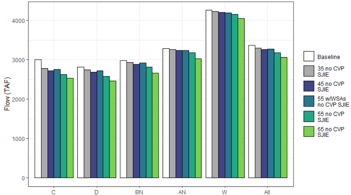
Figure H1a4-234. Total Average Annual Groundwater Recharge by WYT and Scenario (TAF/yr).
