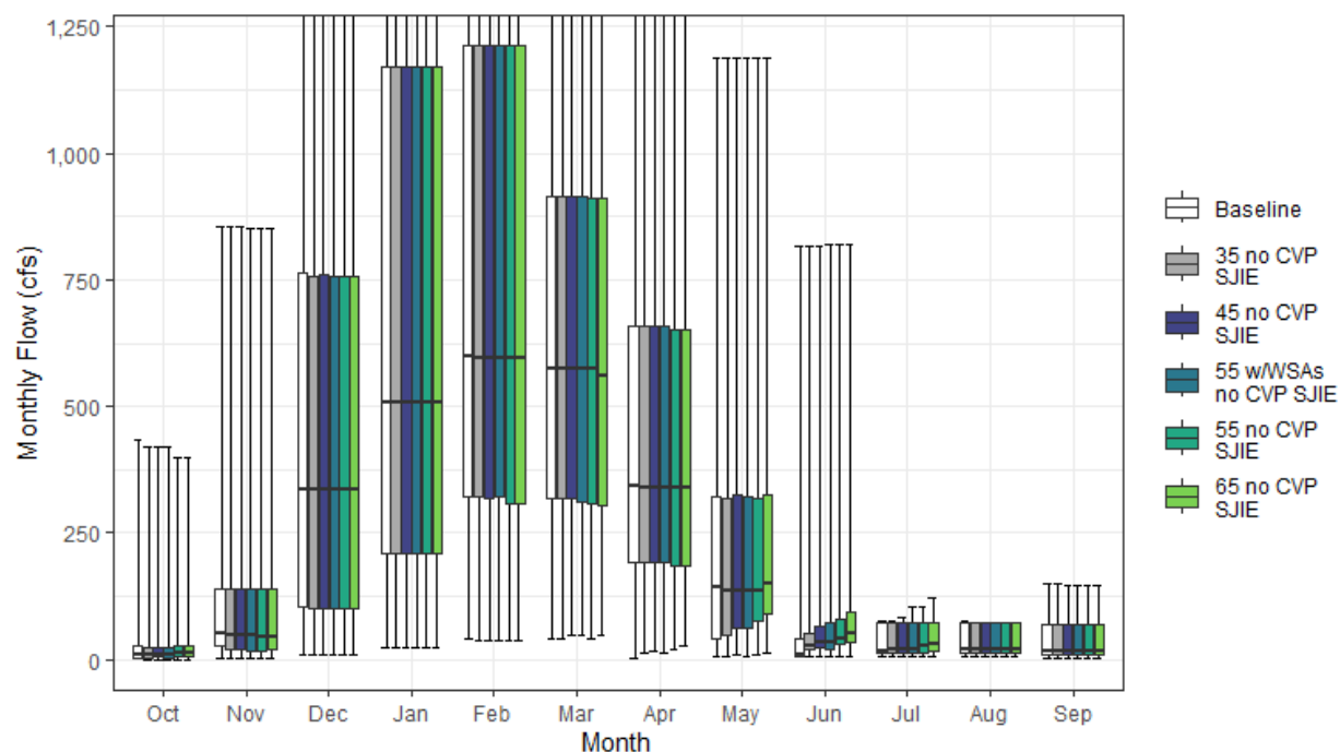
Figure H1a4-37. Thomes Creek Streamflow above Confluence with Sacramento River Monthly Boxplot (cfs)
