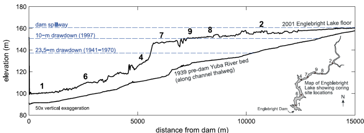
Figure H1b-2. Longitudinal Profile of Sediment Accumulation in Englebright Reservoir
