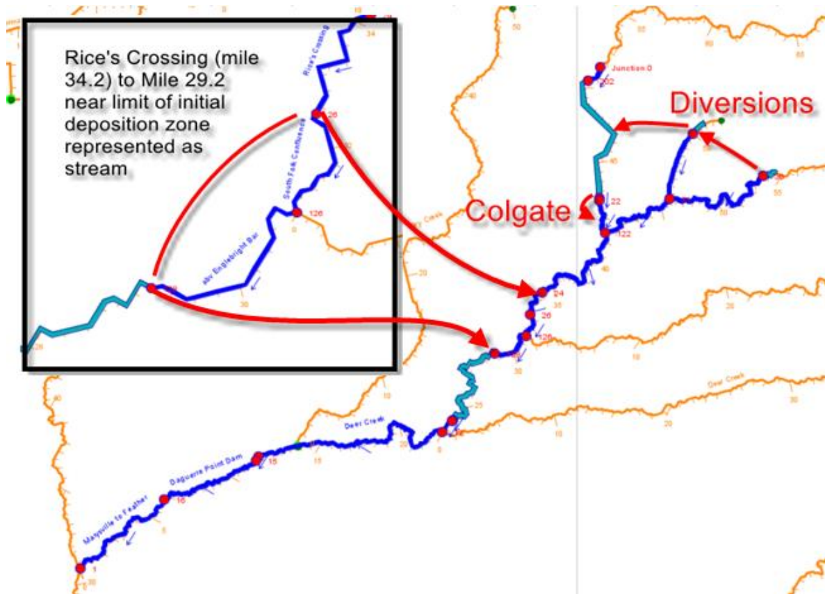
Figure H1b-1. Model Domain Covered by the Yuba River Water Temperature Model. (Blue Indicates River Channels Included in the Yuba River Water Temperature Model.)
