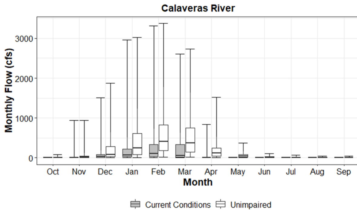
Figure 2.2-21. Calaveras River Simulated Current Conditions (gray) and Unimpaired (white) Monthly Flows
