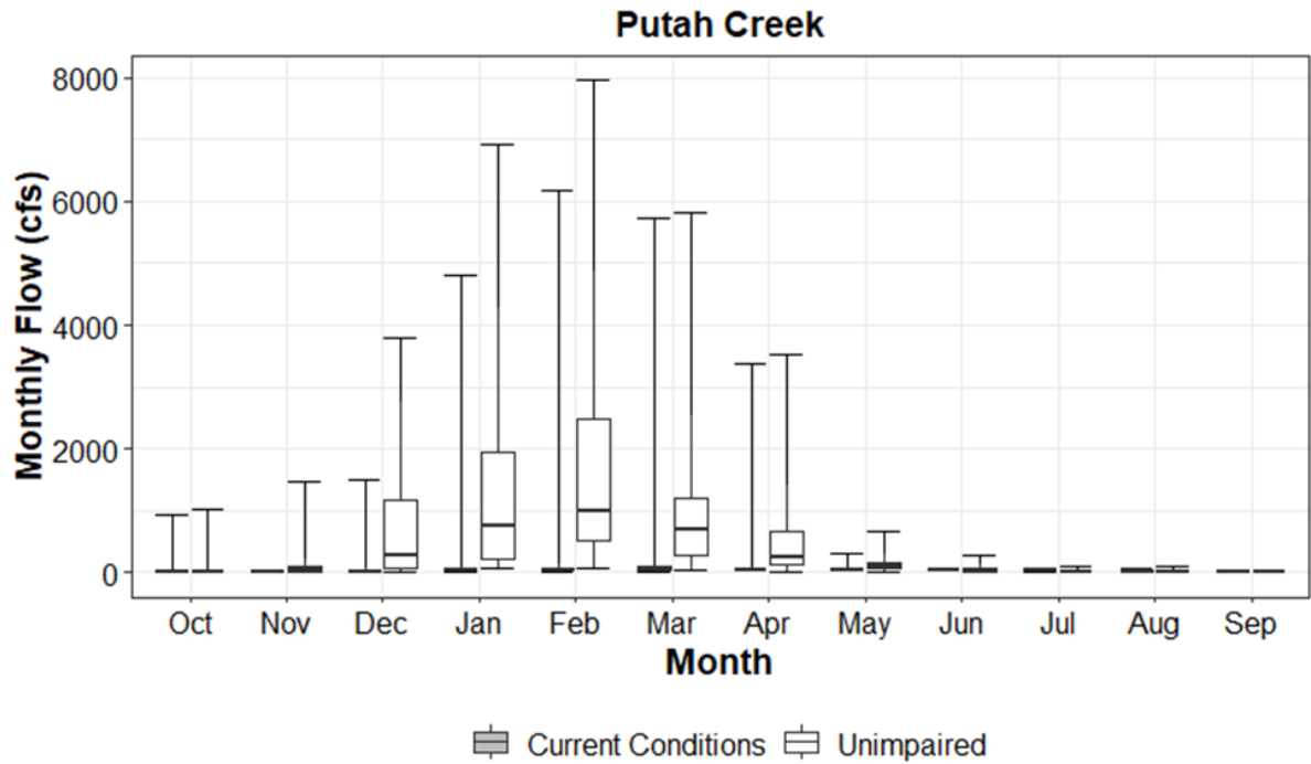
Figure 2.2-26. Putah Creek Simulated Current Conditions (gray) and Unimpaired (white) Monthly Flows
