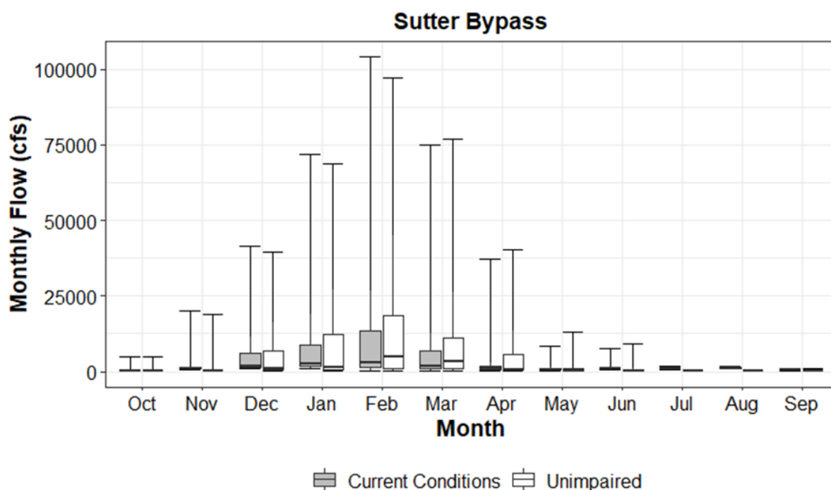
Figure 2.3-2. Sutter Bypass Simulated Current Conditions (gray) and Unimpaired (white) Monthly Flows
