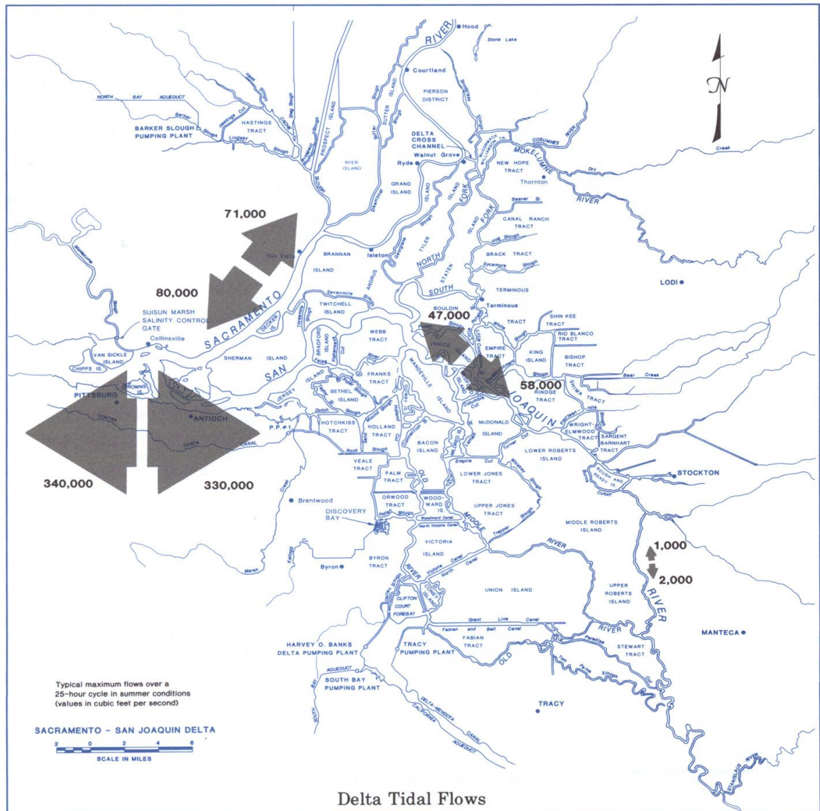
Figure 2.4-6. Delta Tidal Flows over a 25-Hour Cycle in Summer Conditions (values in cubic feet per second)
