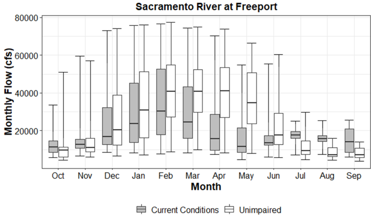
Figure 2.2-6. Sacramento River at Freeport Simulated Current Conditions (gray) and Unimpaired (white) Monthly Flows
