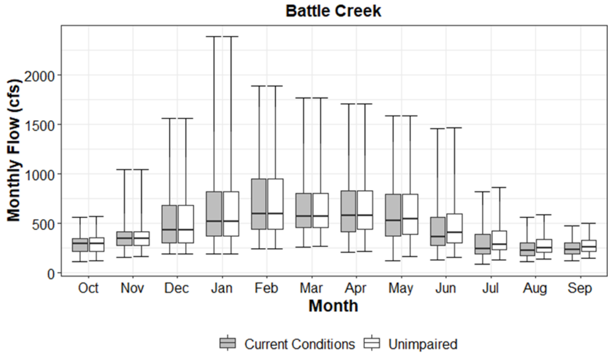
Figure 2.2-7. Battle Creek Simulated Current Conditions (gray) and Unimpaired (white) Monthly Flows
