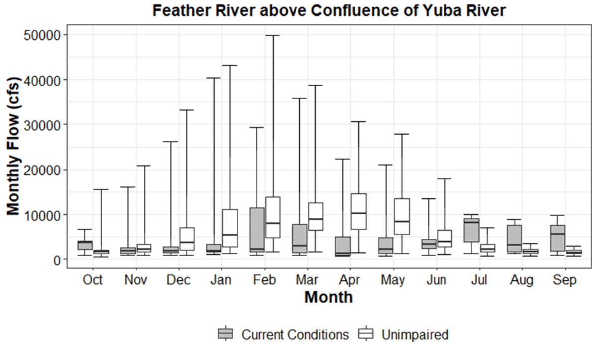
Figure 2.2-14. Feather River above Confluence with the Yuba River Simulated Current Conditions (gray) and Unimpaired (white) Monthly Flows
