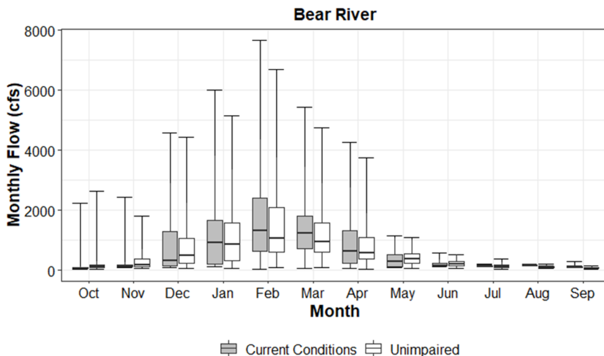
Figure 2.2-17. Bear River Simulated Current Conditions (gray) and Unimpaired (white) Monthly Flows
