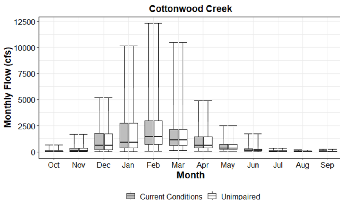
Figure 2.2-23. Cottonwood Creek Simulated Current Conditions (gray) and Unimpaired (white) Monthly Flows
