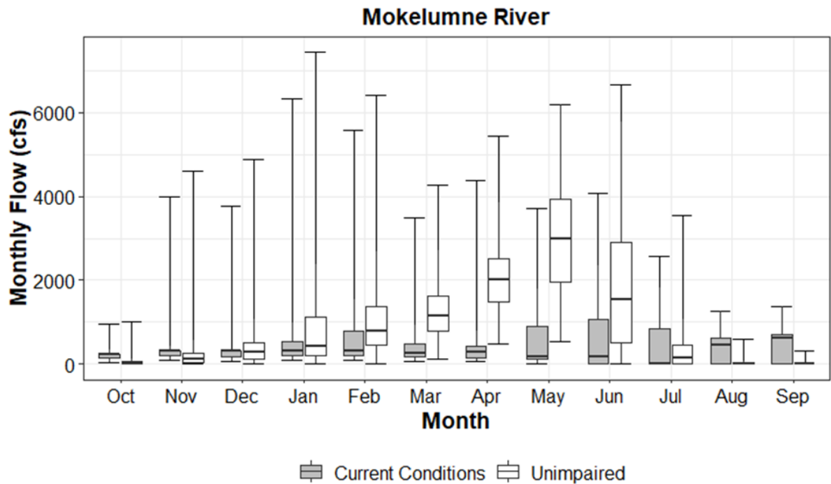
Figure 2.2-19. Mokelumne River Simulated Current Conditions (gray) and Unimpaired (white) Monthly Flows
