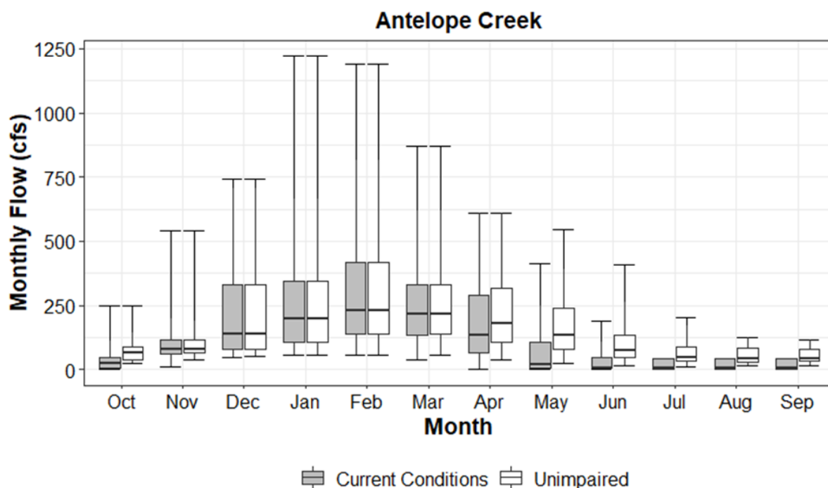
Figure 2.2-9. Antelope Creek Simulated Current Conditions (gray) and Unimpaired (white) Monthly Flows
