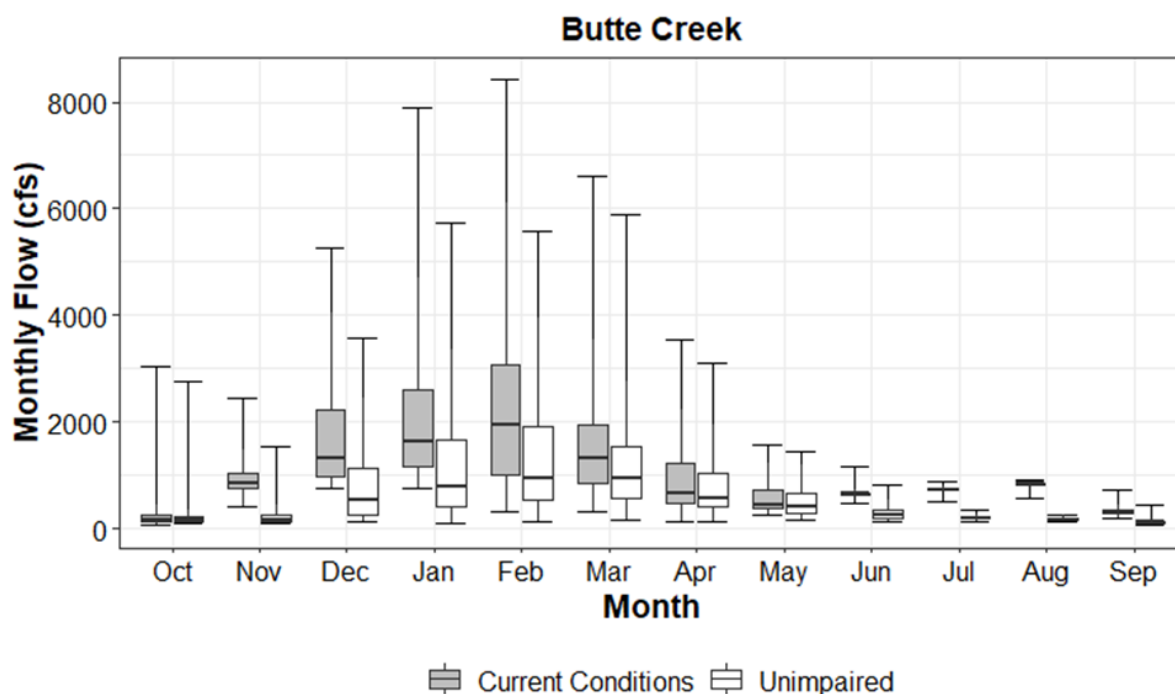
Figure 2.2-13. Butte Creek Simulated Current Conditions (gray) and Unimpaired (white) Monthly Flows
