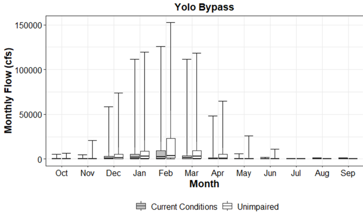
Figure 2.3-3. Yolo Bypass Simulated Current Conditions (gray) and Unimpaired (white) Monthly Flows
