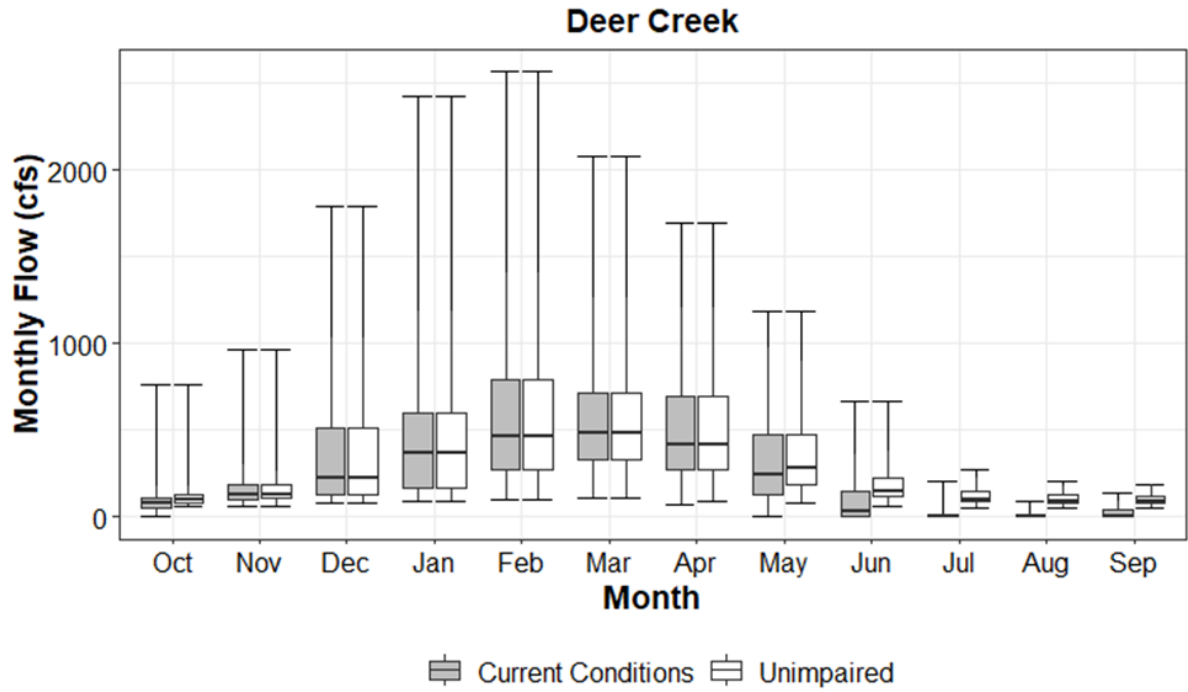
Figure 2.2-10. Deer Creek Simulated Current Conditions (gray) and Unimpaired (white) Monthly Flows
