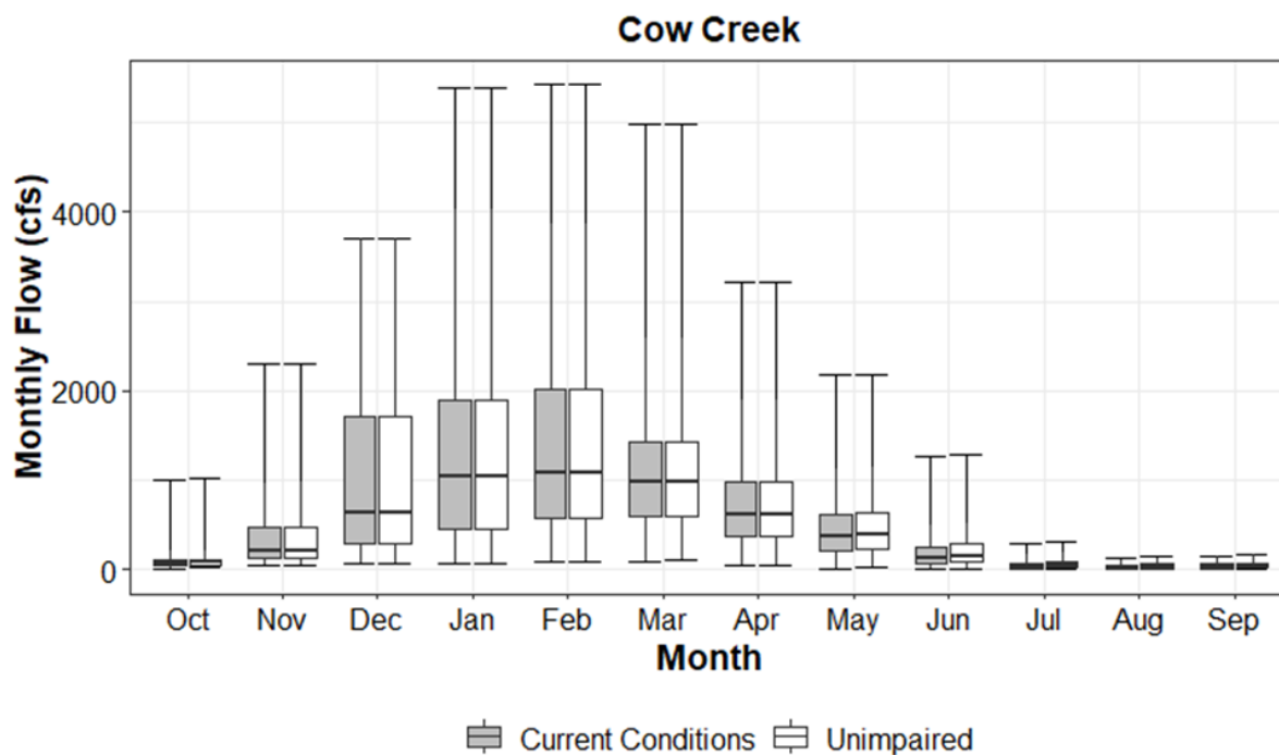
Figure 2.2-8. Cow Creek Simulated Current Conditions (gray) and Unimpaired (white) Monthly Flows
