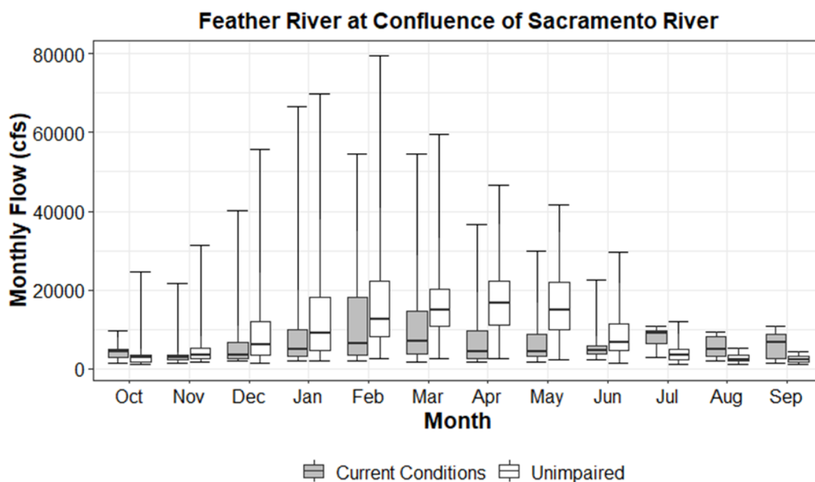
Figure 2.2-15. Feather River at Confluence with the Sacramento River Simulated Current Conditions (gray) and Unimpaired (white) Monthly Flows
