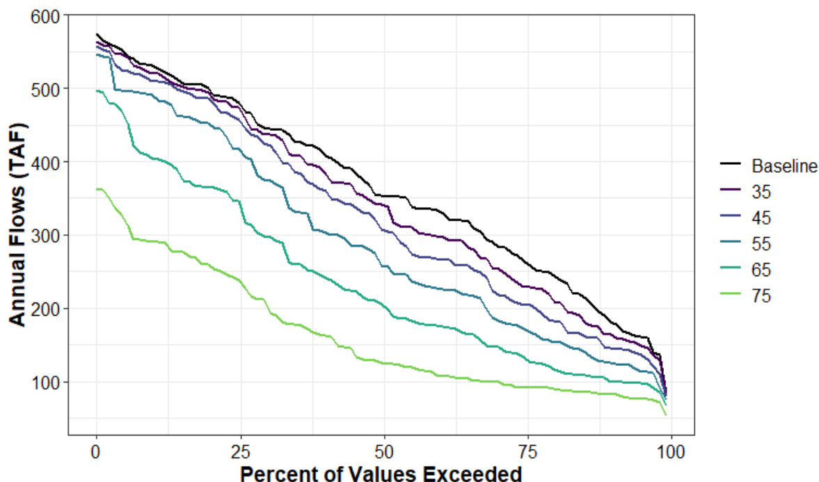
Figure 6.3-24. Exceedance Frequency Distribution of Annual Drum Canal Total Inflow (thousand acre-feet)
