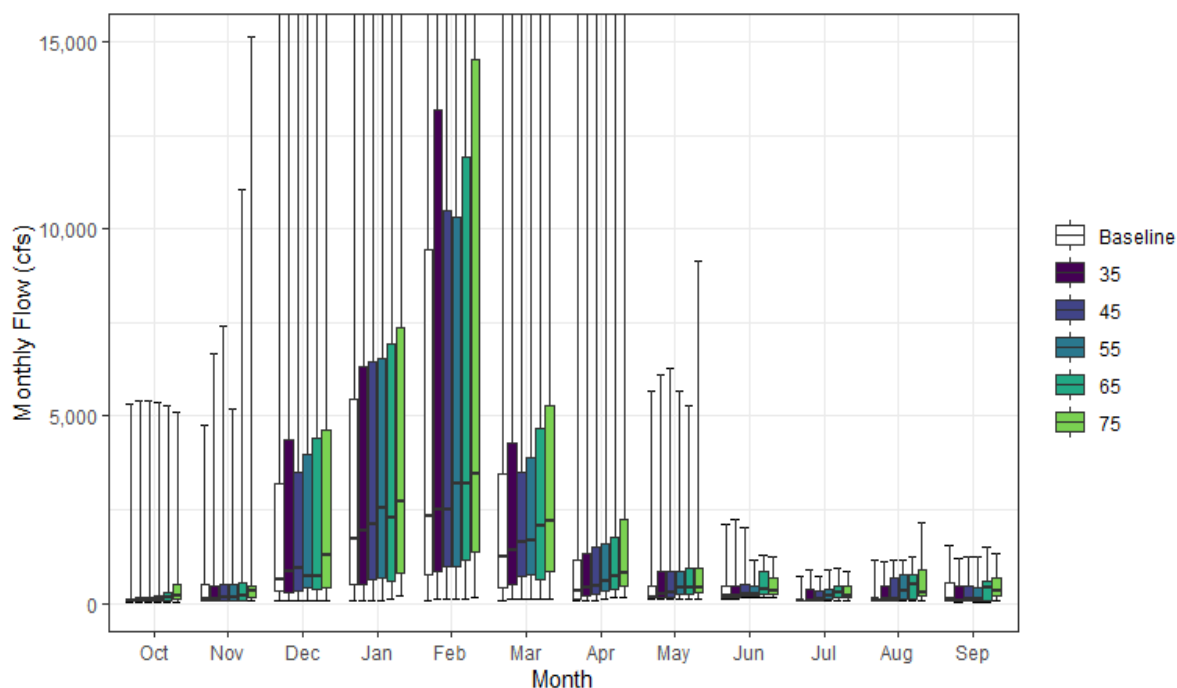
Figure 6.3-18. Changes in Hydrology across the Scenarios for Yolo Bypass below Putah Creek Inflow
