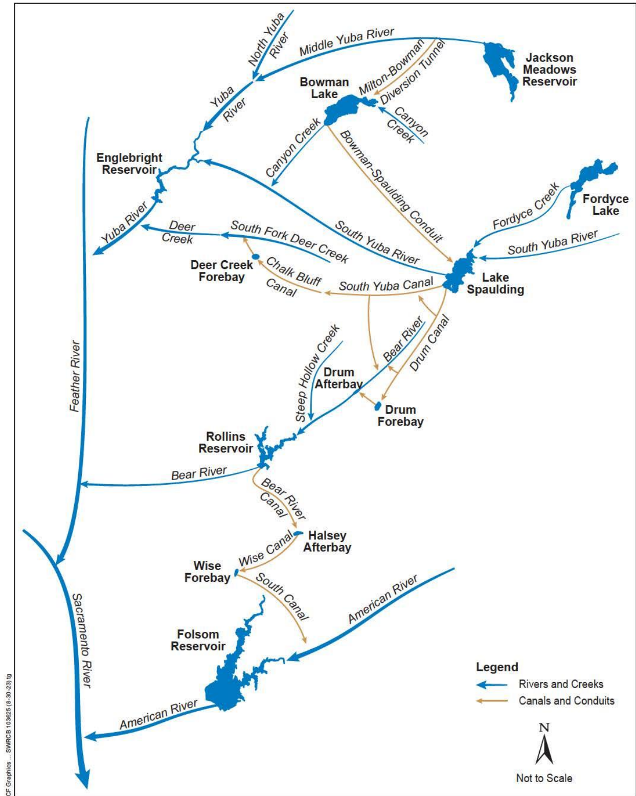
Figure 6.3-23. Example of an Interbasin Diversion (Yuba-Bear Project)
