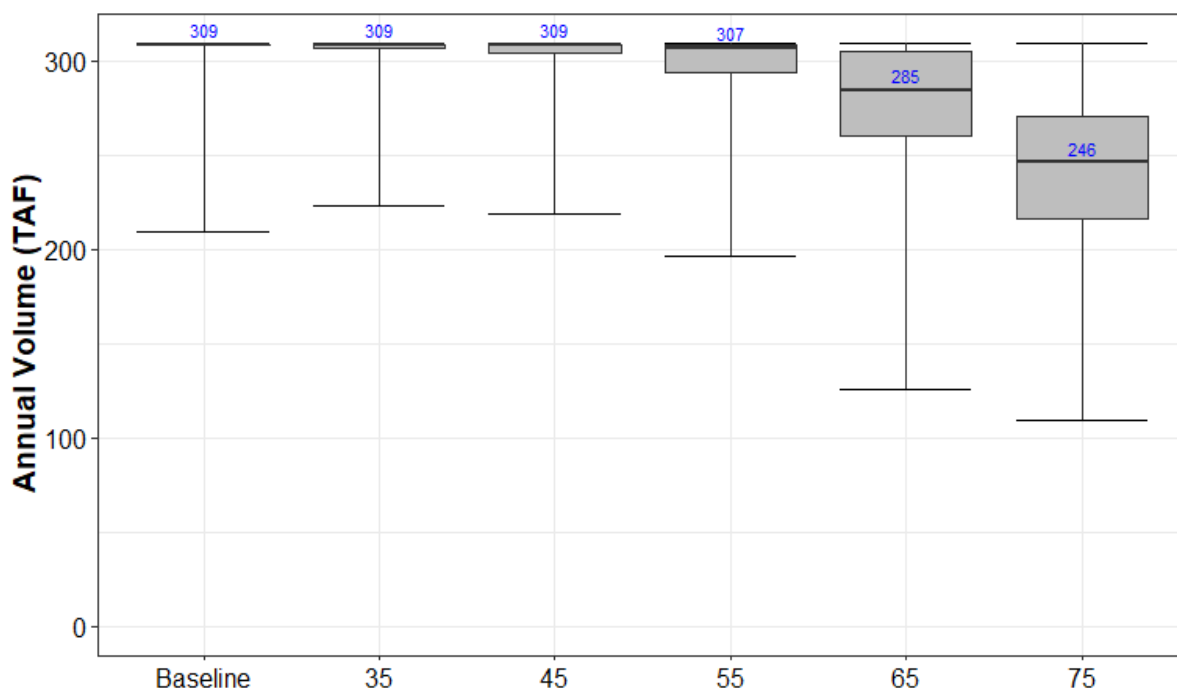
Figure 6.4-13. Sacramento/Delta Supply to Wildlife Refuges in the San Joaquin Valley Region
