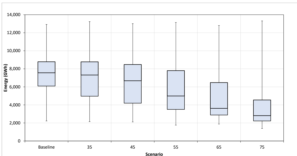
Figure 7.8-13. Estimated Annual Changes in Energy Required for CVP and SWP Exports
