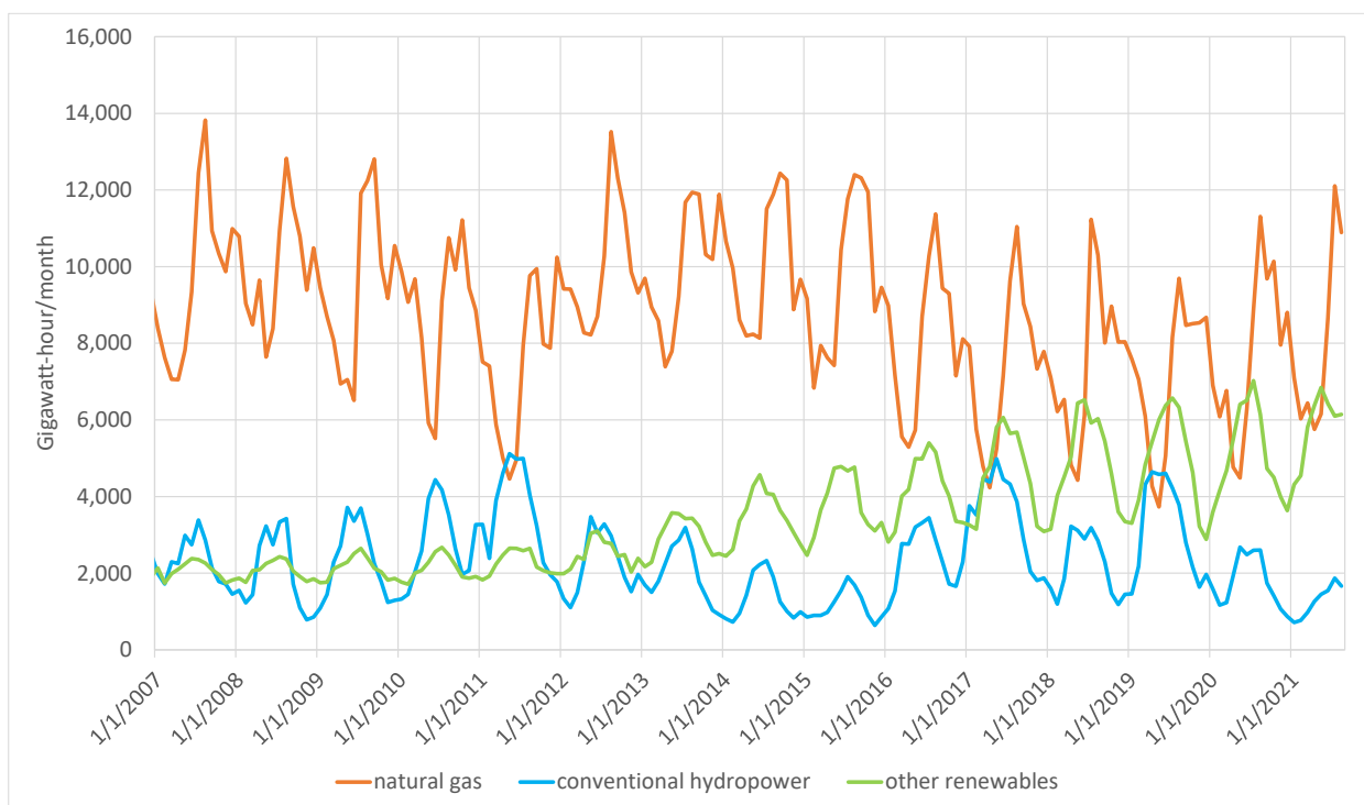
Figure 7.8-9. Monthly Natural Gas, Conventional Hydropower, and Other Renewable Electrical Production in California 2007–2021
