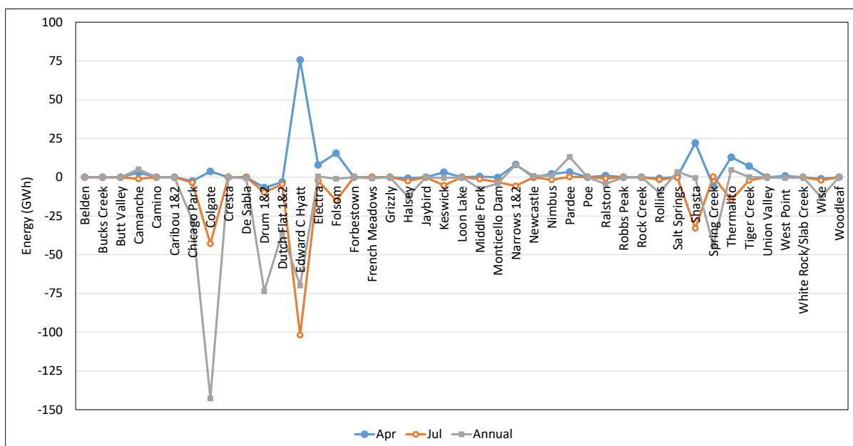
Figure 7.8-14. Estimated Average Change in Hydropower Generation for the 55 Scenario at Individual Hydropower Facilities
