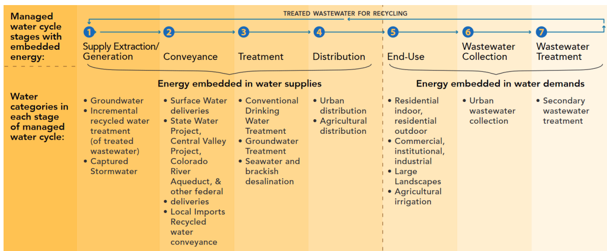
Figure 7.8-3. Stages of the Water Cycle with Embedded Energy—California Water Sector
