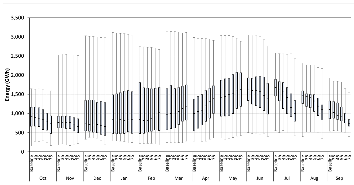
Figure 7.8-10. Monthly Hydropower Generation for Sacramento River Watershed and Delta Eastside Tributaries Regions—Facilities Potentially Subject to Changes in Flow as Simulated by SacWAM
