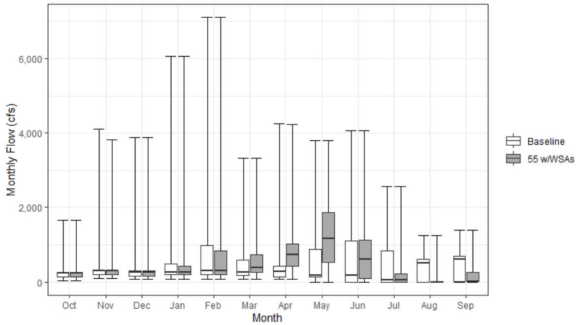
Figure 13.4-12. Monthly Streamflow for the Mokelumne River above the Confluence with the Cosumnes River under the Baseline and 55 w/WSAs Scenarios
