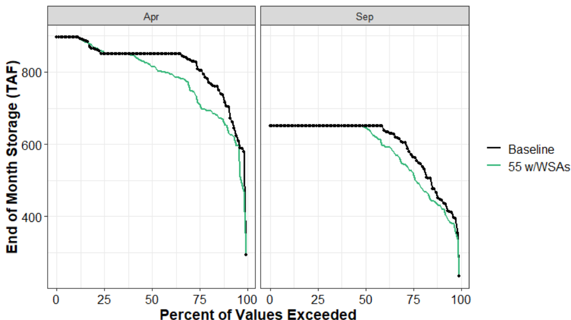
Figure 13.4-44. New Bullards Bar Reservoir End-of-April and End-of-September Carryover Storage under the Baseline and 55 w/WSAs Scenarios
