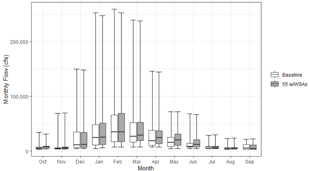
Figure 13.4-36. Monthly Delta Outflow under the Baseline and 55 w/WSAs Scenarios
