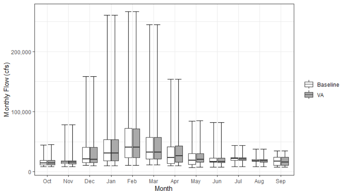
Figure 13.4-29. Monthly Delta Inflow under the Baseline and VA Scenarios
