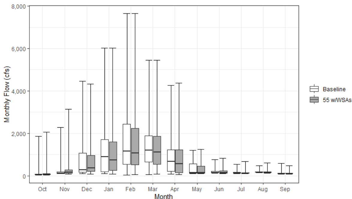
Figure 13.4-11. Monthly Streamflow for the Bear River above the Feather River under the Baseline and 55 w/WSAs Scenarios
