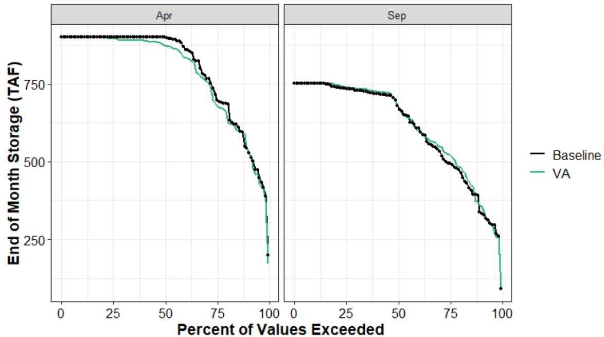
Figure 13.4-51. Folsom Lake End-of-April and End-of-September Carryover Storage under the Baseline and VA Scenarios
