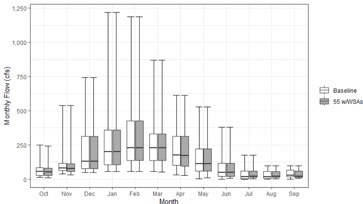
Figure 13.4-21. Monthly Streamflow for Antelope Creek under the Baseline and 55 w/WSAs Scenarios
