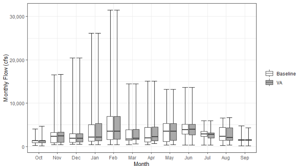
Figure 13.4-2. Monthly Streamflow for the American River above the Sacramento River under the Baseline and VA Scenarios
