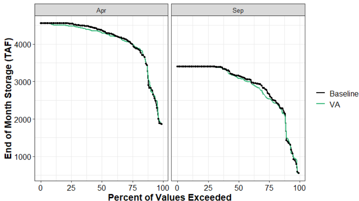
Figure 13.4-55. Shasta Reservoir End-of-April and End-of-September Carryover Storage under the Baseline and VA Scenarios
