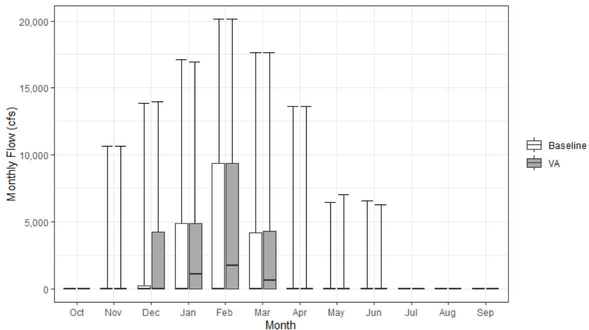
Figure 13.4-26. Monthly Streamflow over the Tisdale Weir into the Sutter Bypass under the Baseline and VA Scenarios
