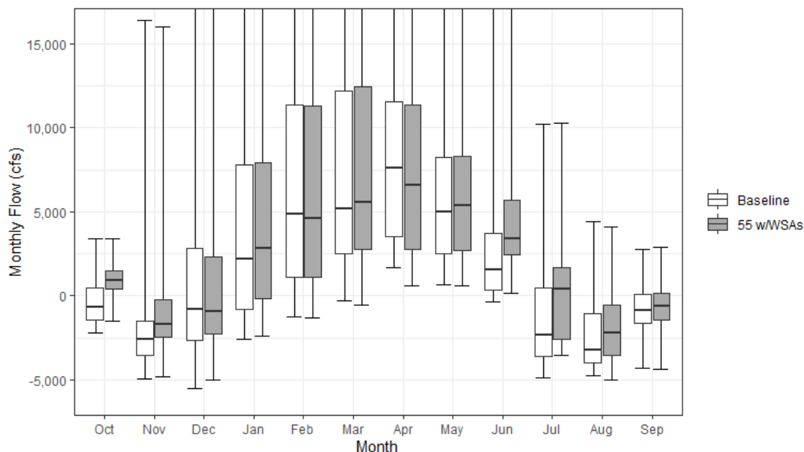
Figure 13.4-33. QWEST under the Baseline and 55 w/WSAs Scenarios
