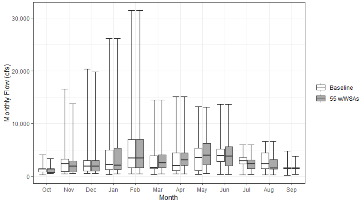
Figure 13.4-1. Monthly Streamflow for the American River above the Sacramento River under Baseline and 55 w/WSAs Scenarios
