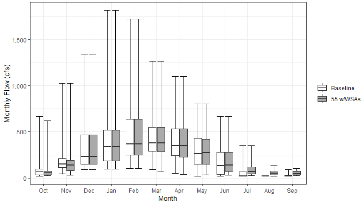
Figure 13.4-19. Monthly Streamflow for Mill Creek under the Baseline and 55 w/WSAs Scenarios
