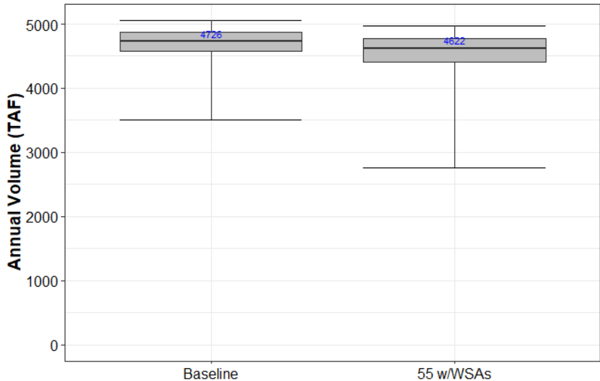
Figure 13.4-60. Annual Sacramento/Delta Supply to Agriculture in the Sacramento River Watershed for Baseline and 55 w/WSAs Scenarios
