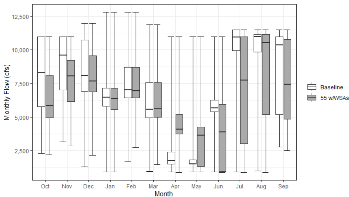
Figure 13.4-30. Monthly South of Delta Exports for the Baseline and 55 w/WSAs Scenarios
