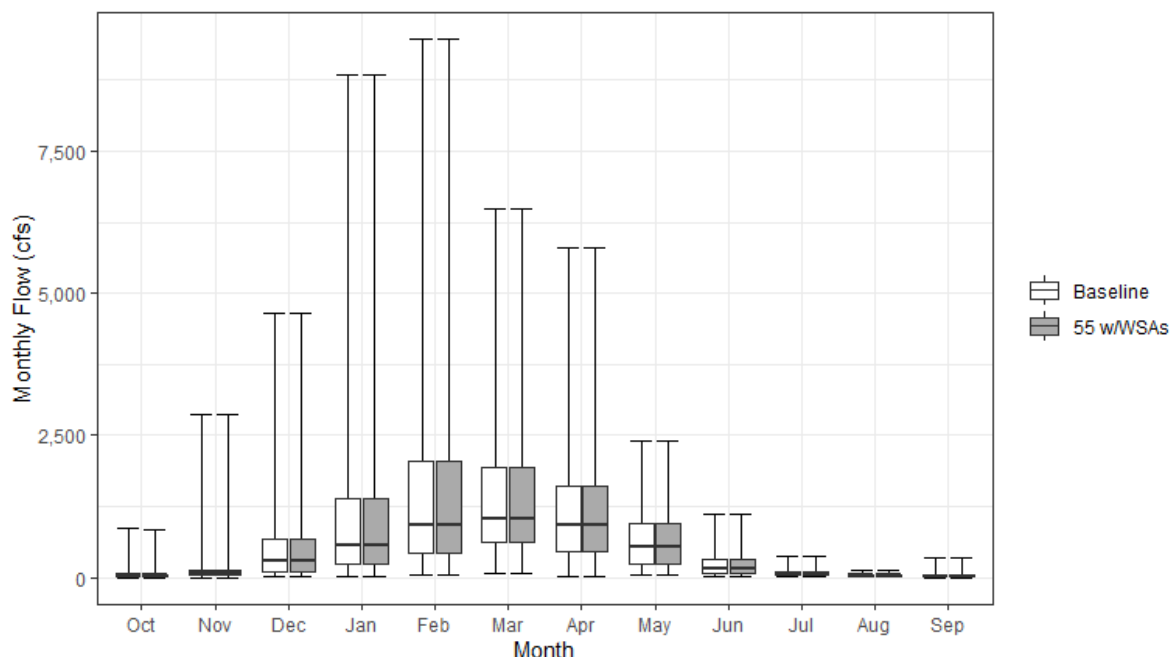
Figure 13.4-18. Monthly Streamflow for the Cosumnes River under the Baseline and 55 w/WSAs Scenarios
