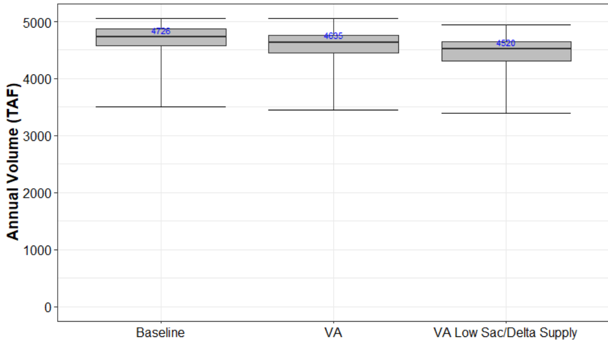
Figure 13.4-64. Annual Sacramento/Delta Supply to Agriculture in the Sacramento River Watershed for Baseline and VA Scenarios
