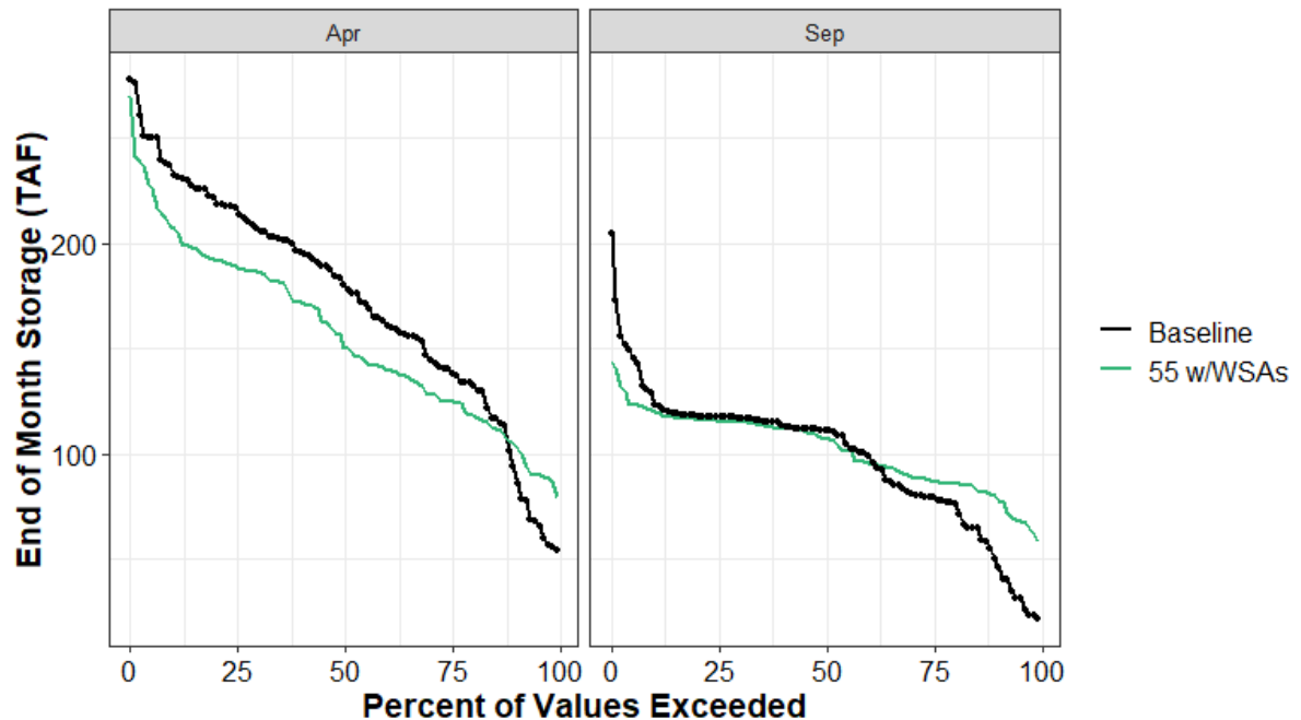
Figure 13.4-45. New Hogan Reservoir End-of-April and End-of-September Carryover Storage under the Baseline and 55 w/WSAs Scenarios
