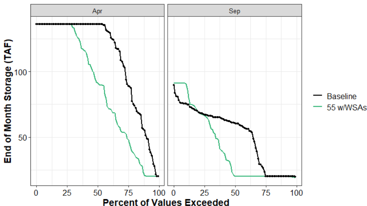
Figure 13.4-38. Black Butte Reservoir End-of-April and End-of-September Carryover Storage under the Baseline and 55 w/WSAs Scenarios
