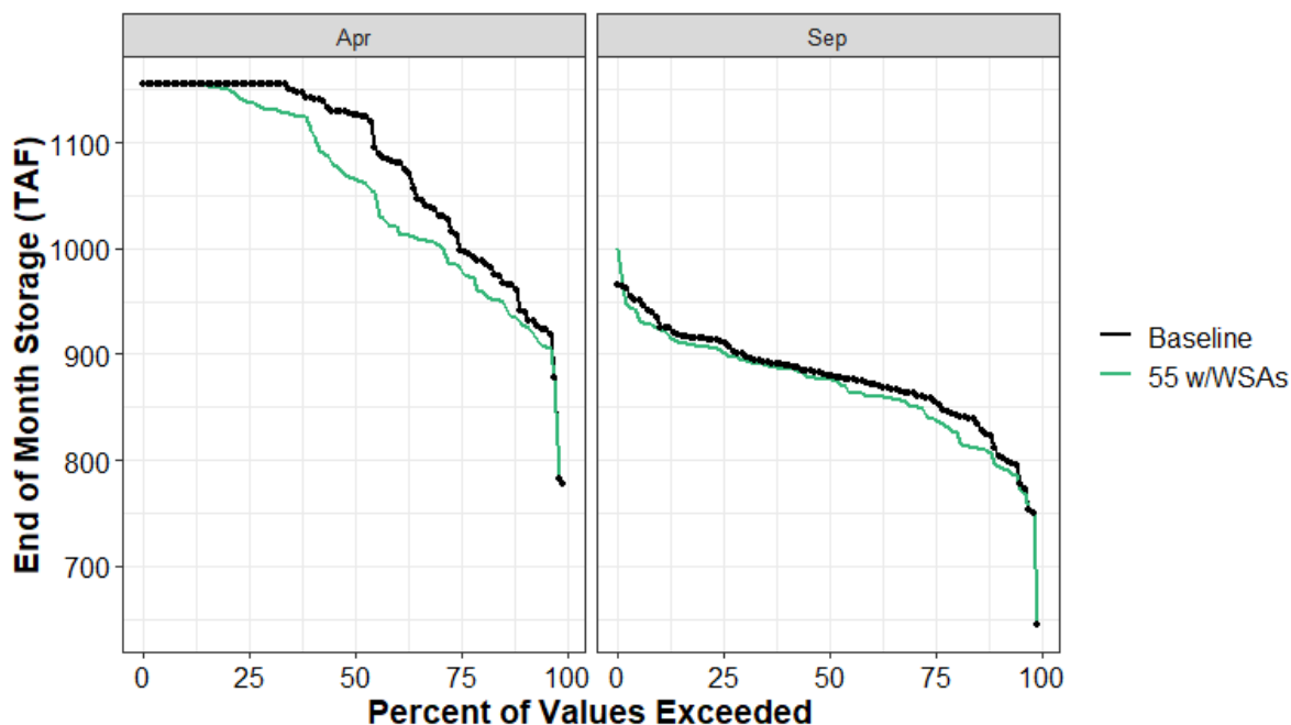
Figure 13.4-41. Clear Lake End-of-April and End-of-September Carryover Storage under the Baseline and 55 w/WSAs Scenarios
