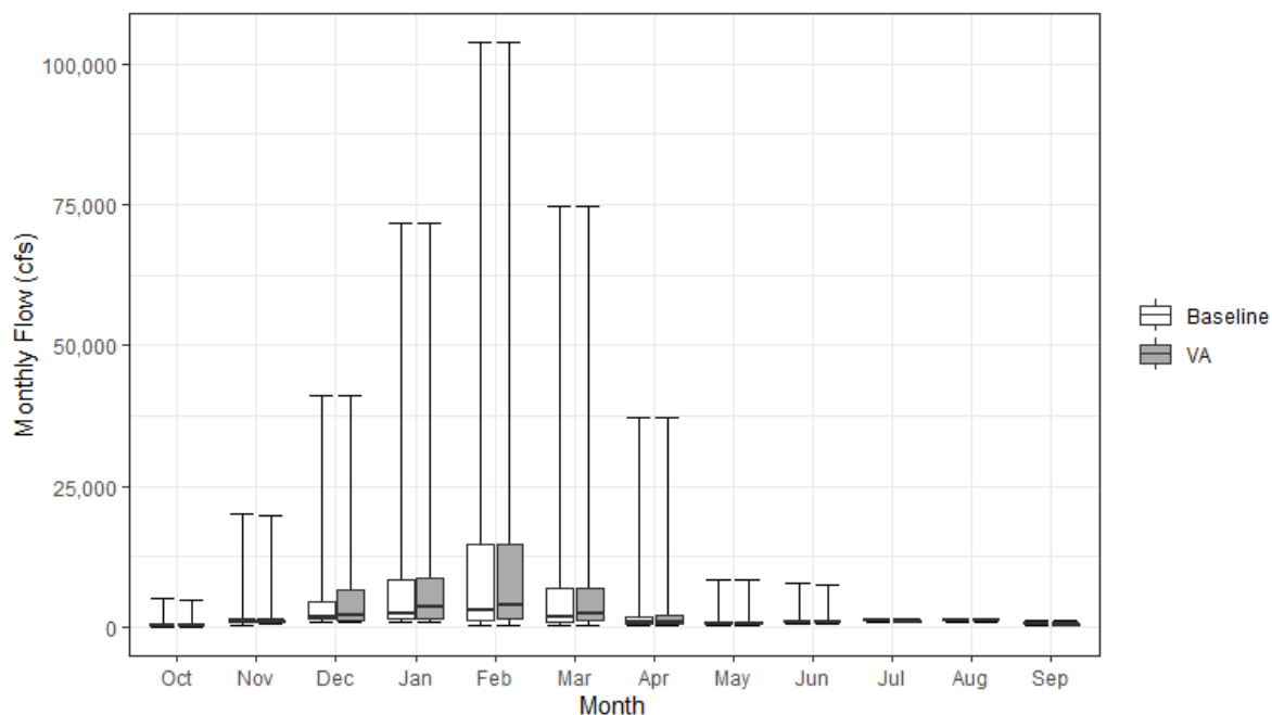
Figure 13.4-27. Monthly Streamflow at Sacramento Slough (Downstream End of Sutter Bypass) under the Baseline and VA Scenarios
