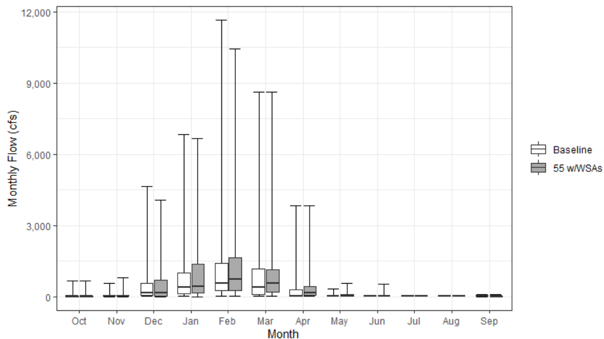
Figure 13.4-17. Monthly Streamflow for Cache Creek above the Yolo Bypass under the Baseline and 55 w/WSAs Scenarios
