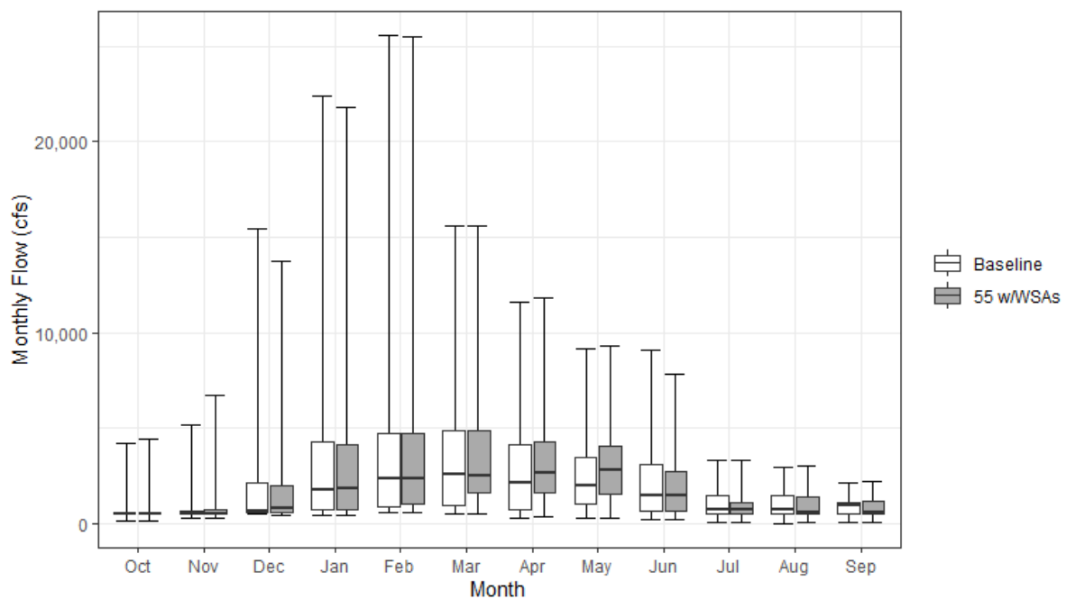
Figure 13.4-9. Monthly Streamflow for the Yuba River above the Feather River under Baseline and 55 w/WSAs
