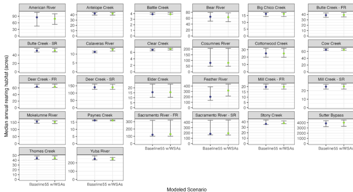
Figure 13.5-2. Median (across All Years Modeled) Rearing Habitat (acres)
