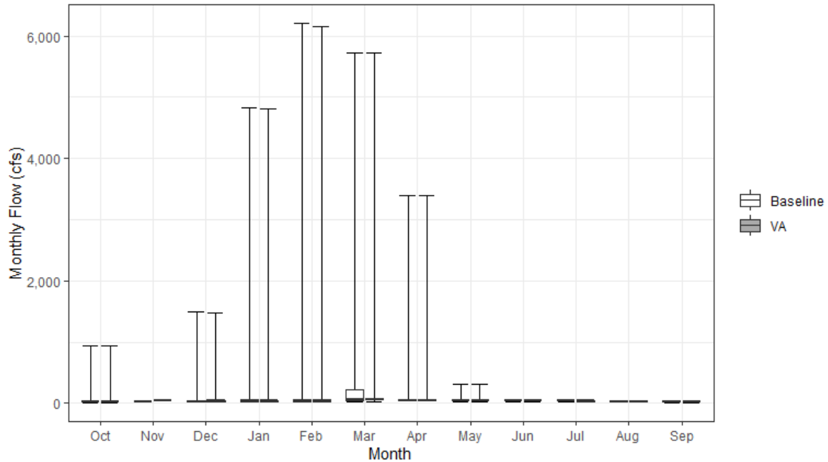
Figure 13.4-16. Monthly Streamflow for Putah Creek above the Yolo Bypass under the Baseline and VA Scenarios
