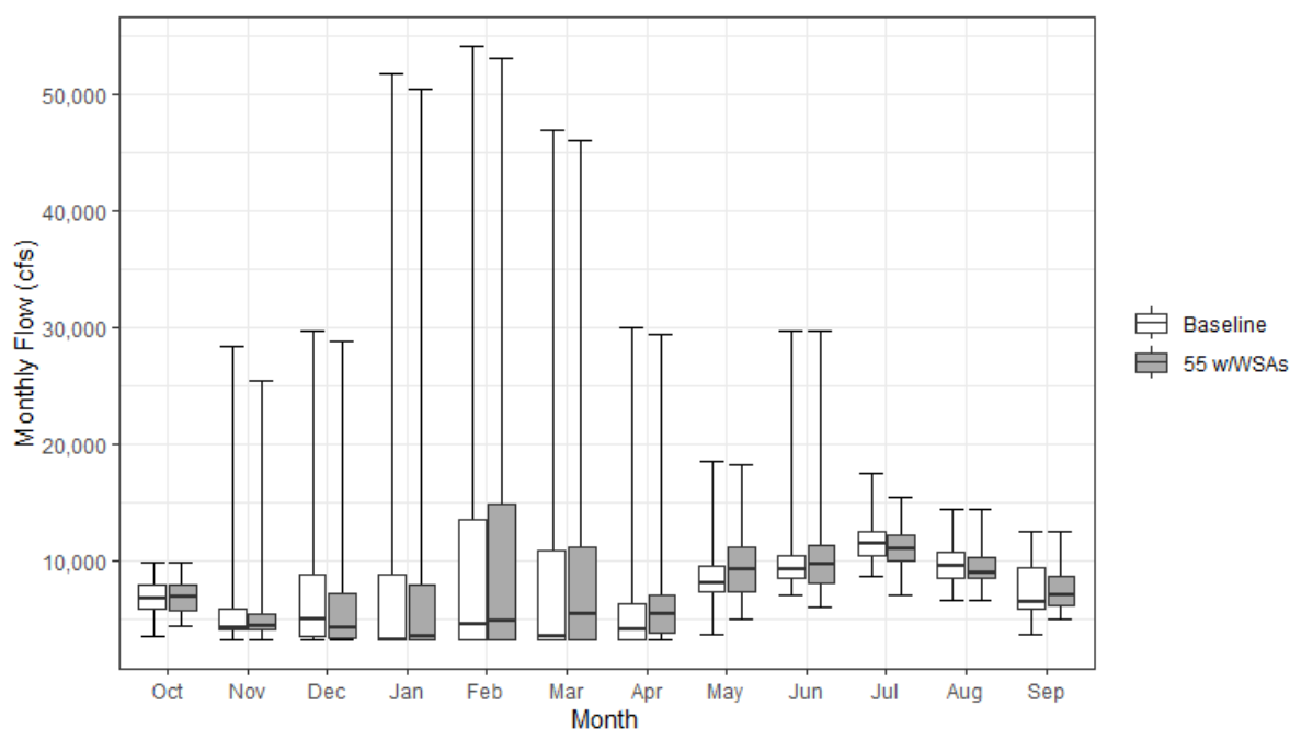
Figure 13.4-5. Monthly Streamflow for the Sacramento River below Keswick Reservoir under the Baseline and 55 w/WSAs Scenarios
