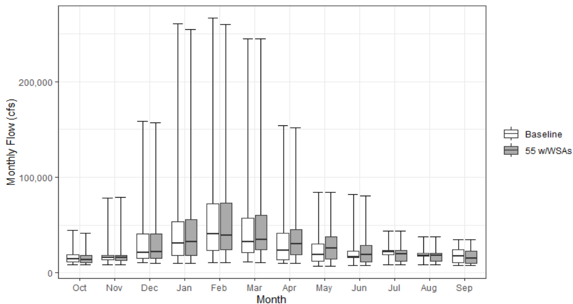
Figure 13.4-28. Monthly Delta Inflow under the Baseline and 55 w/WSAs Scenarios
