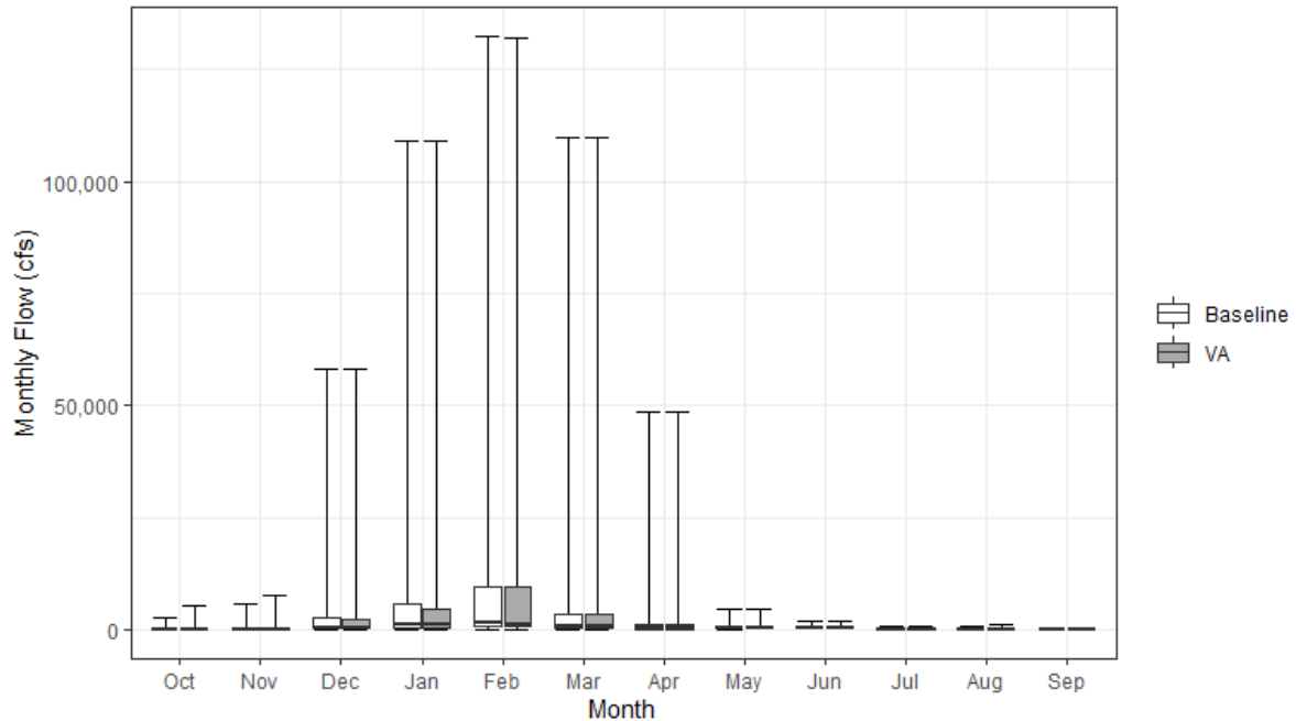
Figure 13.4-25. Monthly Streamflow for Yolo Bypass below Putah Creek Inflow under the Baseline and VA Scenarios
