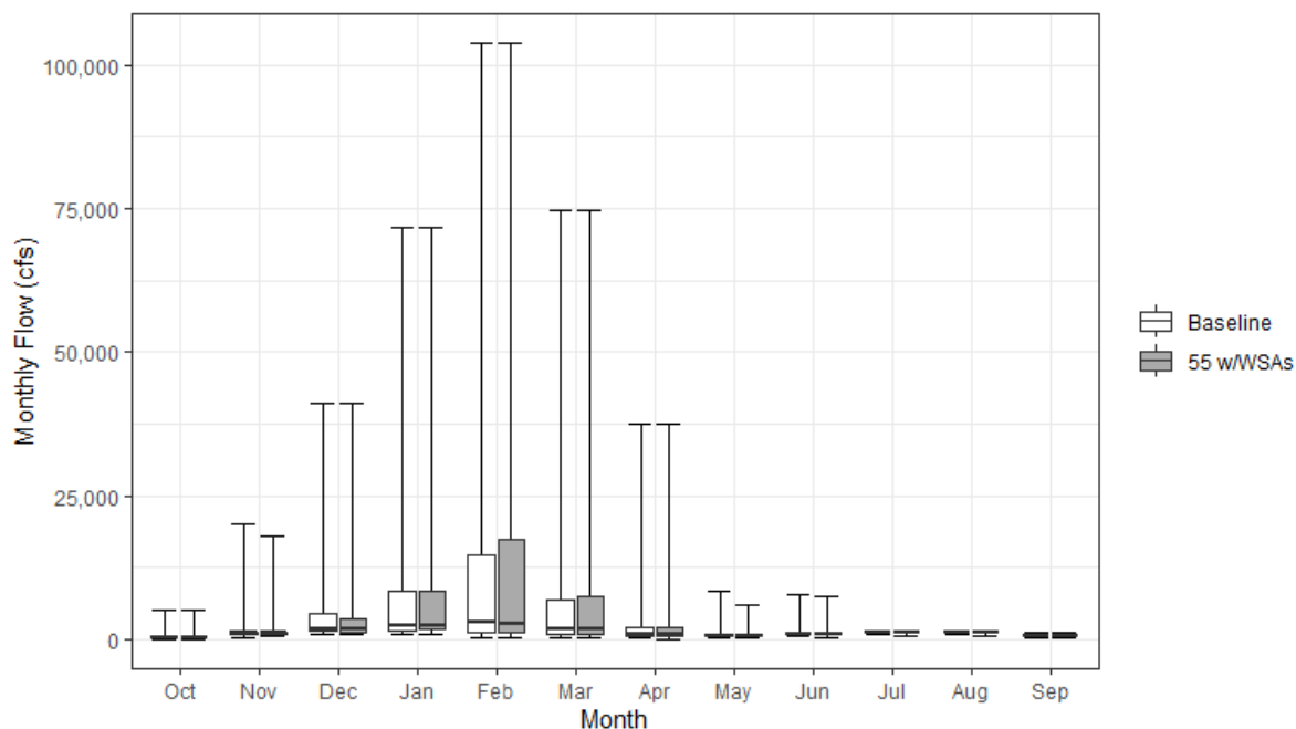
Figure 13.4-24. Monthly Streamflow at Sacramento Slough (Downstream End of Sutter Bypass) under the Baseline and 55 w/WSAs Scenarios
