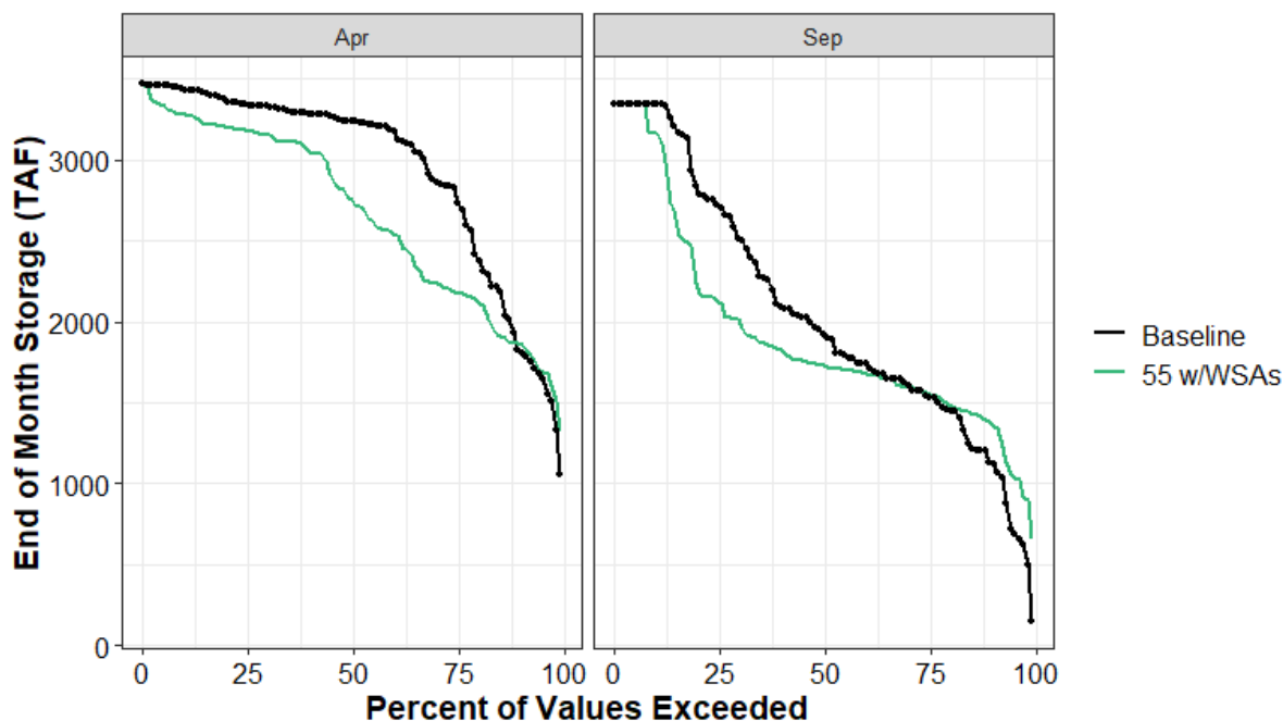
Figure 13.4-46. Oroville Reservoir End-of-April and End-of-September Carryover Storage under the Baseline and 55 w/WSAs Scenarios
