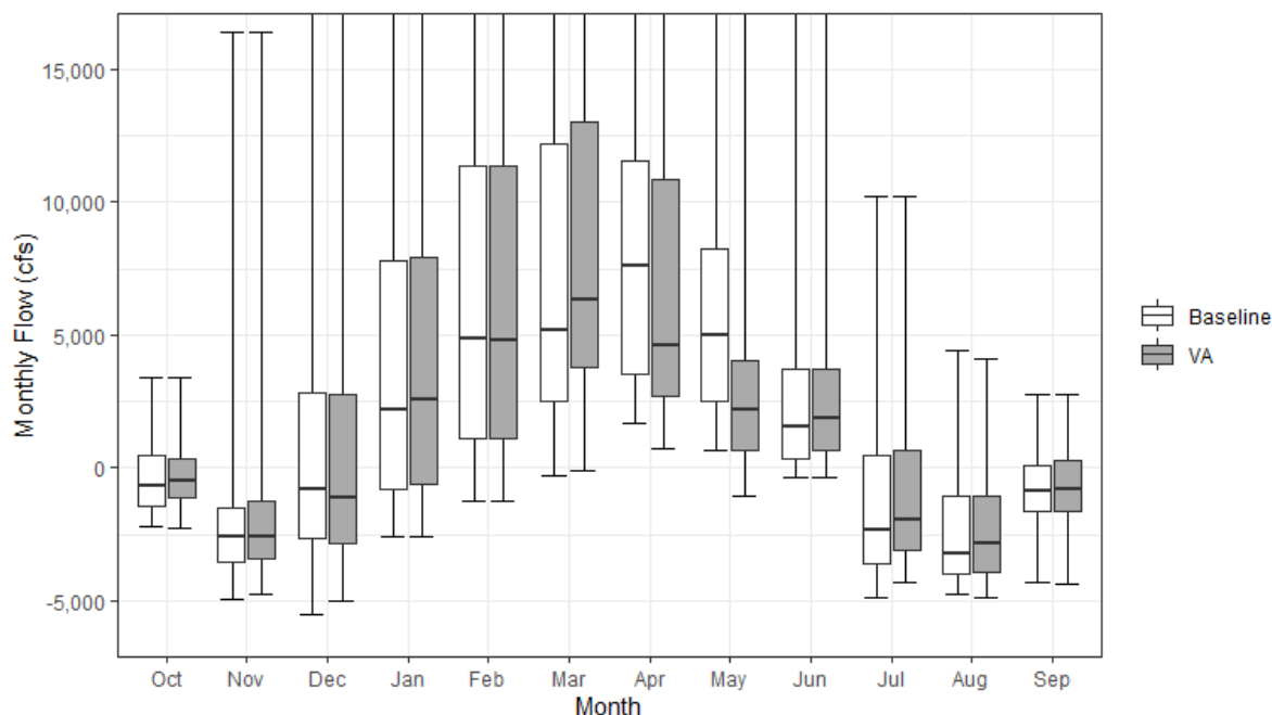
Figure 13.4-35. QWEST under the Baseline and VA Scenarios
