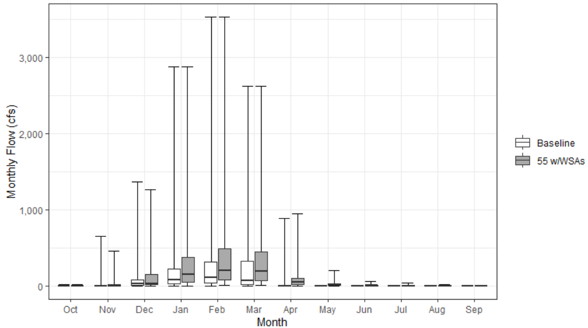
Figure 13.4-14. Monthly Streamflow for the Calaveras River Inflow to the Delta under the Baseline and 55 w/WSAs Scenarios
