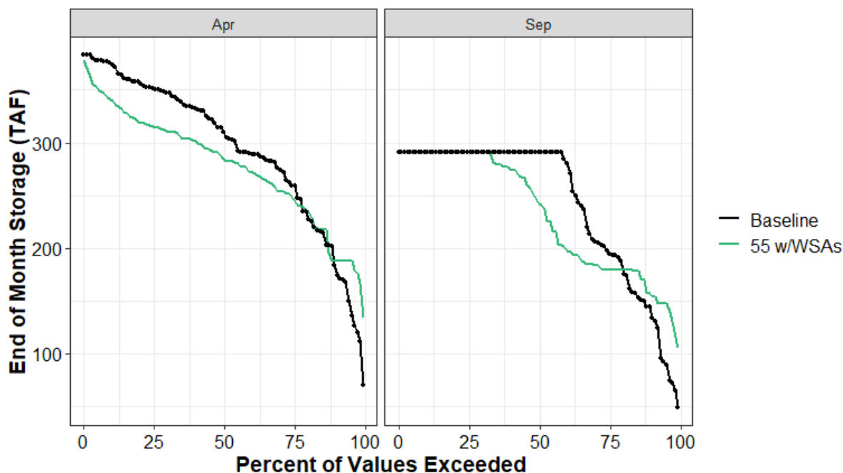
Figure 13.4-39. Camanche Reservoir End-of-April and End-of-September Carryover Storage under the Baseline and 55 w/WSAs Scenarios
