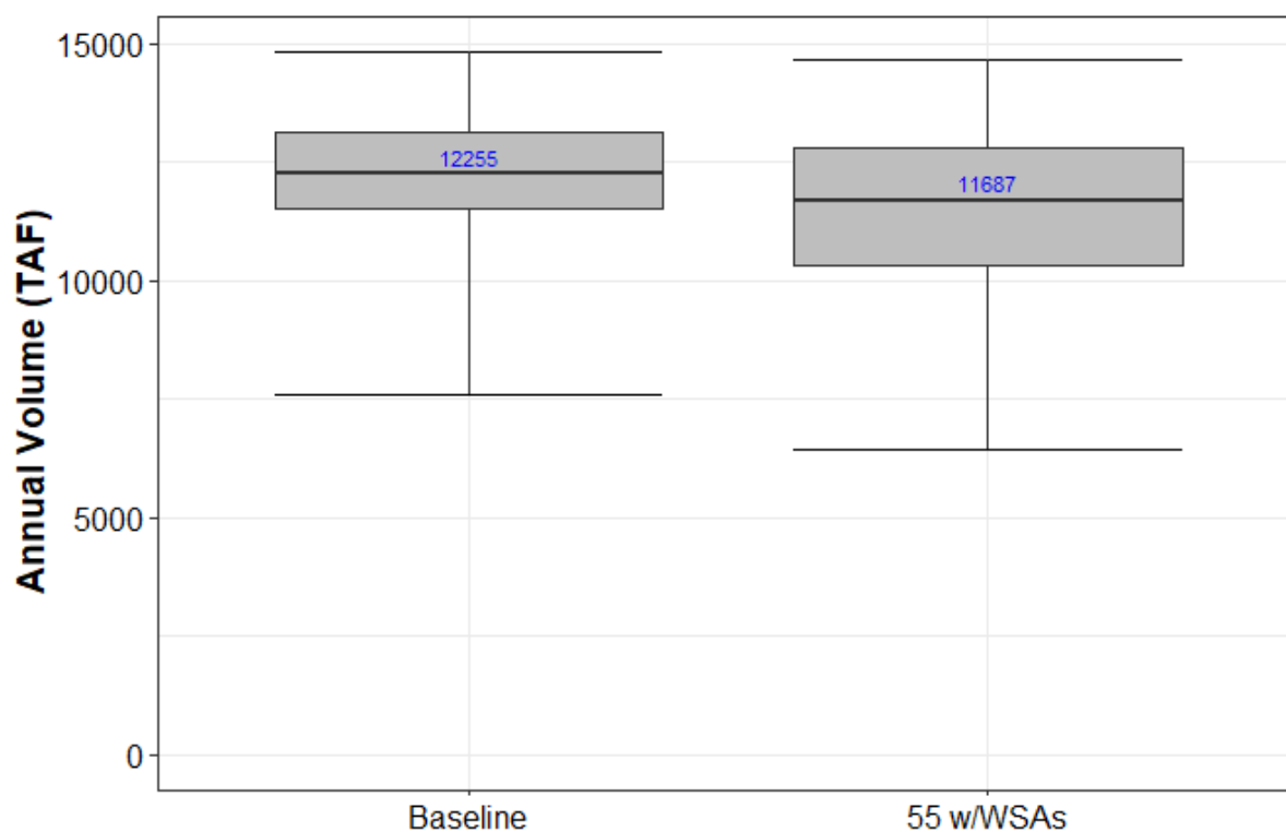
Figure 13.4-57. Annual Total Sacramento/Delta Supply for Baseline and 55 w/WSAs Scenarios
