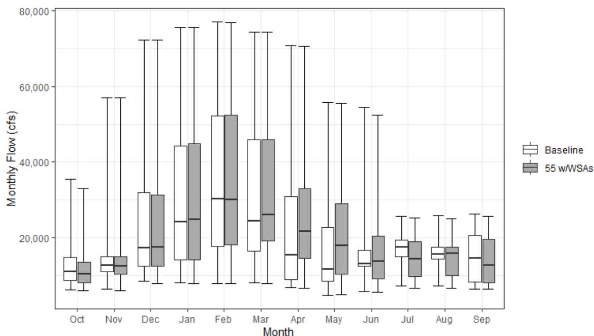
Figure 13.4-6. Monthly Streamflow for the Sacramento River at Freeport under the Baseline and 55 w/WSAs Scenarios
