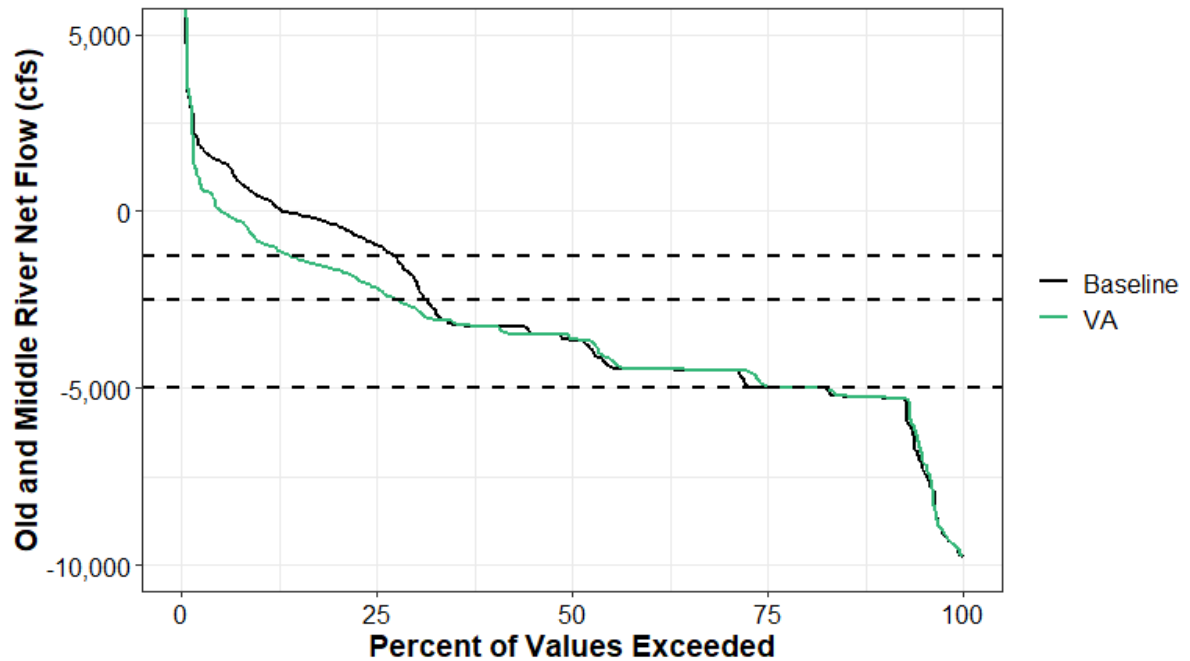
Figure 13.4-34. Monthly Exceedance Frequency Distribution of Old and Middle River Net Flow (cfs) for December–June under the Baseline and VA Scenarios
