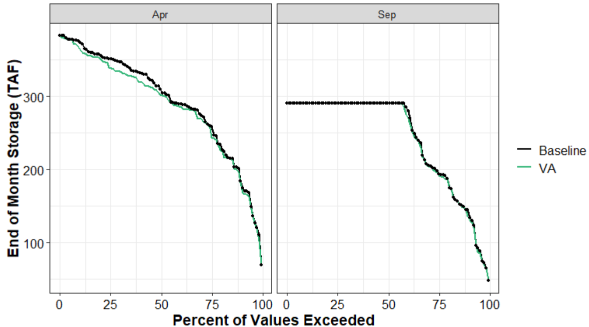
Figure 13.4-50. Camanche Reservoir End-of-April and End-of-September Carryover Storage under the Baseline and VA Scenarios
