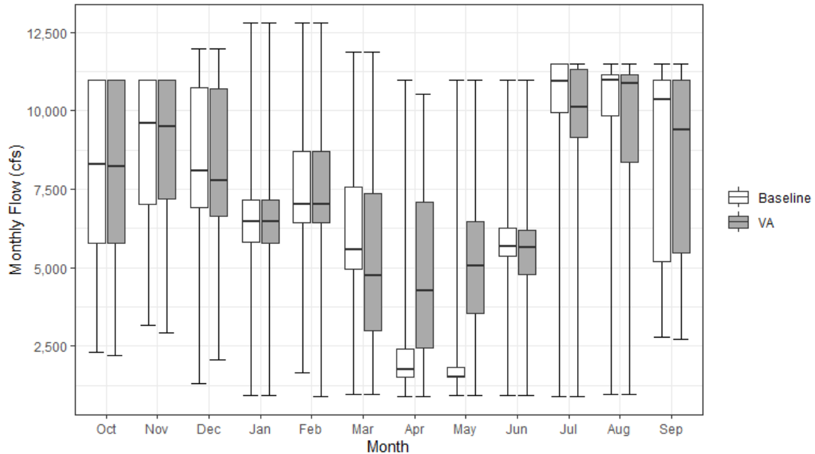
Figure 13.4-31. Monthly South of Delta Exports for the Baseline and VA Scenarios
