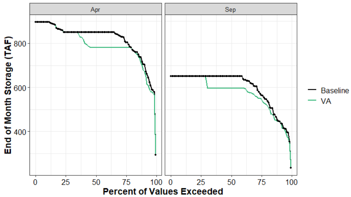
Figure 13.4-53. New Bullards Bar Reservoir End-of-April and End-of-September Carryover Storage under the Baseline and VA Scenarios
