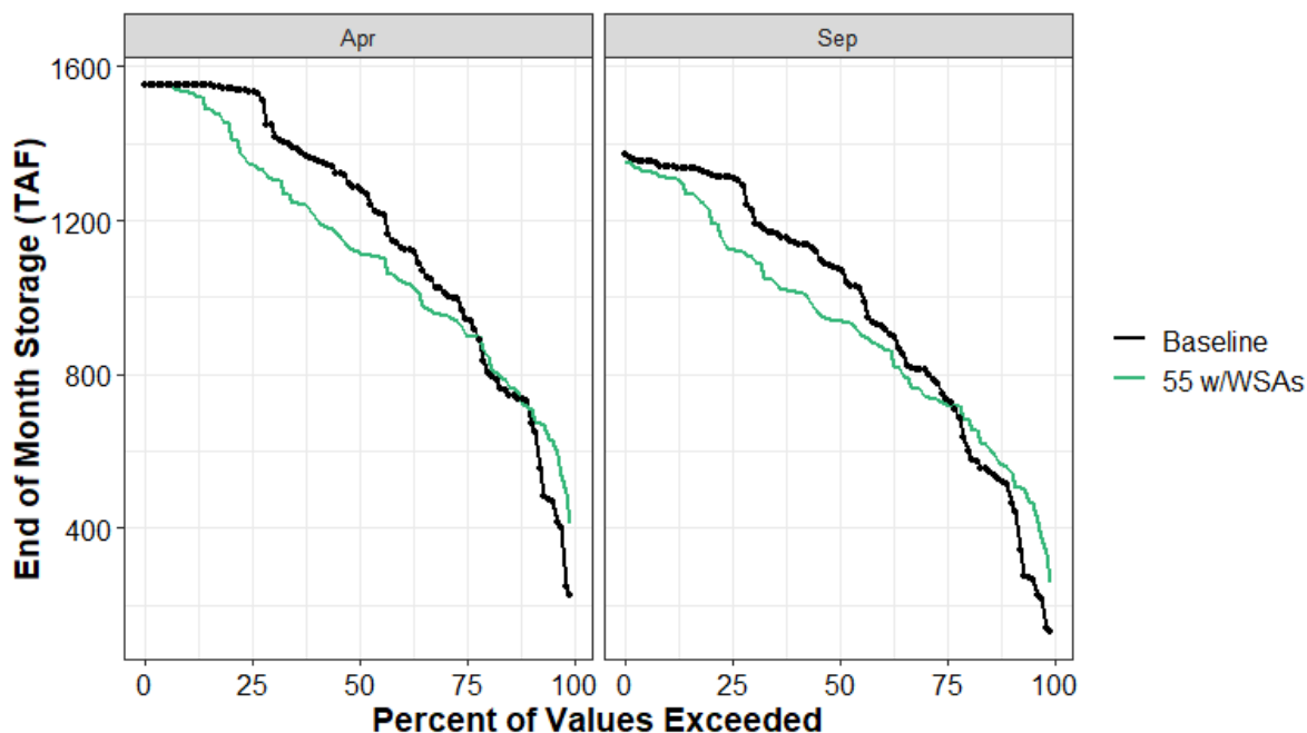
Figure 13.4-43. Lake Berryessa End-of-April and End-of-September Carryover Storage under the Baseline and 55 w/WSAs Scenarios
