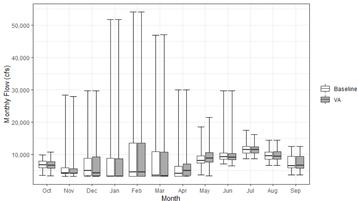
Figure 13.4-7. Monthly Streamflow for the Sacramento River below Keswick Reservoir under the Baseline and VA Scenarios
