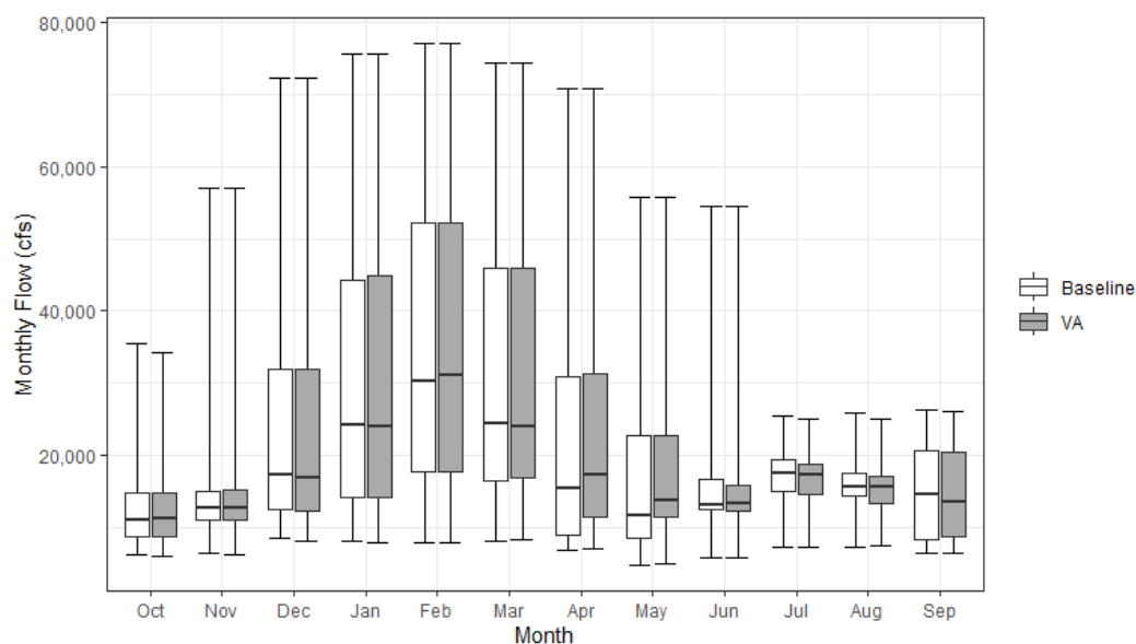
Figure 13.4-8. Monthly Streamflow for the Sacramento River at Freeport under the Baseline and VA Scenarios
