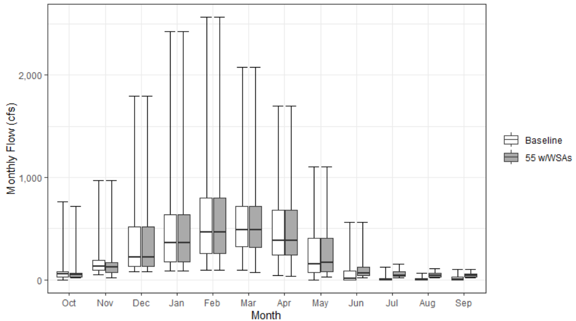
Figure 13.4-20. Monthly Streamflow for Deer Creek under the Baseline and 55 w/WSAs Scenarios
