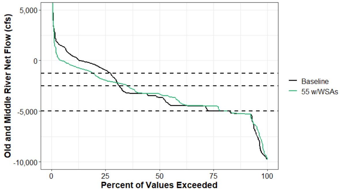
Figure 13.4-32. Monthly Exceedance Frequency Distribution of Old and Middle River Net Flow (cfs) for December–June under the Baseline and 55 w/WSAs Scenarios
