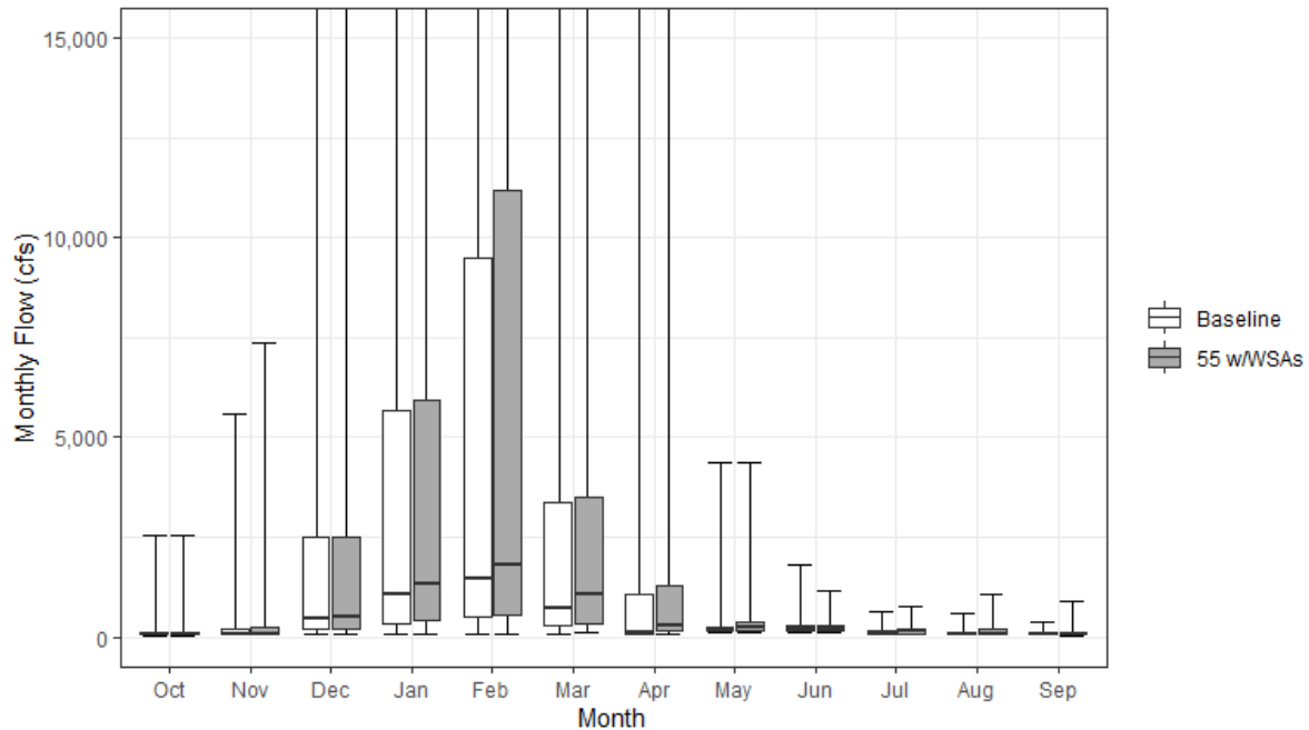
Figure 13.4-22. Monthly Streamflow for Yolo Bypass below Putah Creek Inflow under the Baseline and 55 w/WSAs Scenarios
