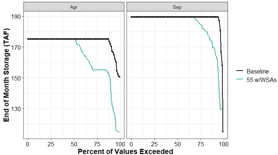
Figure 13.4-47. Pardee Reservoir End-of-April and End-of-September Carryover Storage under the Baseline and 55 w/WSAs Scenarios
