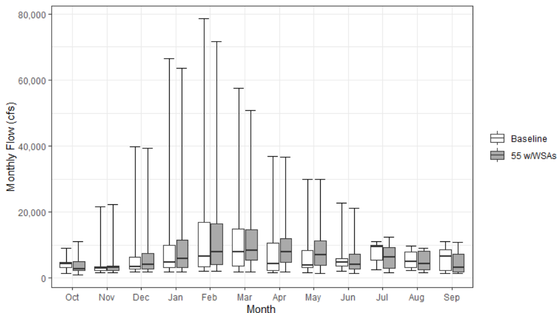
Figure 13.4-3. Monthly Streamflow for the Feather River above the Sacramento River under the Baseline and 55 w/WSAs Scenarios
