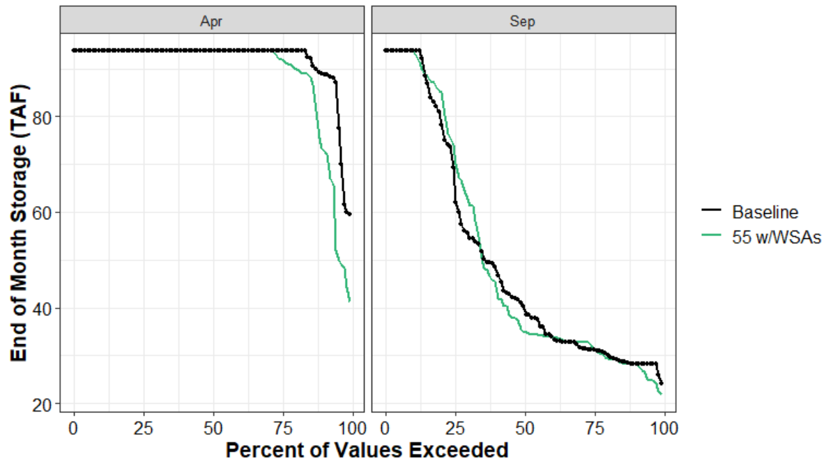
Figure 13.4-40. Camp Far West Reservoir End-of-April and End-of-September Carryover Storage under the Baseline and 55 w/WSAs Scenarios
