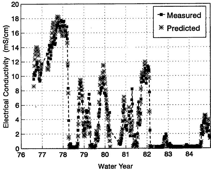
Figure 4.5. Measured and predicted 14-day average salinity at Chipps Island for the period, 1976-1985. The stars represent predictions using Denton's antecedent flow model. The squares joined by dashed lines represent field measured salinities.
