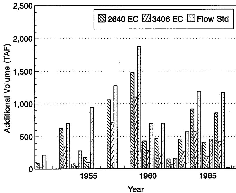
Figure 5.2.2.1. Additional outflow requirements of X2 standards for the period, 1951-1967, using Denton's antecedent flow-salinity relations based on: (i) EC=2640 \mu\text{S}/\text{cm} standard; (ii) EC=3406 \mu\text{S}/\text{cm} standard; (iii) equivalent flow standard.
