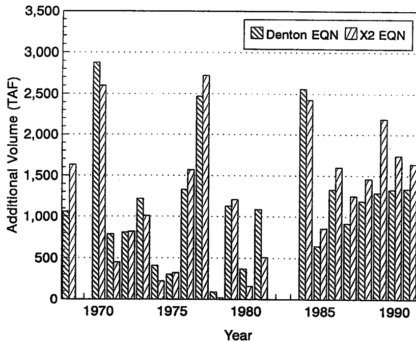
Figure 5.2.5.1. Additional outflow requirements of X2 standards for the period, 1968-1991, using: (i) Denton's antecedent flow-salinity relations; (ii) X2 equation. The X2 standard is implemented as an EC=2640 \mu S/cm standard in both cases.
