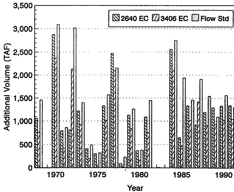
Figure 5.2.1.1. Additional outflow requirements of X2 standards for the period, 1968-1991, using Denton's antecedent flow-salinity relations based on: (i) EC=2640 \mu\text{S}/\text{cm} standard; (ii) EC=3406 \mu\text{S}/\text{cm} standard; (iii) equivalent flow standard.
