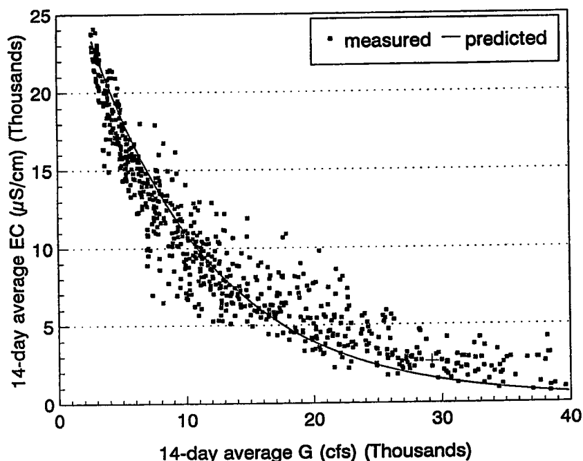
Figure 4.3. Predicted and measured 14-day average salinity at Port Chicago. The solid line is the salinity predicted using Denton's antecedent flow relations and overall "best-fit" parameters from table 4.1. The cross indicates the model prediction at EC=2640 \mu\text{S}/\text{cm} using local "best-fit" parameters in the vicinity of EC=2640 \mu\text{S}/\text{cm} .
