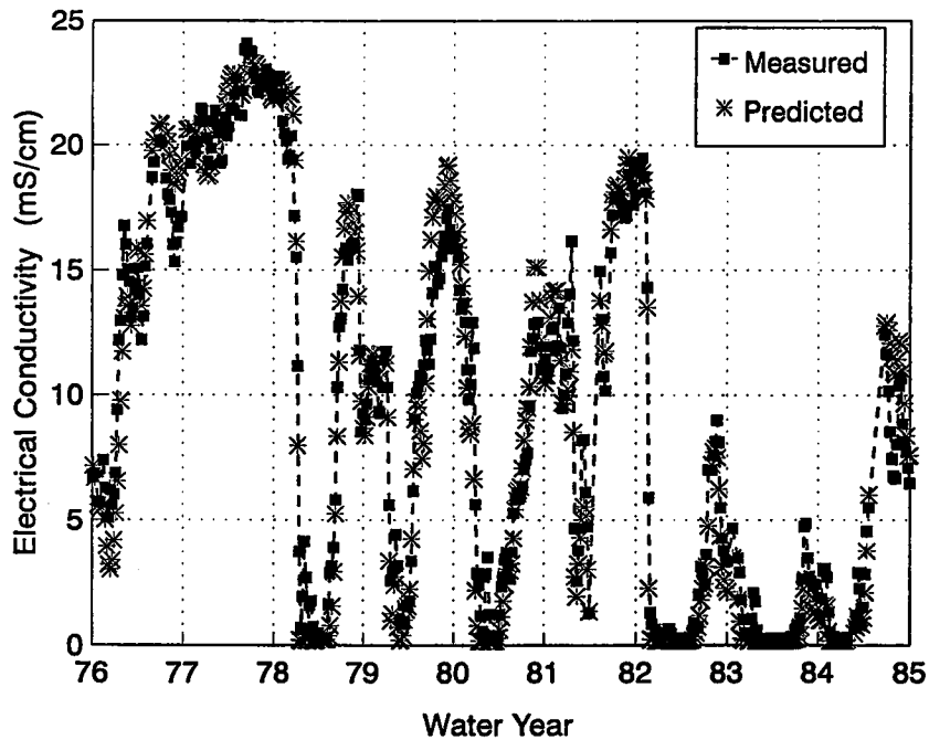
Figure 4.5. Measured and predicted 14-day average salinity at Chipps Island for the period, 1976-1985. The stars represent predictions using Denton's antecedent flow model. The squares joined by dashed lines represent field measured salinities.
