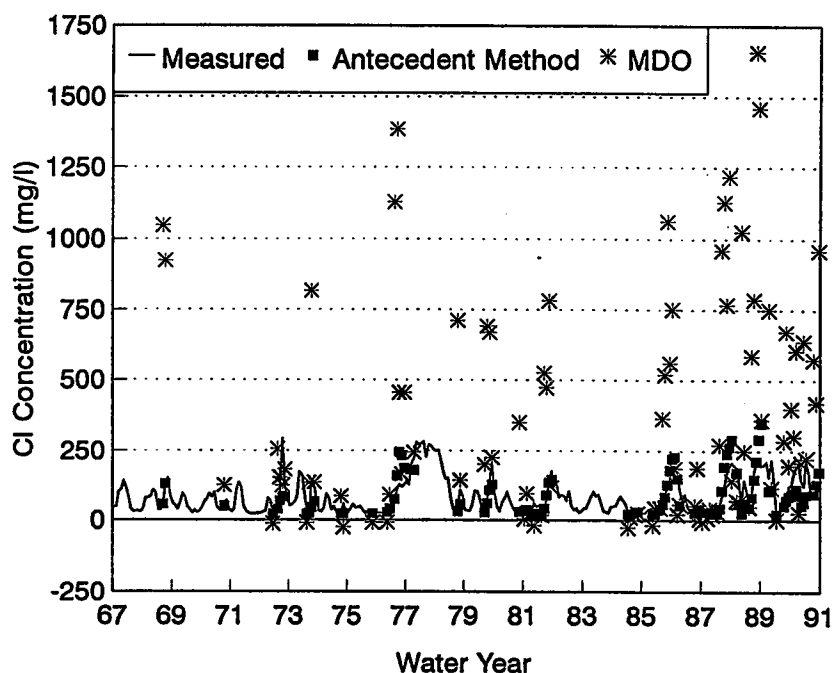
Figure 3.1. Measured and predicted monthly-averaged salinity at Rock Slough. Predictions are based on: (1) Denton's antecedent flow method; and (2) steady-state relations from the "carriage water" model, MDO, used in DWRSIM.
