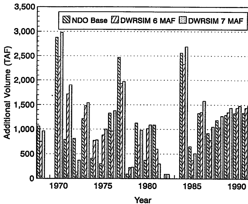
Figure 5.2.4.1. Additional outflow requirements of X2 standards for the period, 1968-1991, using Denton's antecedent flow-salinity relations based on: (i) NDO historical base case; (ii) DWRSIM base case. X2 standard is implemented as EC=2640 \mu S/cm standard in both cases.
