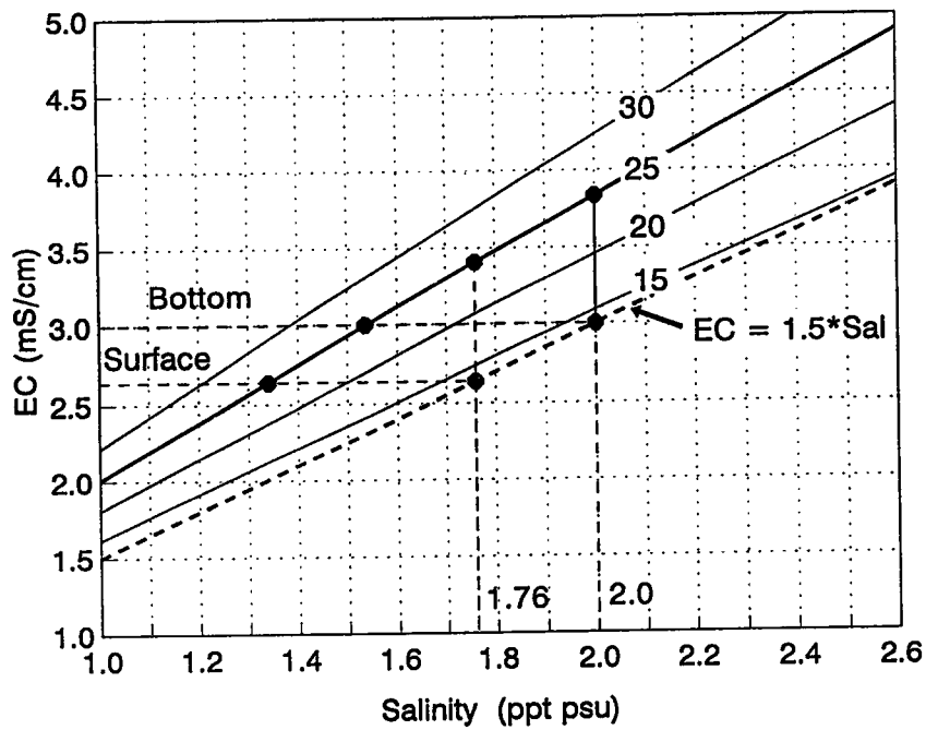
Figure 2.1.1. Conversion from electrical conductivity (EC) to practical salinity using the Accerboni-Mosetti equation. The conversions are shown for four temperatures: 15, 20, 25, and 30 °C.
