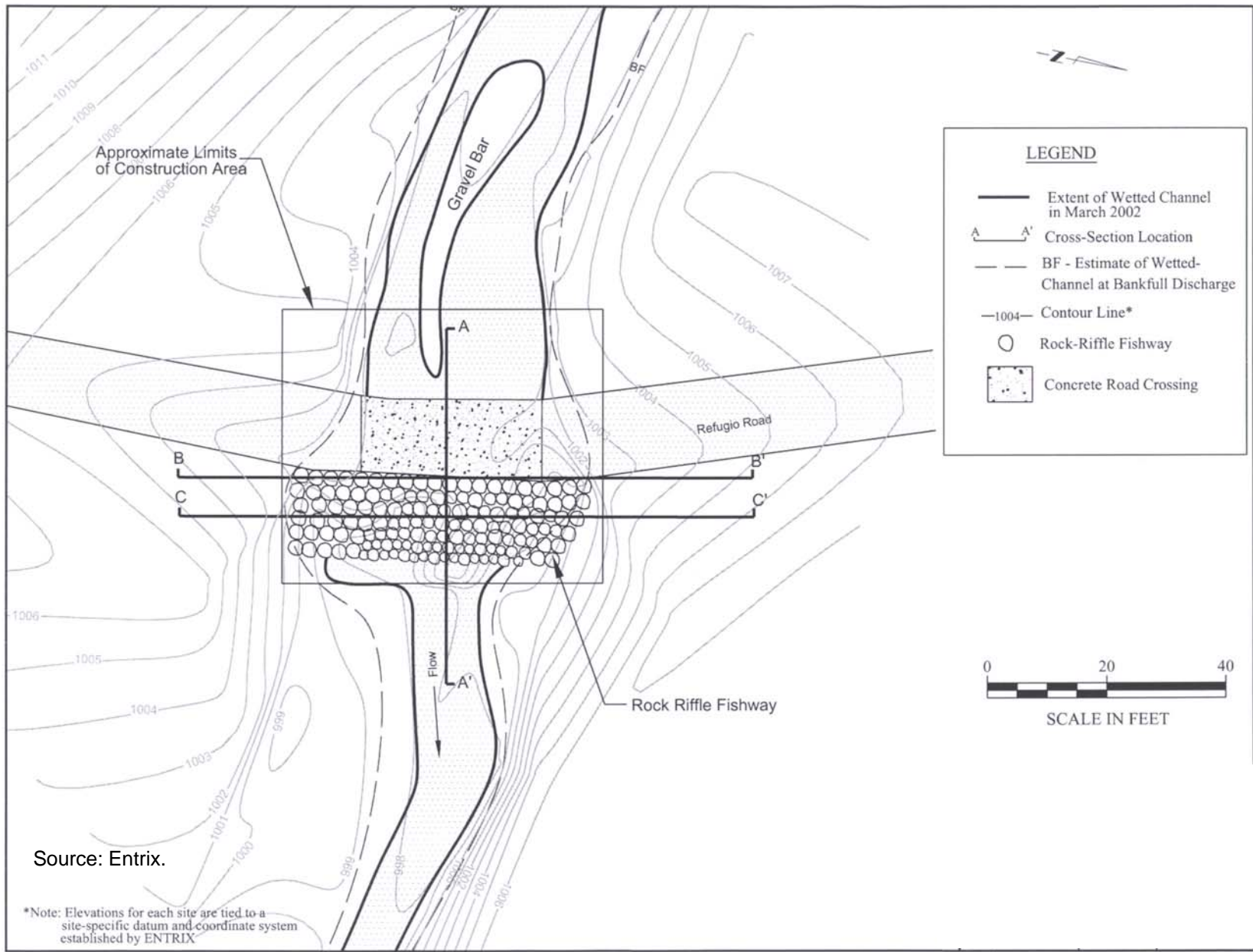
Figure 2-11. Proposed Fishway at Quiota Creek Crossing No. 3
