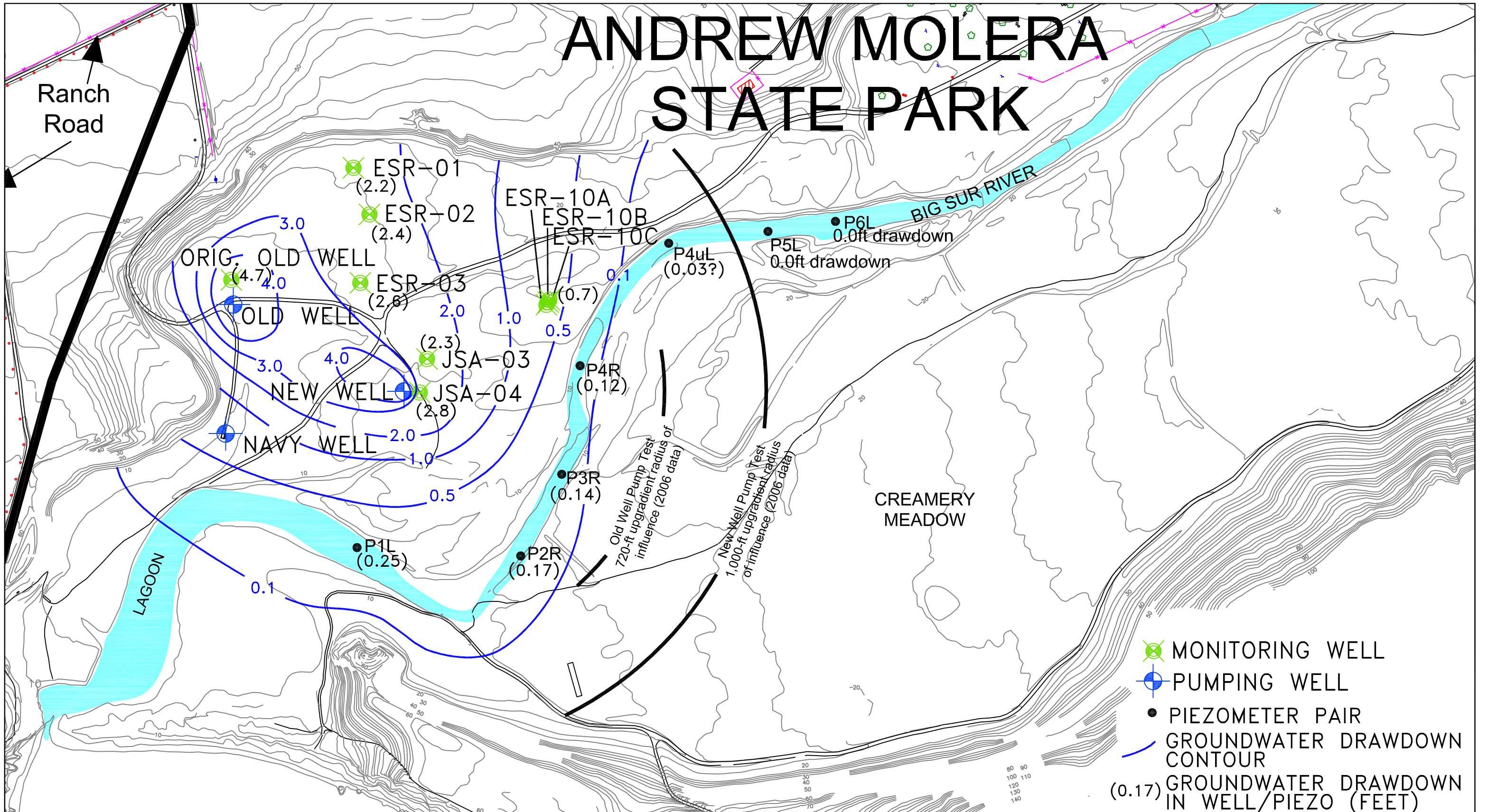
FIGURE 3-1 IRRIGATION WELL RADIUS OF INFLUENCE AND CONCEPTUAL GROUNDWATER DRAWDOWN MAP (2007 MAXIMUM PUMPING CONDITIONS DEPICTED)
