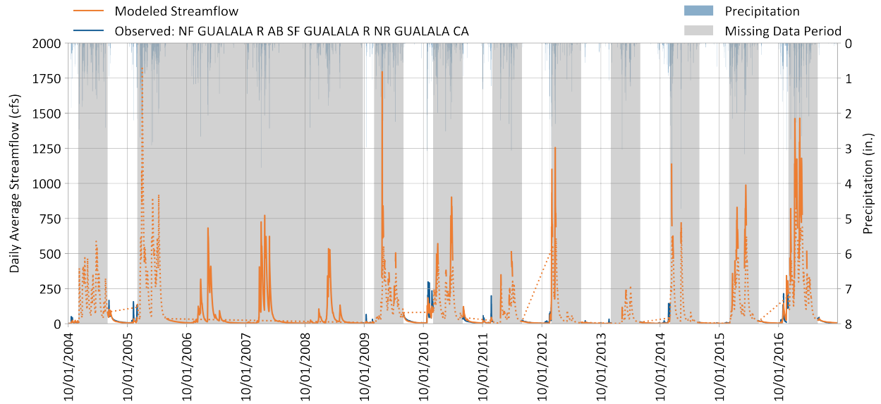
Figure 7-16. Daily simulated vs. observed streamflow for Gualala River North Fork near Gualala.
