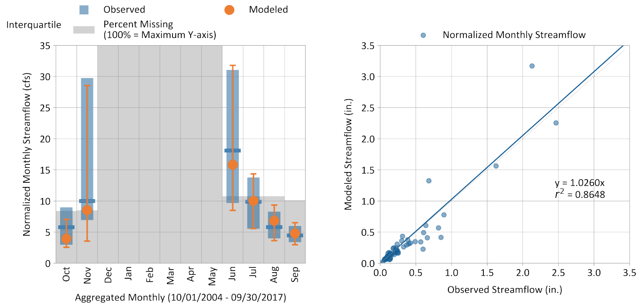
Figure 7-18. Monthly simulated vs. observed streamflow for Gualala River North Fork near Gualala.
