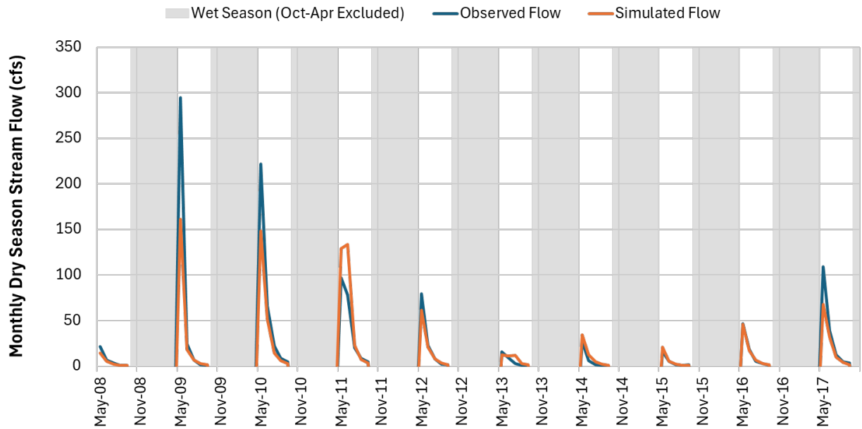
Figure 7-10. Hydrograph of dry season flow during validation period at Gualala River South Fork at Sea Ranch.
