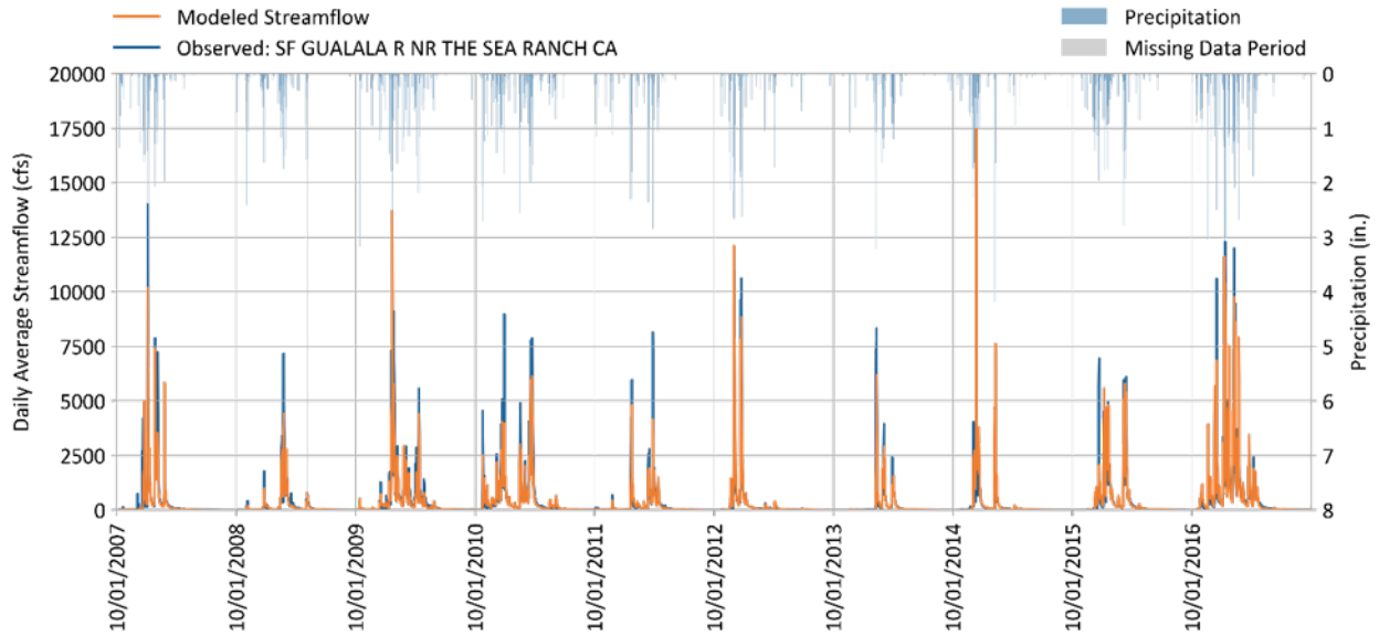
Figure 7-8. Daily simulated vs. observed streamflow for Gualala River South Fork at Sea Ranch.
