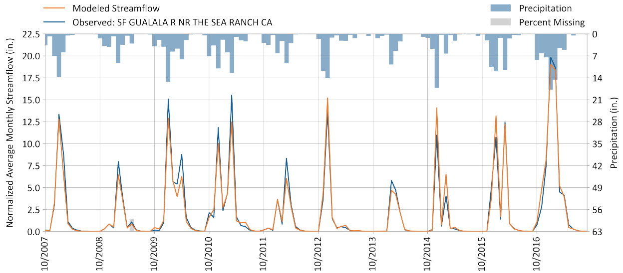
Figure 7-9. Monthly simulated vs. observed streamflow for Gualala River South Fork at Sea Ranch.
