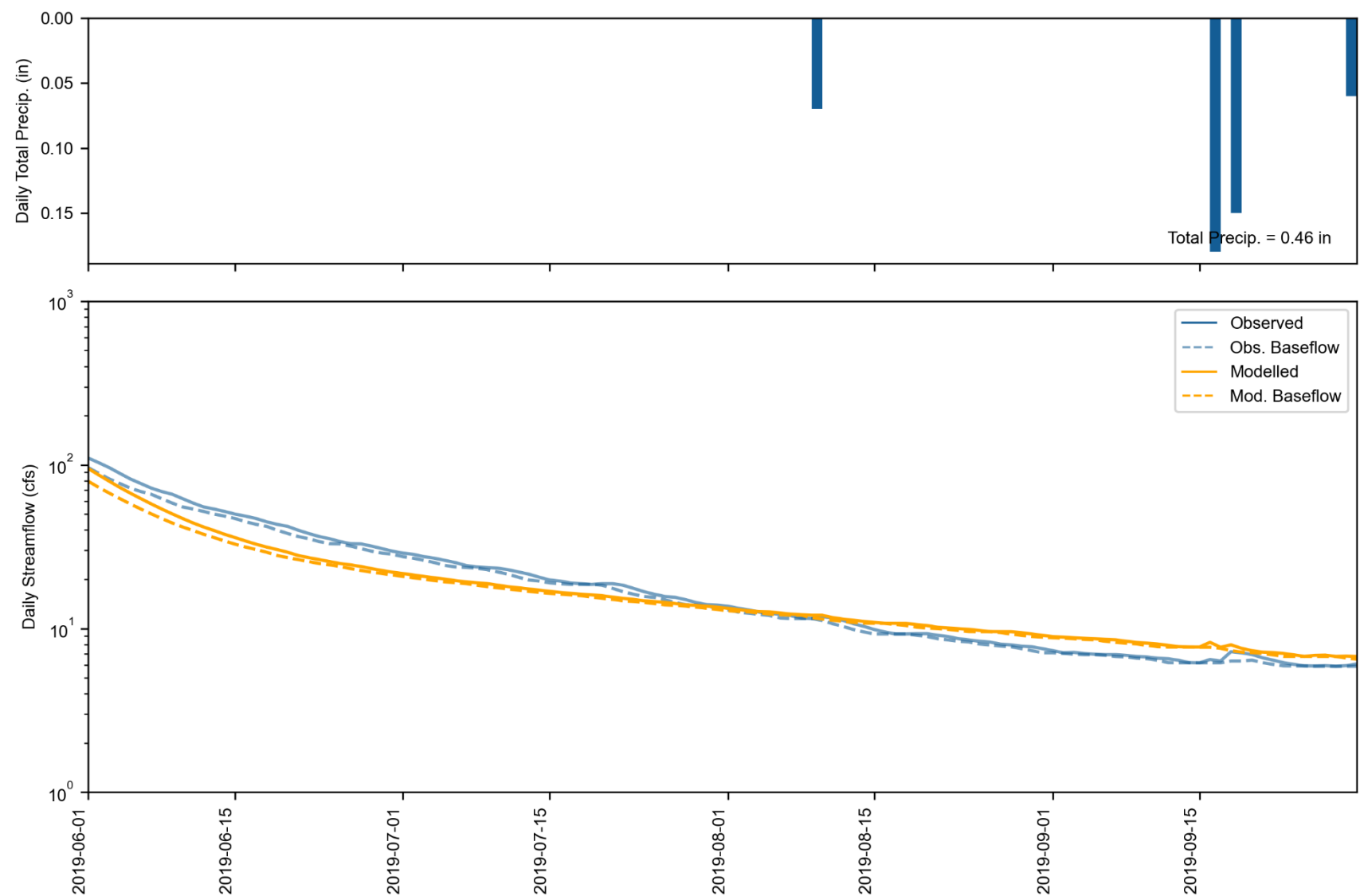
Figure 6-23. Water Year 2019 Dry season daily total precipitation (top) and streamflow (bottom) at Gualala River North Fork near Gualala. Observed and simulated baseflow are calculated with HYSEP.
