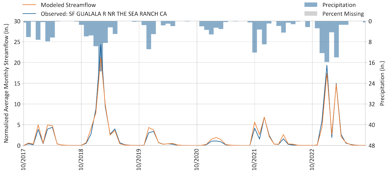
Figure 6-9. Monthly simulated vs. observed streamflow for Gualala River South Fork at Sea Ranch.
