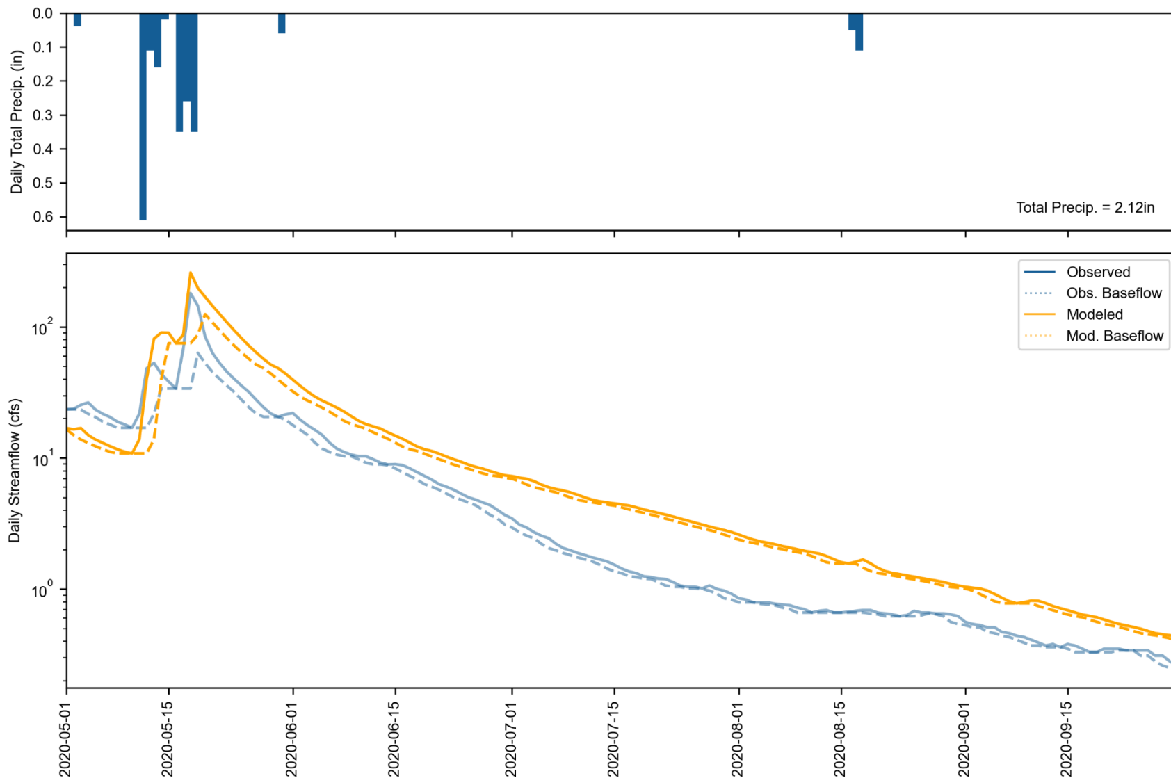
Figure 6-16. Water Year 2020 Dry season daily total precipitation (top) and streamflow (bottom) at Gualala River South Fork at Sea Ranch. Observed and simulated baseflow are calculated with HYSEP.
