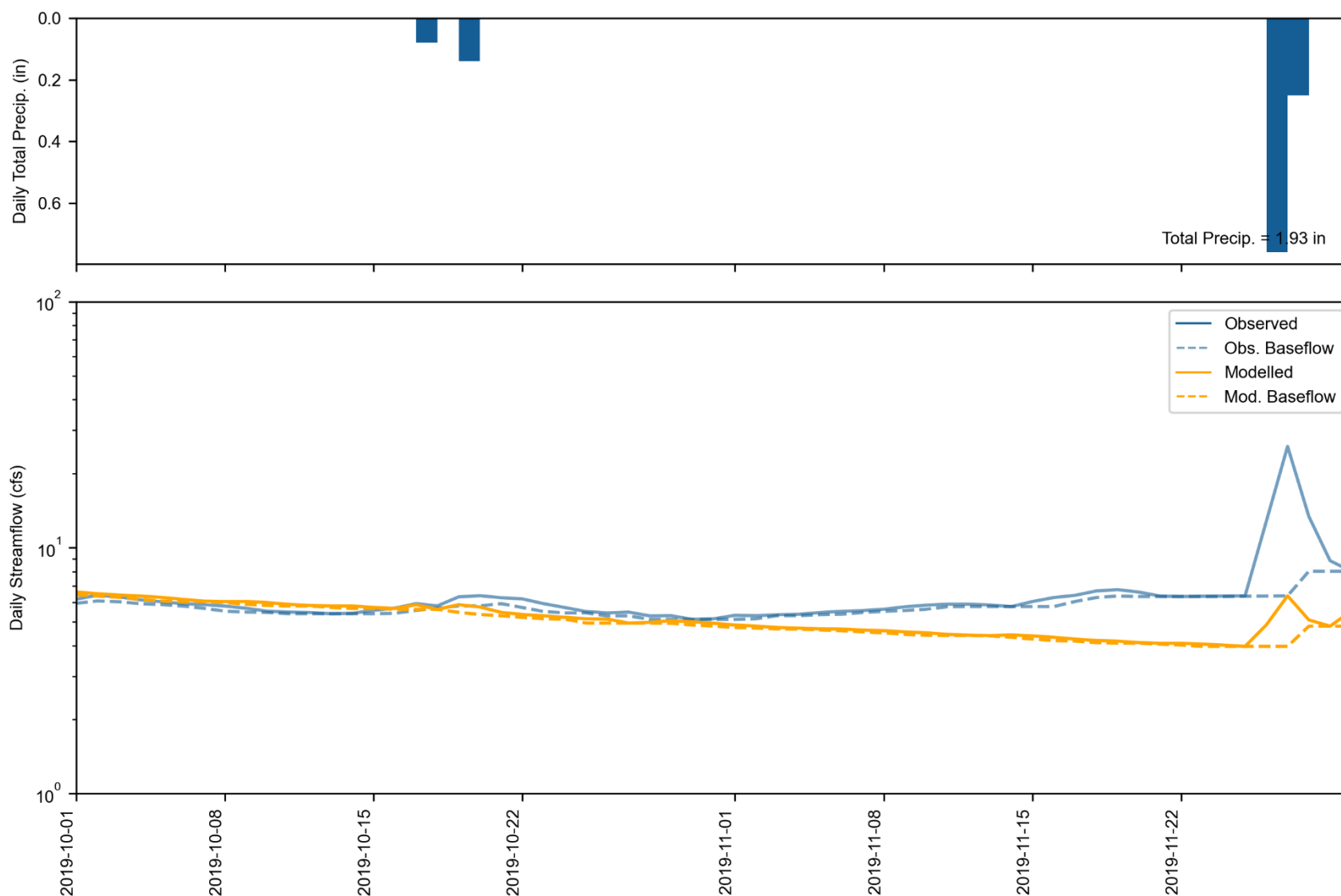
Figure 6-24. Water Year 2020 Wet season daily total precipitation (top) and streamflow (bottom) at Gualala River North Fork near Gualala. Observed and simulated baseflow are calculated with HYSEP.
