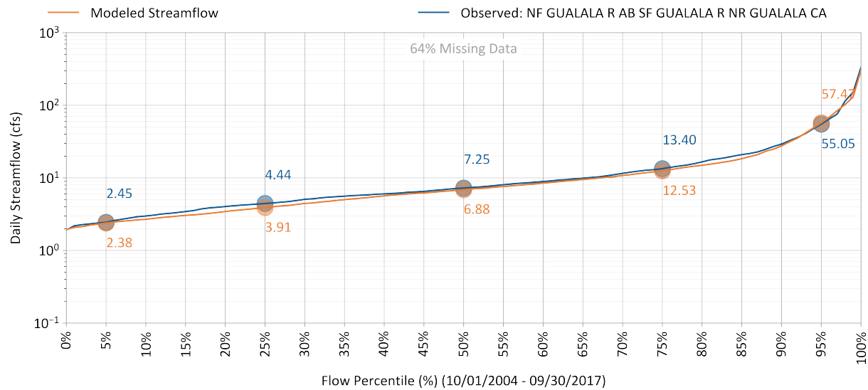
Figure 7-20. Simulated vs. observed flow duration curve for Gualala River North Fork near Gualala.
