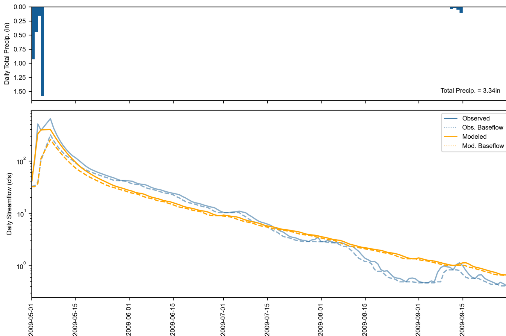
Figure 7-15. Water Year 2009 Dry season daily total precipitation (top) and streamflow (bottom) at Gualala River South Fork at Sea Ranch. Observed and simulated baseflow are calculated with HYSEP.
