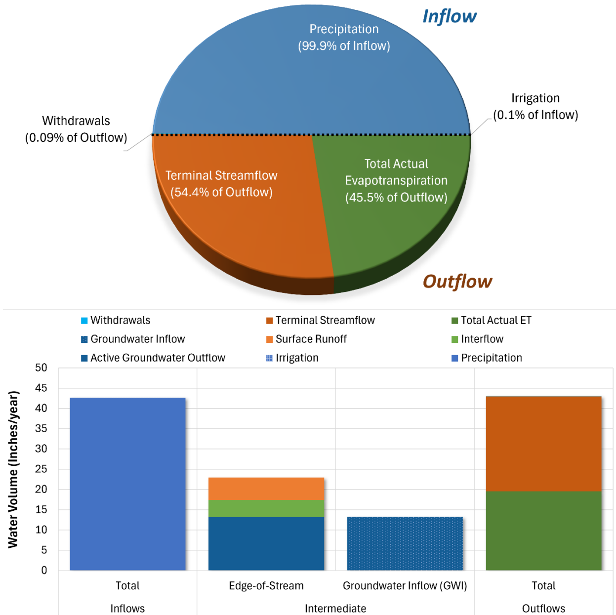
Figure 7-1. Simulated water balance expressed as total volumes and area-normalized annual average depths for the calibration period (water years 2018-2023) across the Gualala River watershed.
