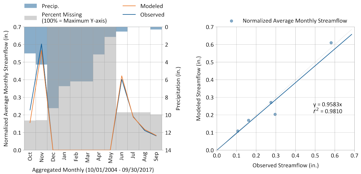
Figure 7-19. Average monthly simulated vs. observed streamflow for Gualala River North Fork near Gualala.
