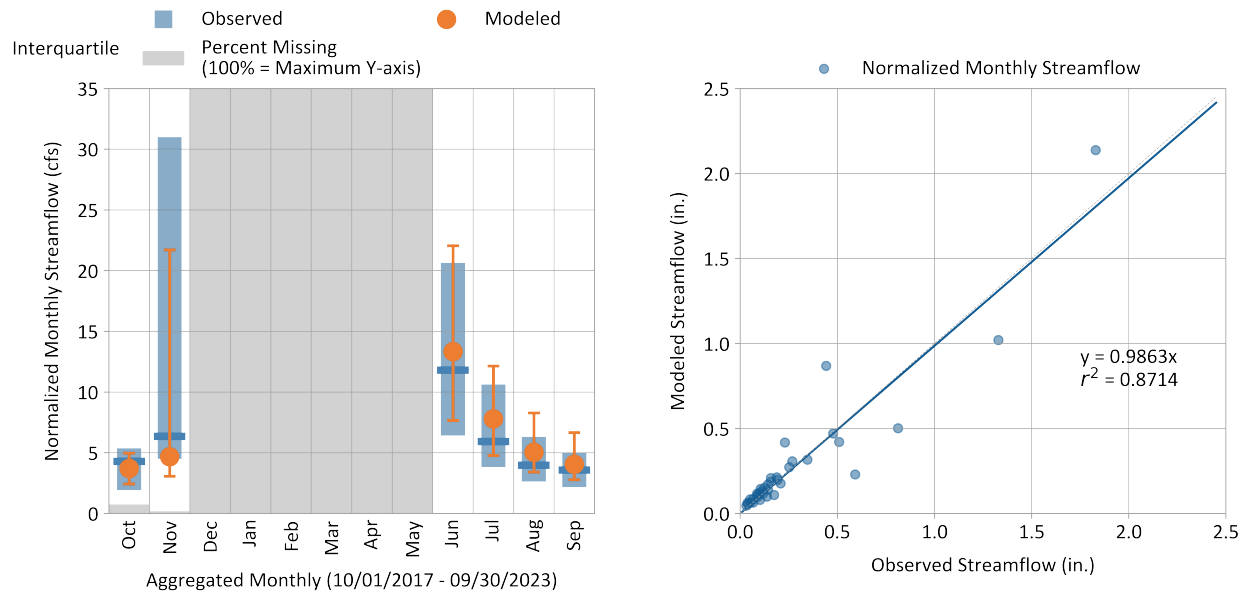
Figure 6-19. Monthly simulated vs. observed streamflow for Gualala River North Fork near Gualala.
