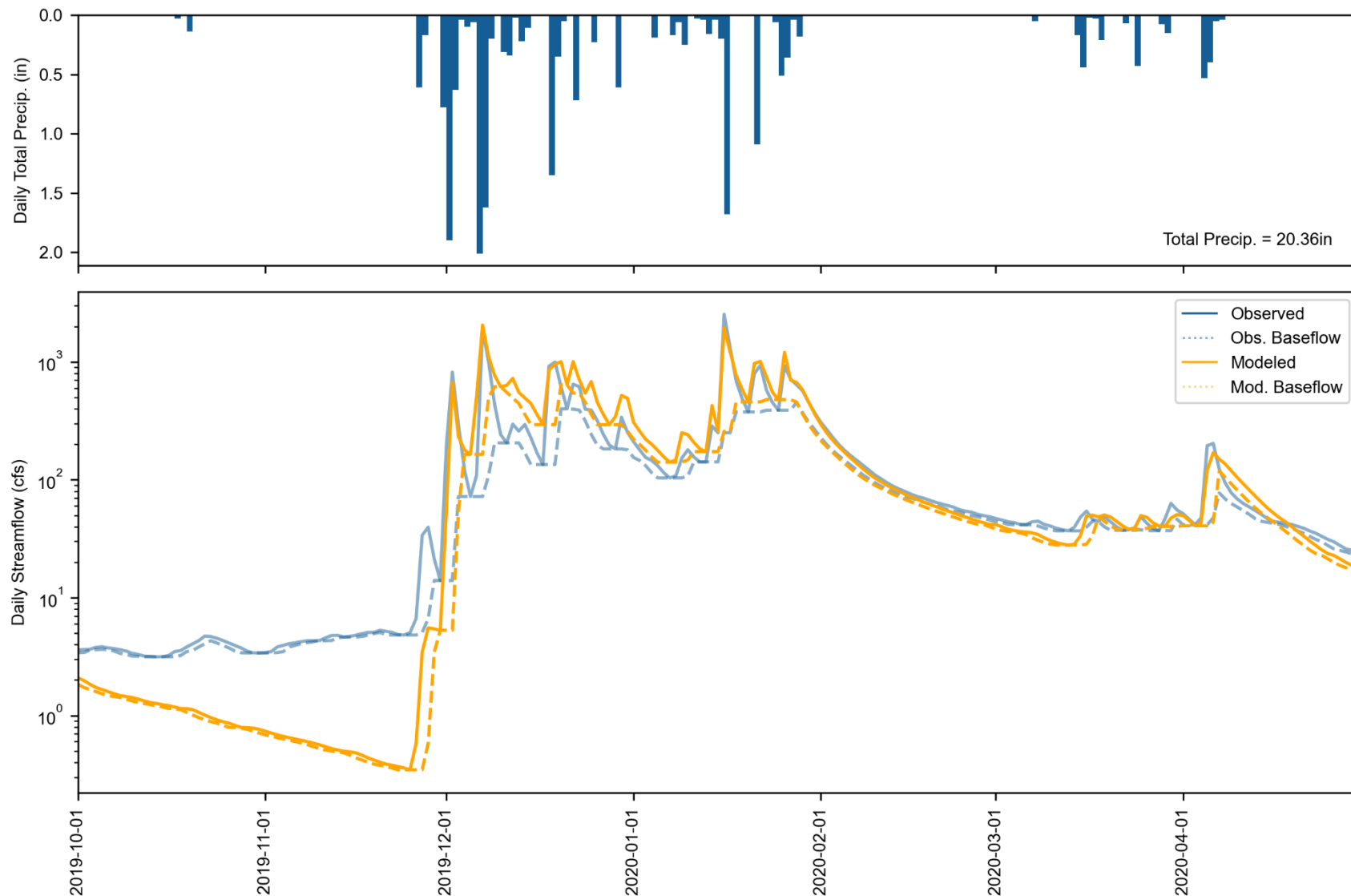
Figure 6-15. Water Year 2020 Wet season daily total precipitation (top) and streamflow (bottom) at Gualala River South Fork at Sea Ranch. Observed and simulated baseflow are calculated with HYSEP.
