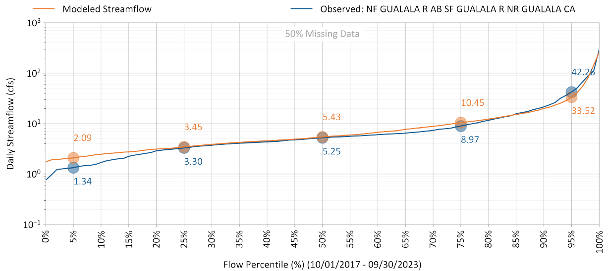
Figure 6-21. Simulated vs. observed flow duration curve for Gualala River North Fork near Gualala.
