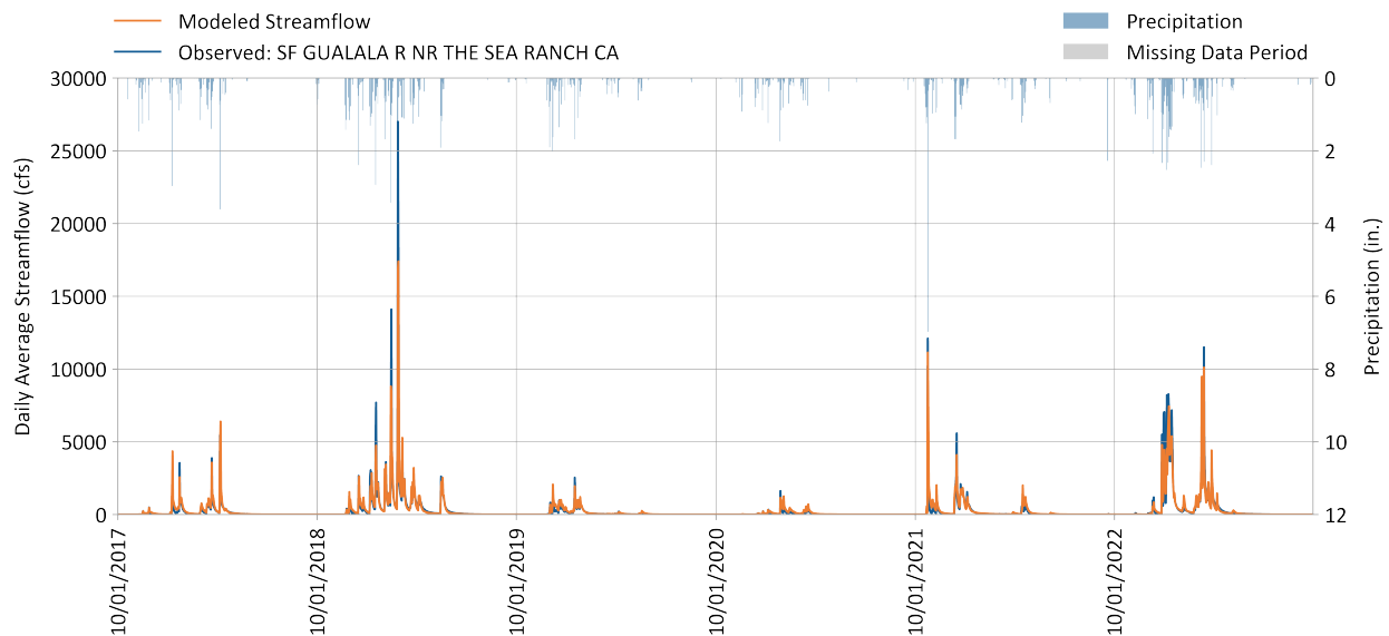
Figure 6-8. Daily simulated vs. observed streamflow for Gualala River South Fork at Sea Ranch.
