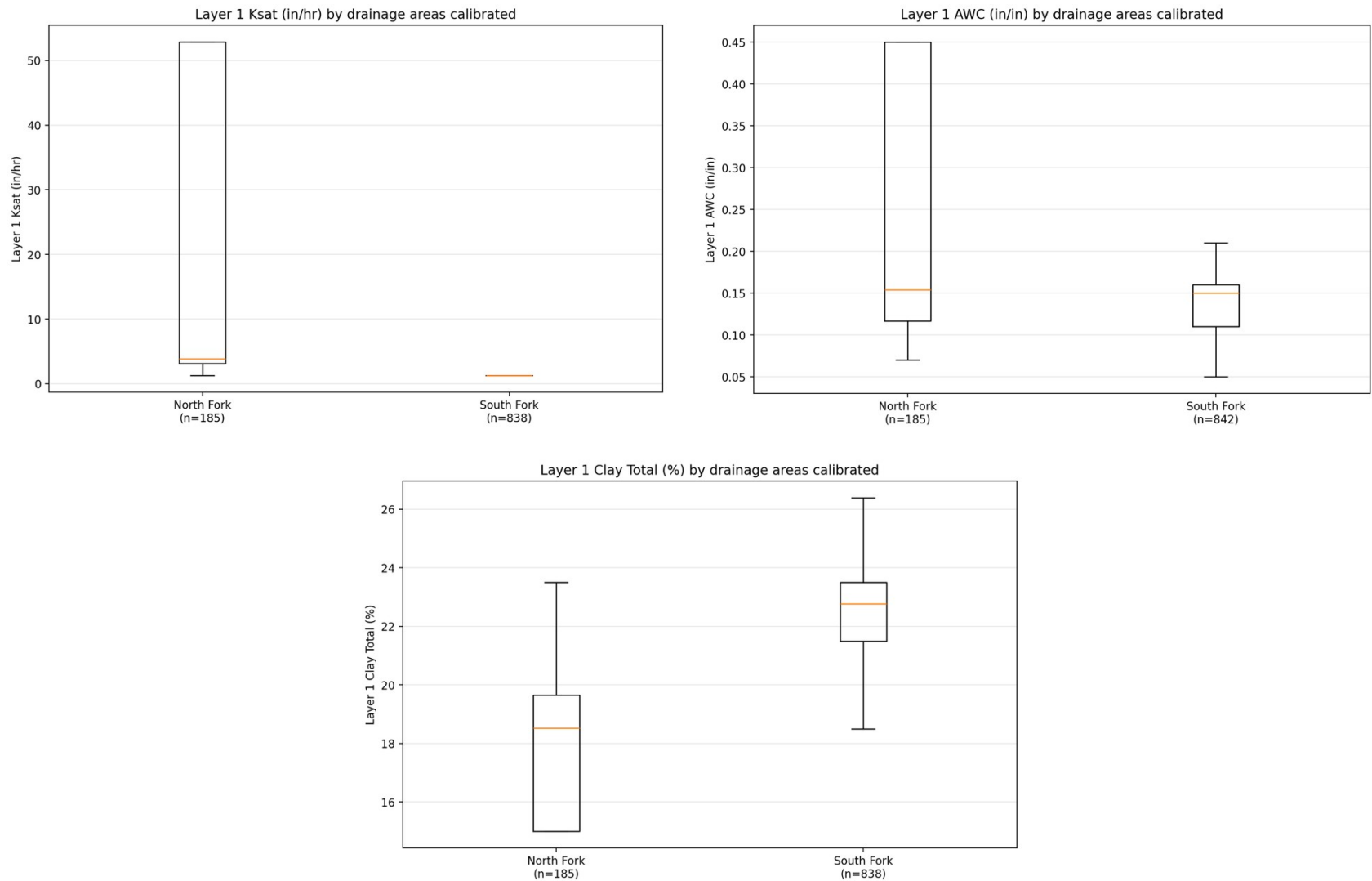
Figure 6-5. Boxplots comparing SSURGO Layer 1 saturated hydraulic conductivity (Ksat), available water content (AWC), and clay percentage between the North Fork and South Fork drainage areas (“n” denotes the number of SSURGO MUPOLYGONS within each boundary).
