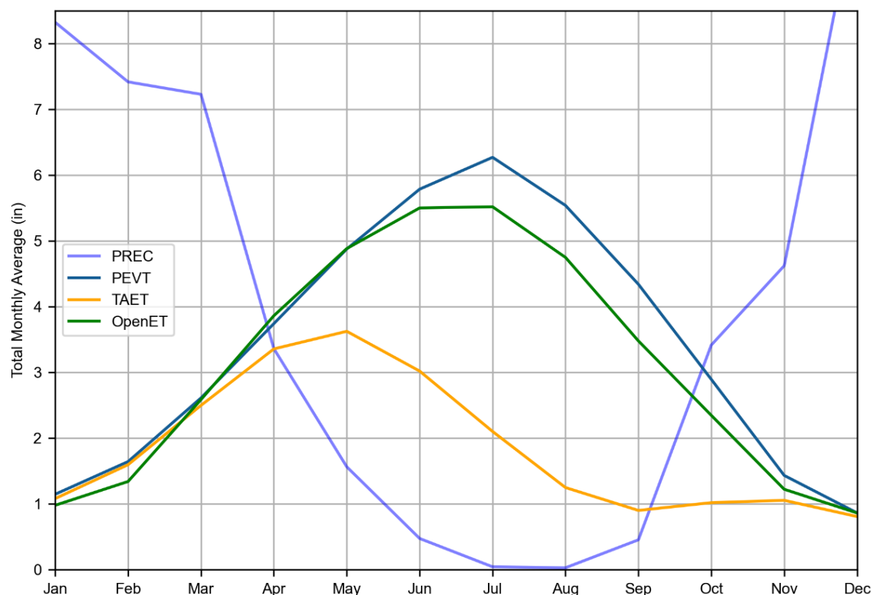
Figure 7-4. Comparison of average monthly totals from October 2003 – September 2023 for rainfall (PREC), potential ET (PET), and simulated total actual ET (TAET) for the Gualala River watershed.
