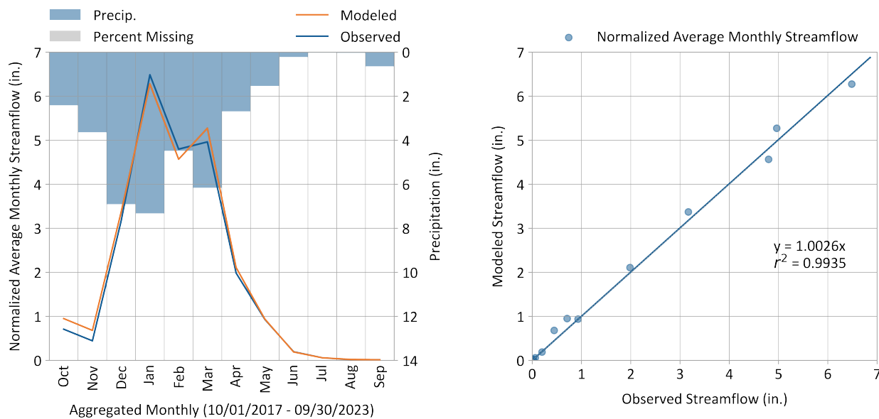
Figure 6-11. Average Monthly simulated vs. observed streamflow for Gualala River South Fork at Sea Ranch.
