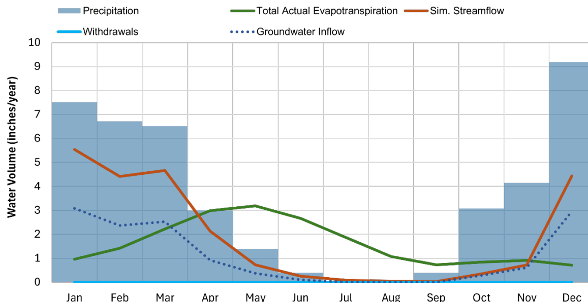
Figure 7-2. Monthly average area-normalized simulated water balance components for water years 2018-2023 across the Gualala River watershed. Note that withdrawals are a minor portion of the total water balance.
