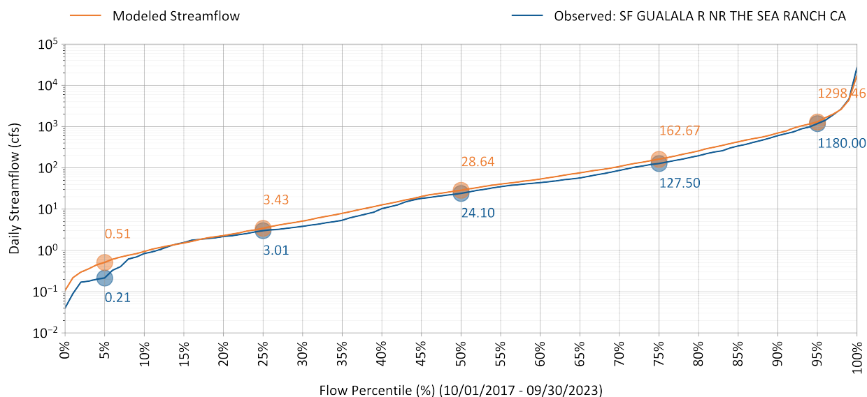
Figure 6-12. Simulated vs. observed flow duration curve for Gualala River South Fork at Sea Ranch.
