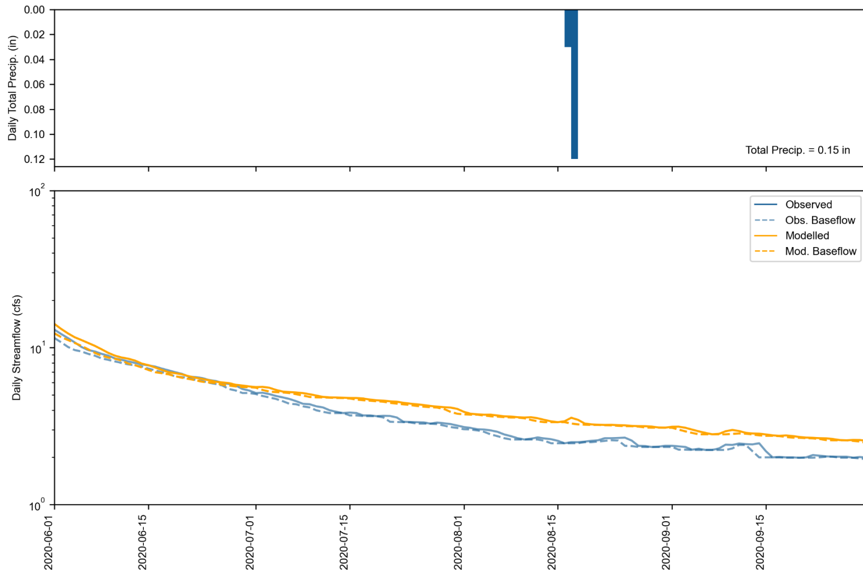
Figure 6-25. Water Year 2020 Dry season daily total precipitation (top) and streamflow (bottom) at Gualala River North Fork near Gualala. Observed and simulated baseflow are calculated with HYSEP.
