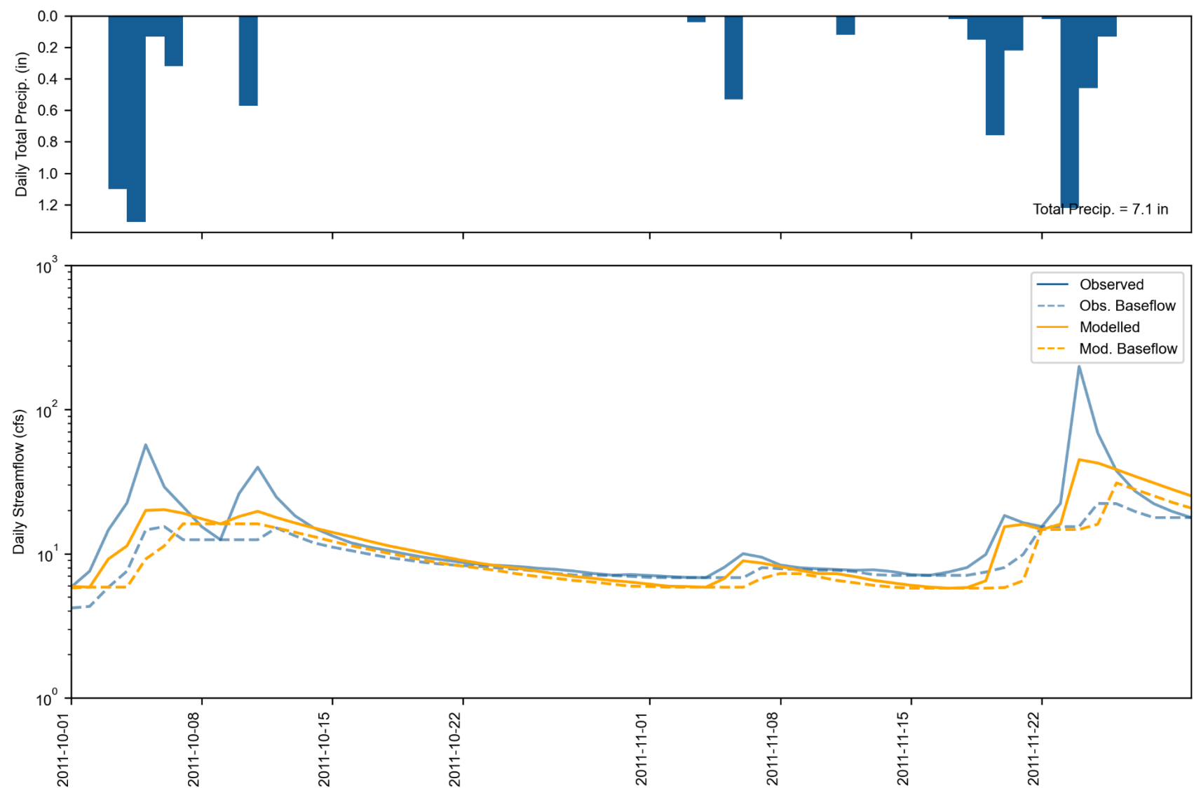
Figure 7-21. Water Year 2012 Wet season daily total precipitation (top) and streamflow (bottom) at Gualala River North Fork near Gualala. Observed and simulated baseflow are calculated with HYSEP.
