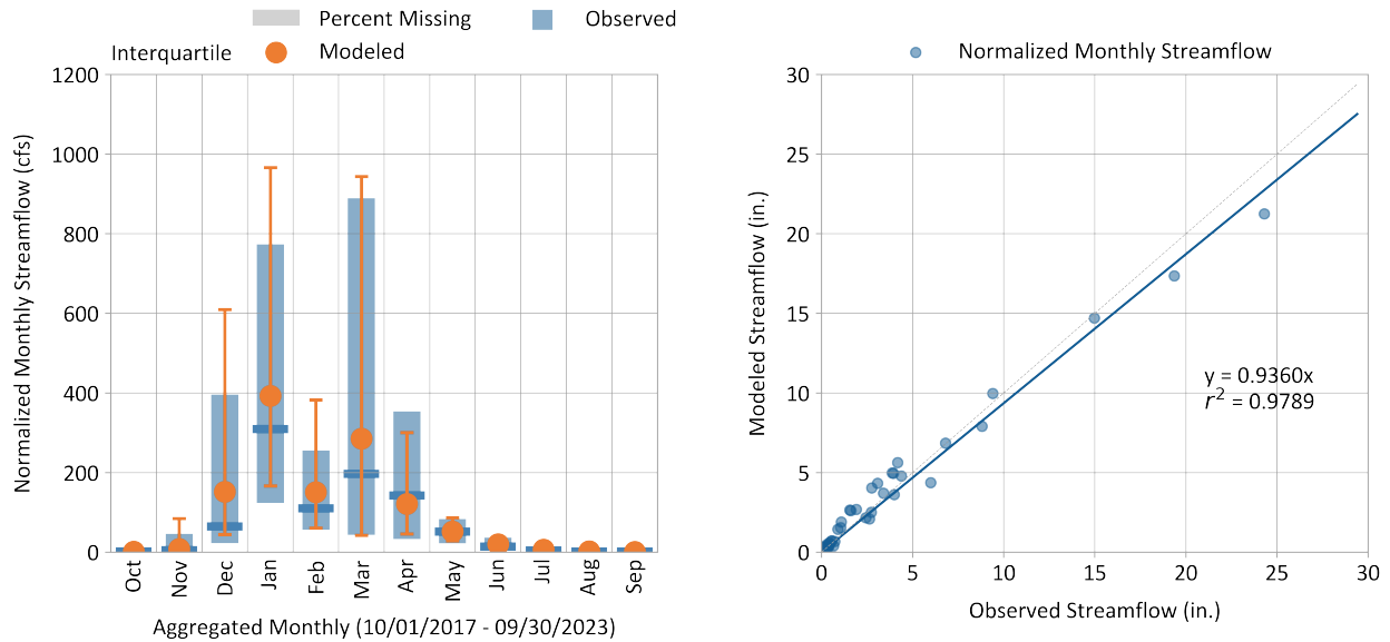
Figure 6-10. Monthly simulated vs. observed streamflow for Gualala River South Fork at Sea Ranch.
