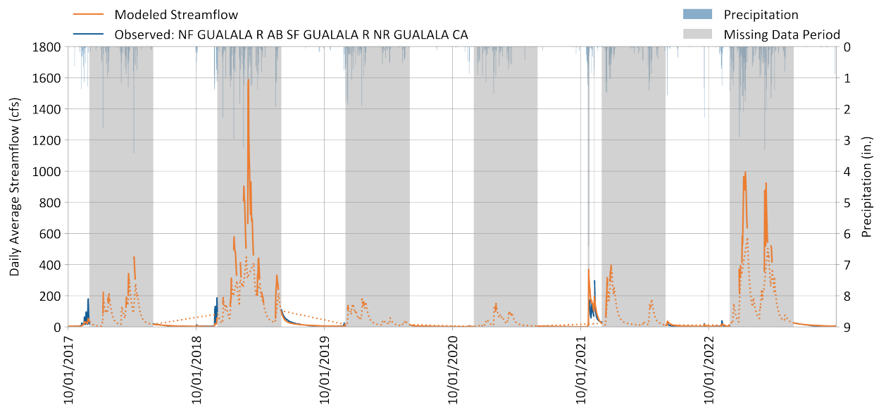
Figure 6-17. Daily simulated vs. observed streamflow for Gualala River North Fork near Gualala.
