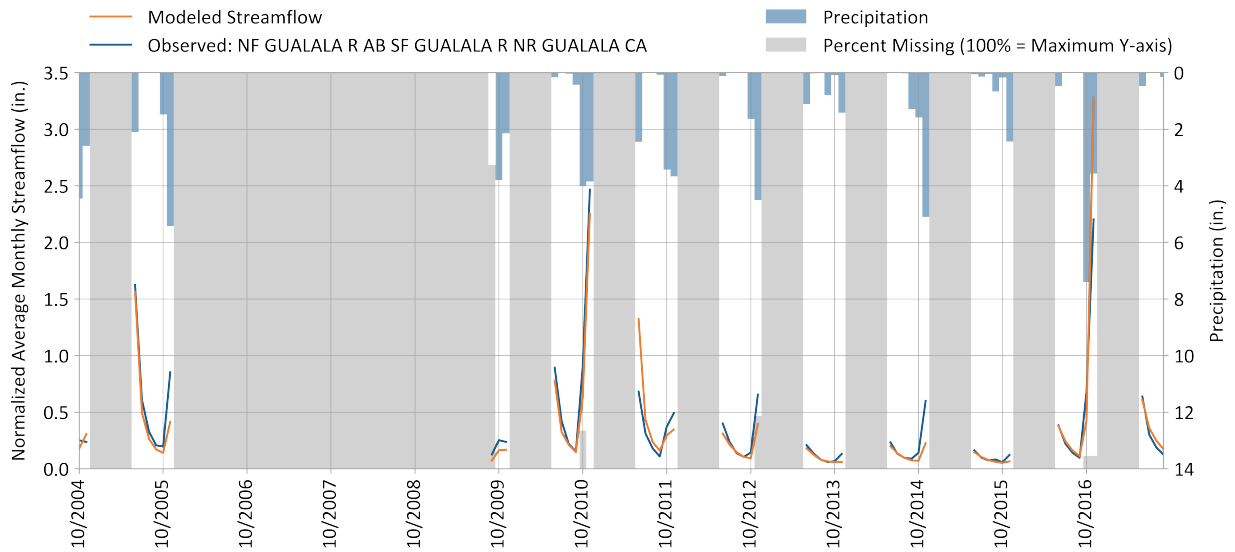
Figure 7-17. Monthly simulated vs. observed streamflow for Gualala River North Fork near Gualala.
