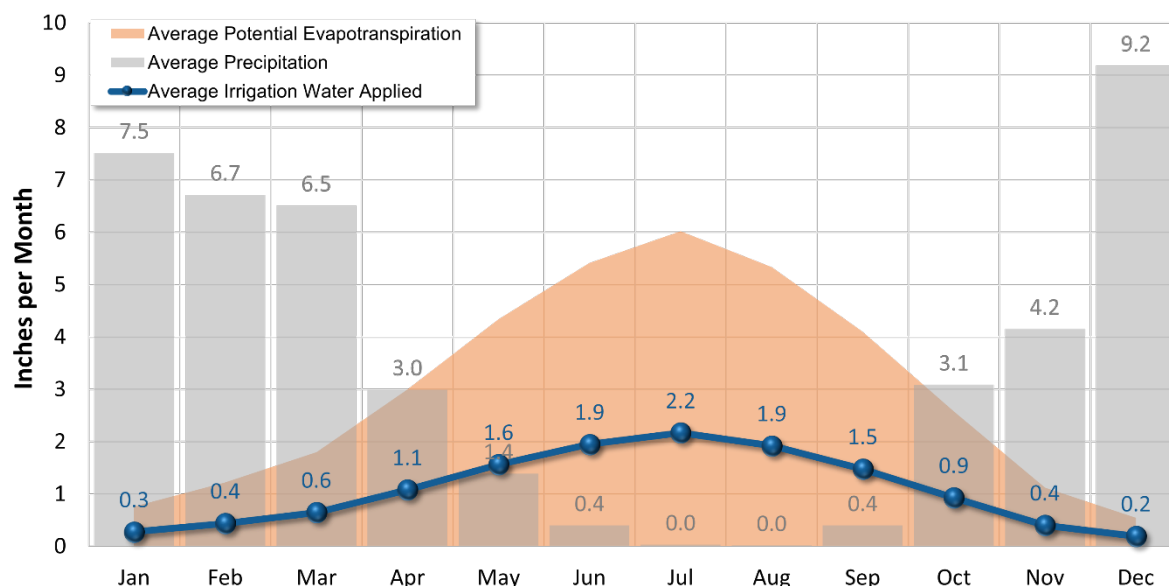
Figure 7-3. Monthly average area-normalized irrigation water balance for irrigated HRUs in the Gualala River watershed.
