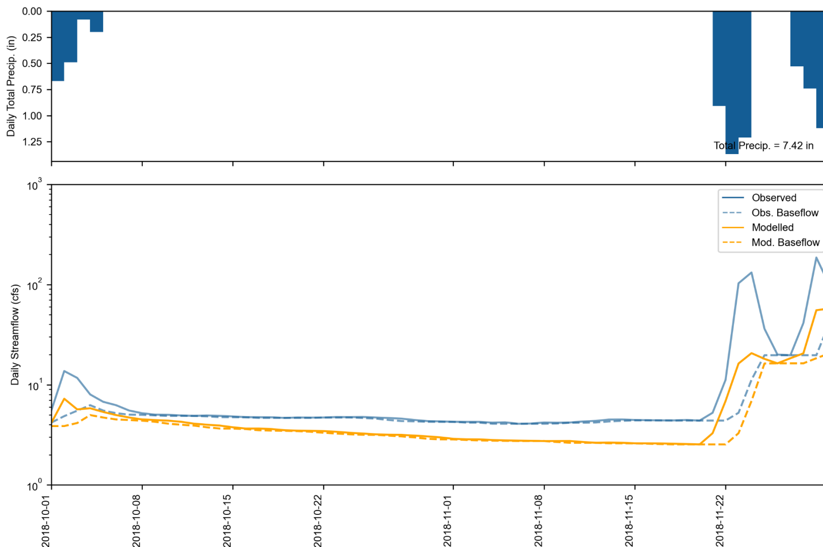
Figure 6-22. Water Year 2019 Wet season daily total precipitation (top) and streamflow (bottom) at Gualala River North Fork near Gualala. Observed and simulated baseflow are calculated with HYSEP.
