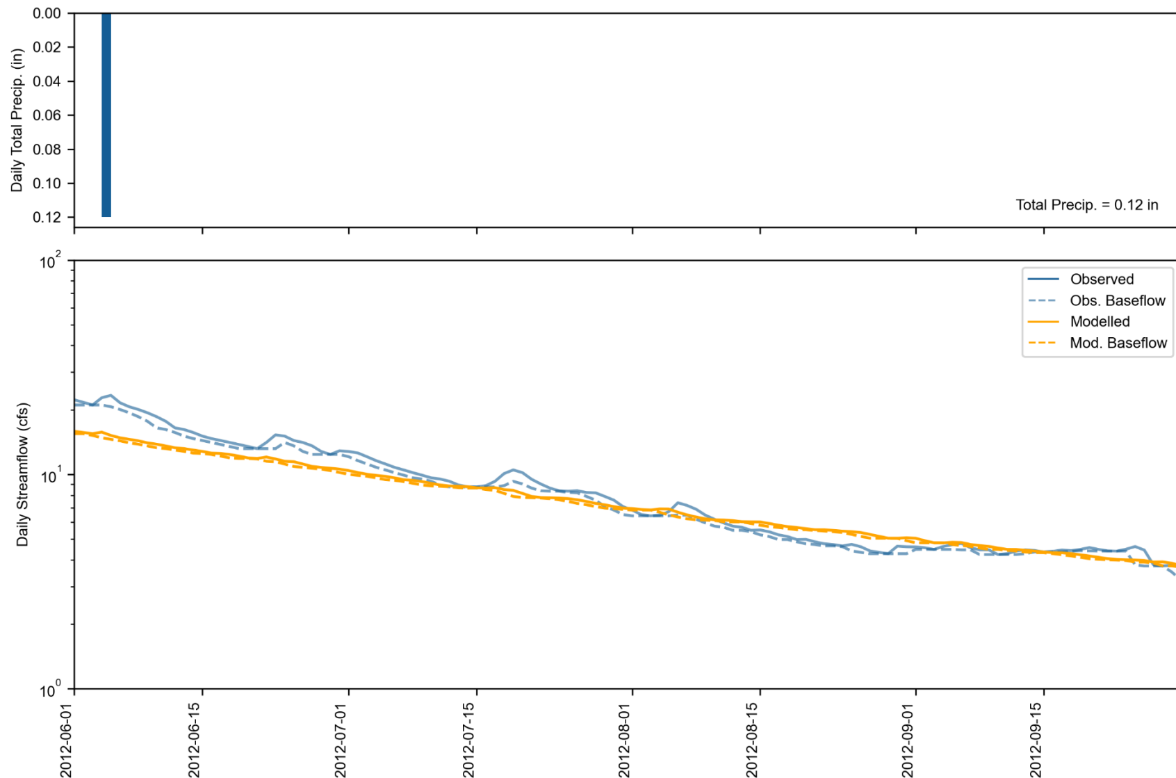
Figure 7-22. Water Year 2012 Dry season daily total precipitation (top) and streamflow (bottom) at Gualala River North Fork near Gualala. Observed and simulated baseflow are calculated with HYSEP.
