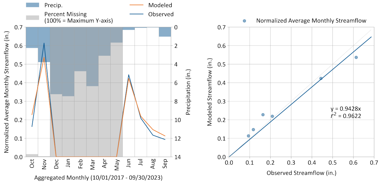
Figure 6-20. Average Monthly simulated vs. observed streamflow for Gualala River North Fork near Gualala.
