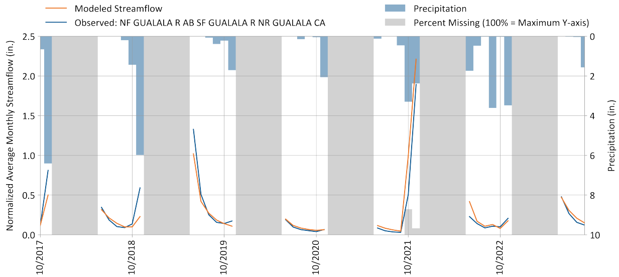
Figure 6-18. Monthly simulated vs. observed streamflow for Gualala River North Fork near Gualala.
