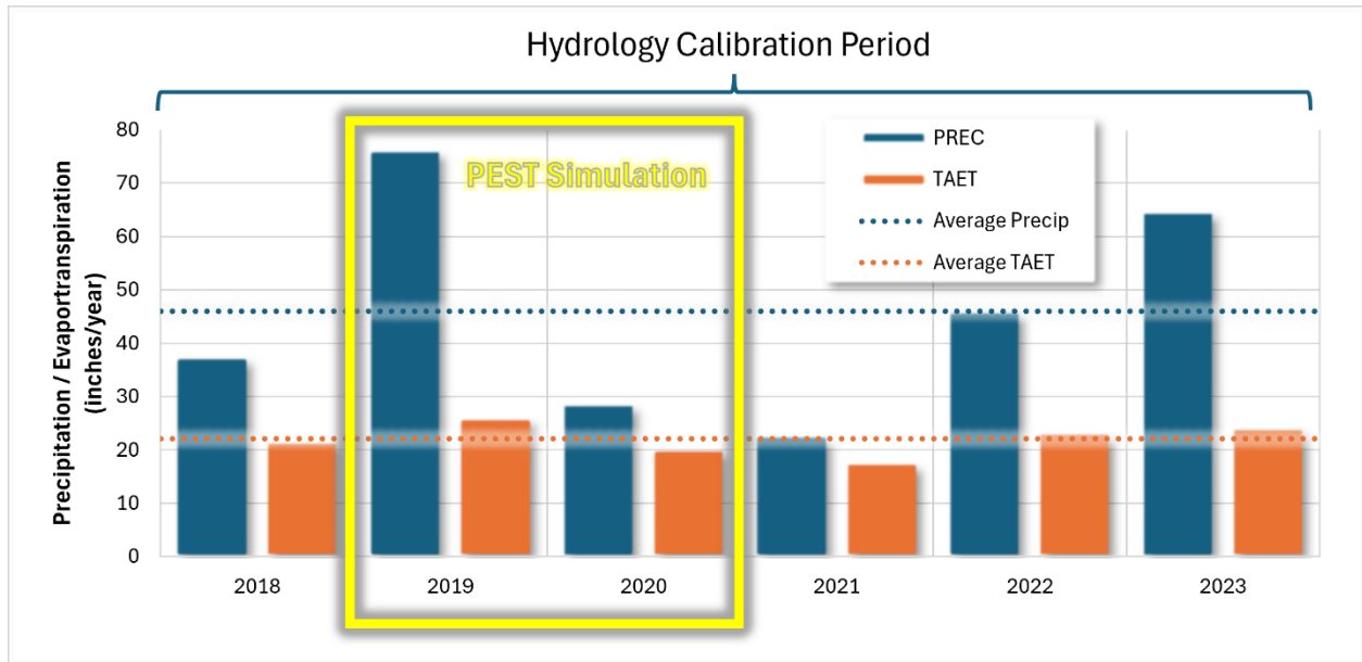
Figure 6-4. Annual average precipitation and evapotranspiration between water years 2018 – 2023, along with PEST simulation and hydrology calibration periods for the Gualala River South Fork at Sea Ranch watershed.
