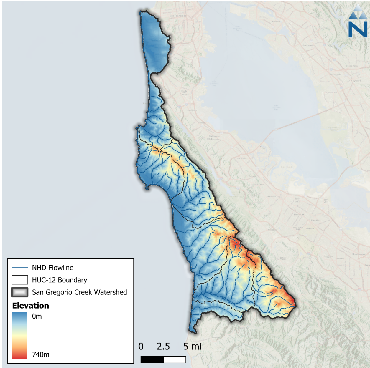
Figure 5-1. Digital elevation model of the San Gregorio Creek watershed.
