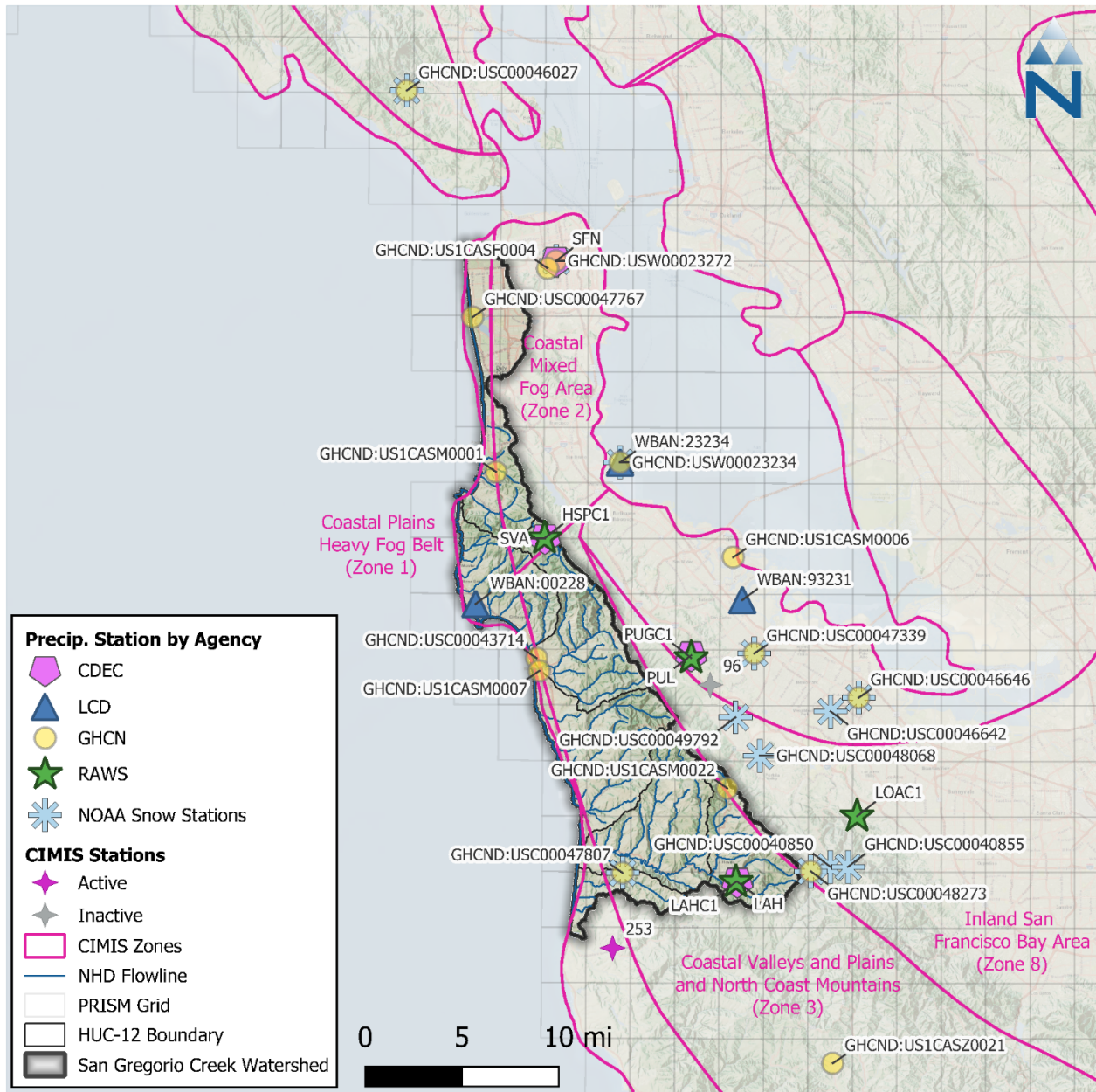
Figure 2-1. Identified rainfall stations and CIMIS ET Zones near the San Gregorio Creek watershed.
