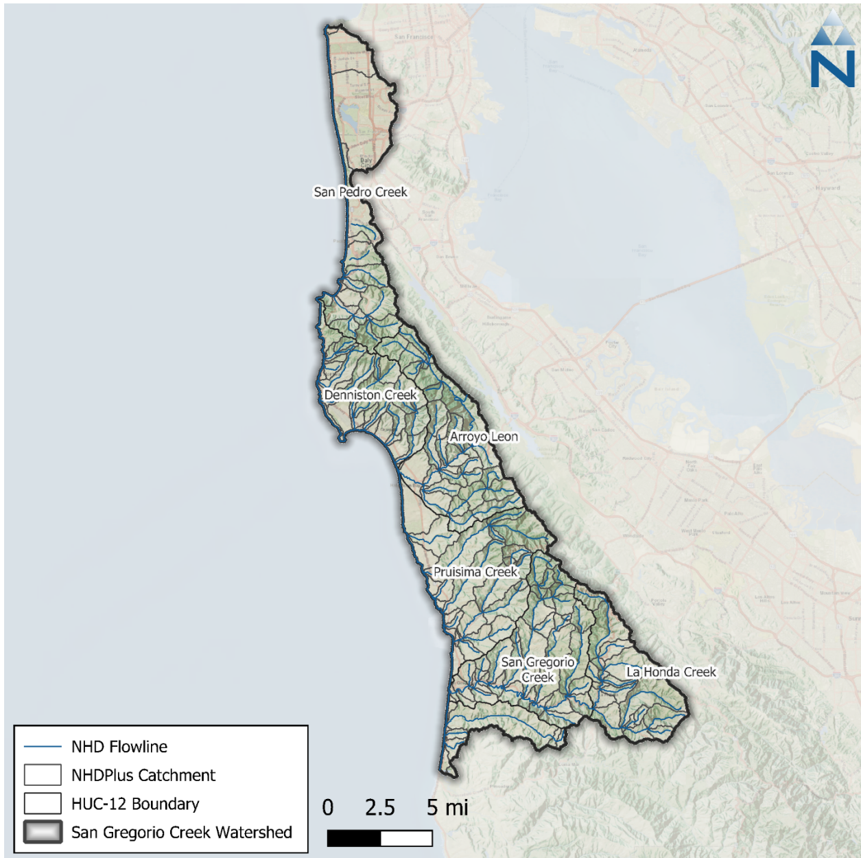
Figure 3-1. Initial catchment segmentation for the San Gregorio Creek watershed.
