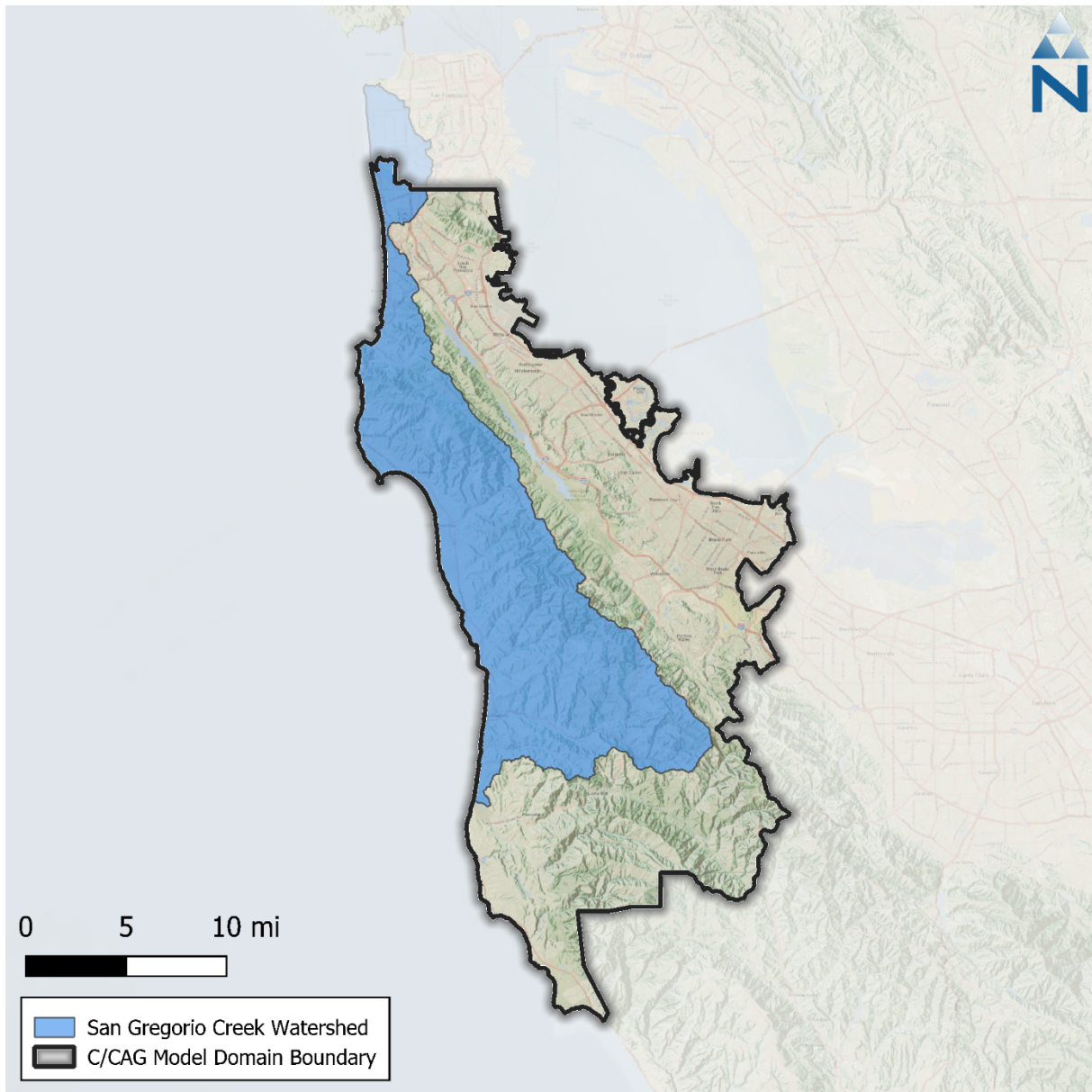
Figure 1-2. Map of the C/CAG regional model domain, which includes nearly all of the San Gregorio Creek watershed.
