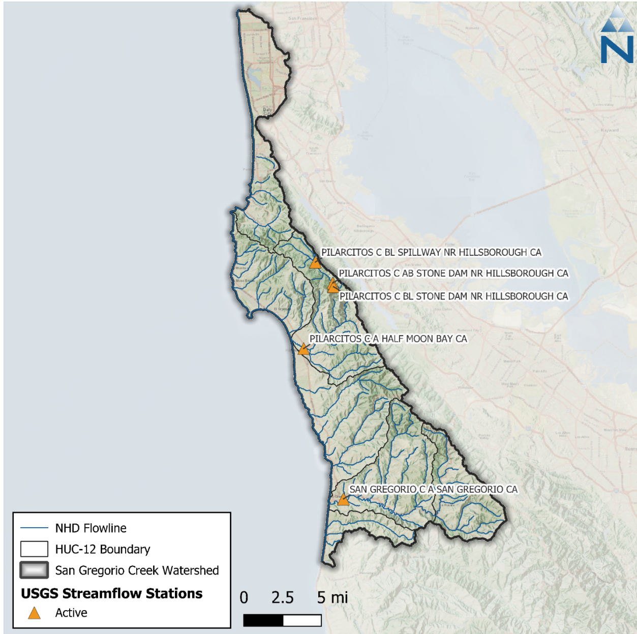
Figure 3-2. USGS streamflow stations in the San Gregorio Creek watershed.
