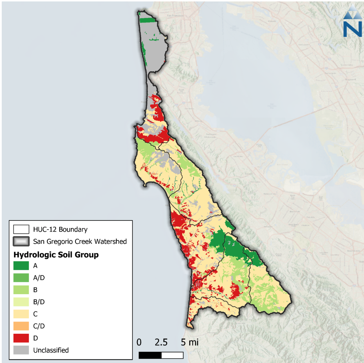
Figure 5-2. SSURGO hydrologic soil groups within the San Gregorio Creek watershed.
