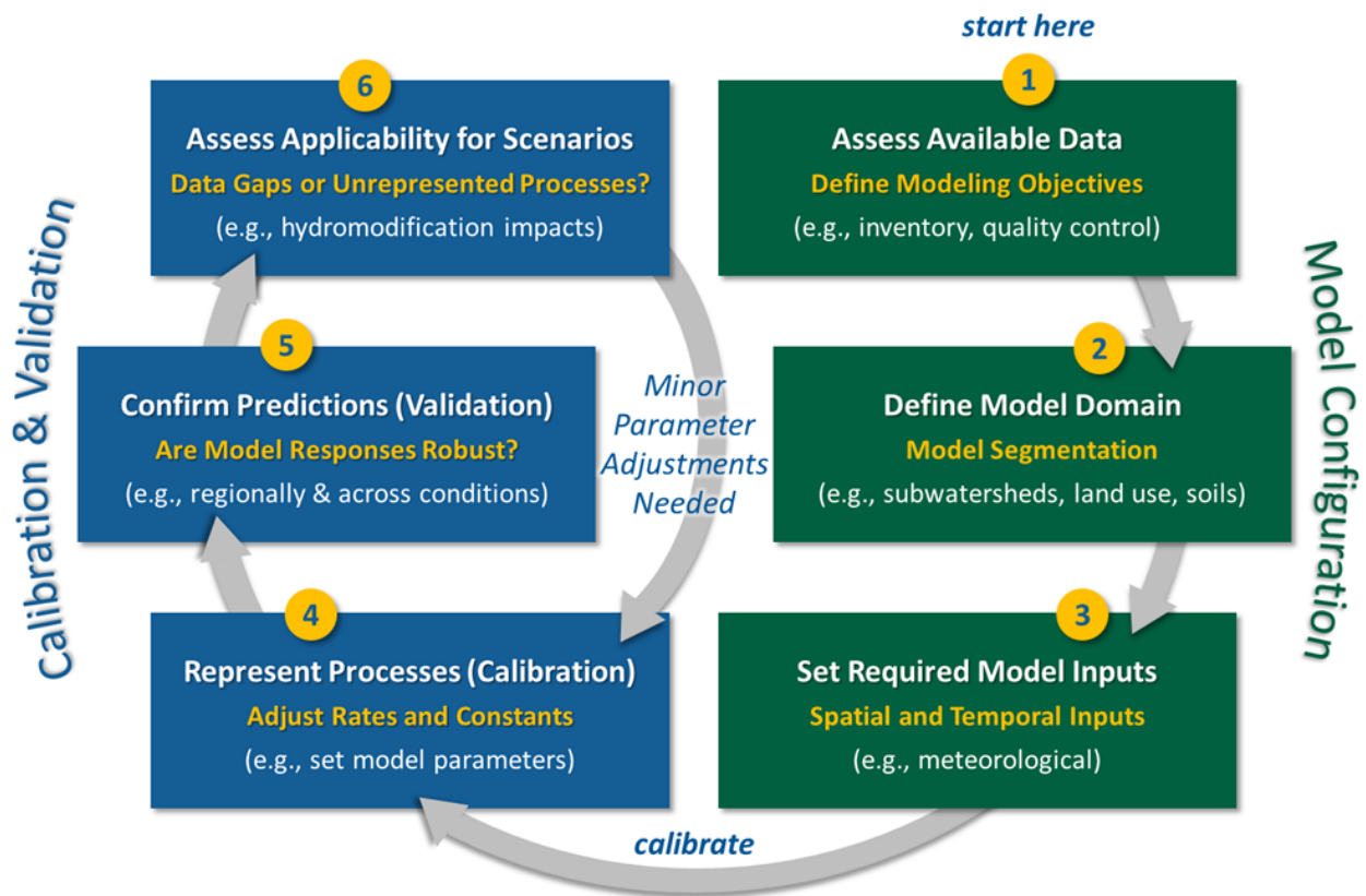
Figure 1-3. Conceptual schematic of model development cycle proposed for assessing instream flow needs in the San Gregorio Creek watershed.
