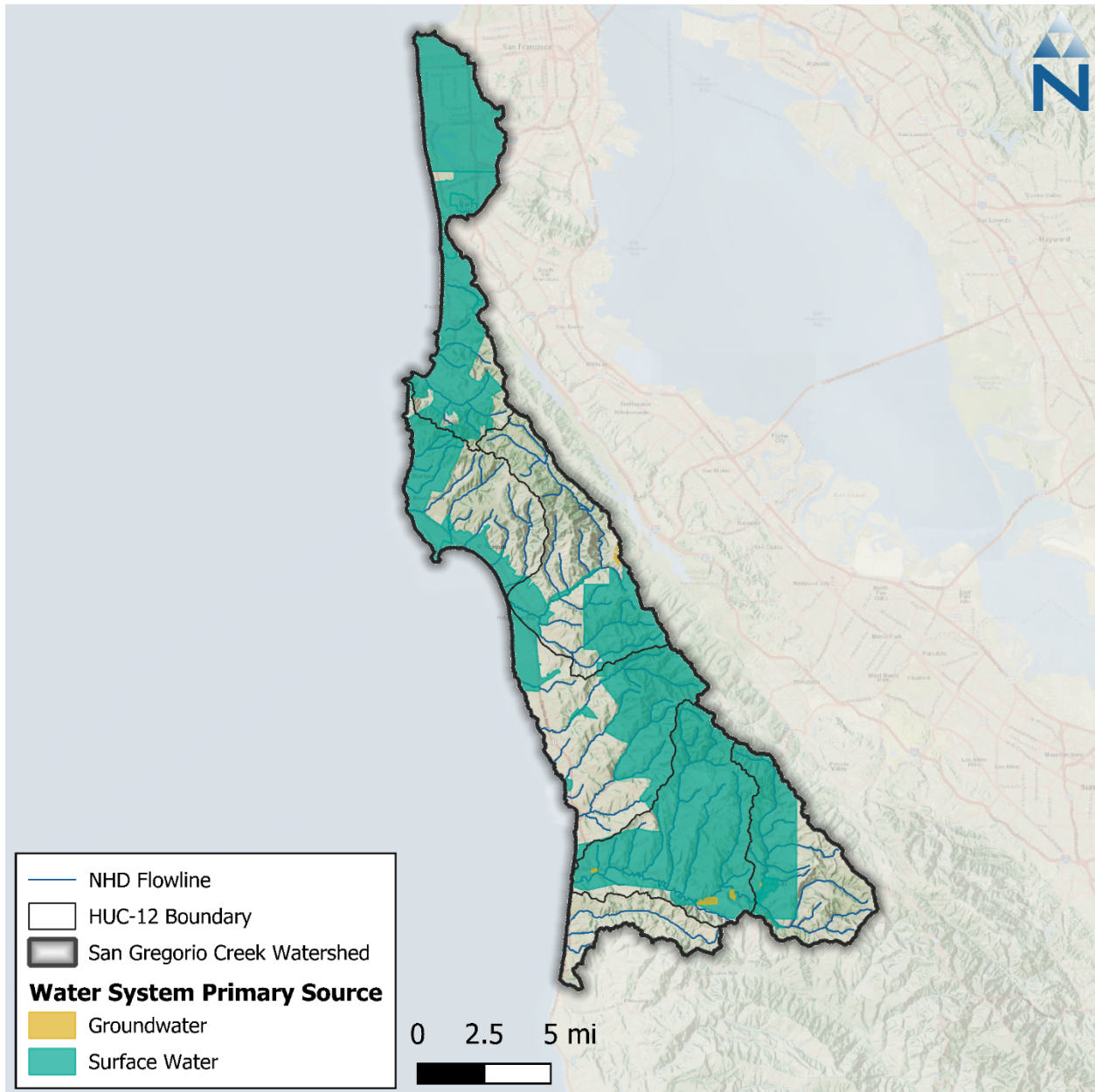
Figure 3-4. Primary Water System Sources in the San Gregorio Creek watershed.
