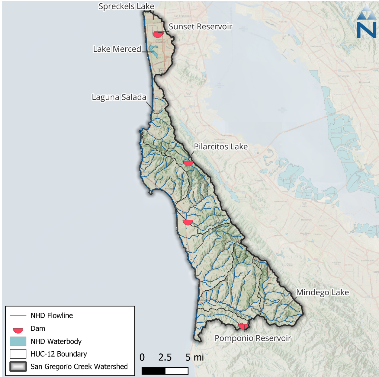
Figure 3-3. Dams within the San Gregorio Creek watershed relevant for watershed modeling effort (NID 2025).
