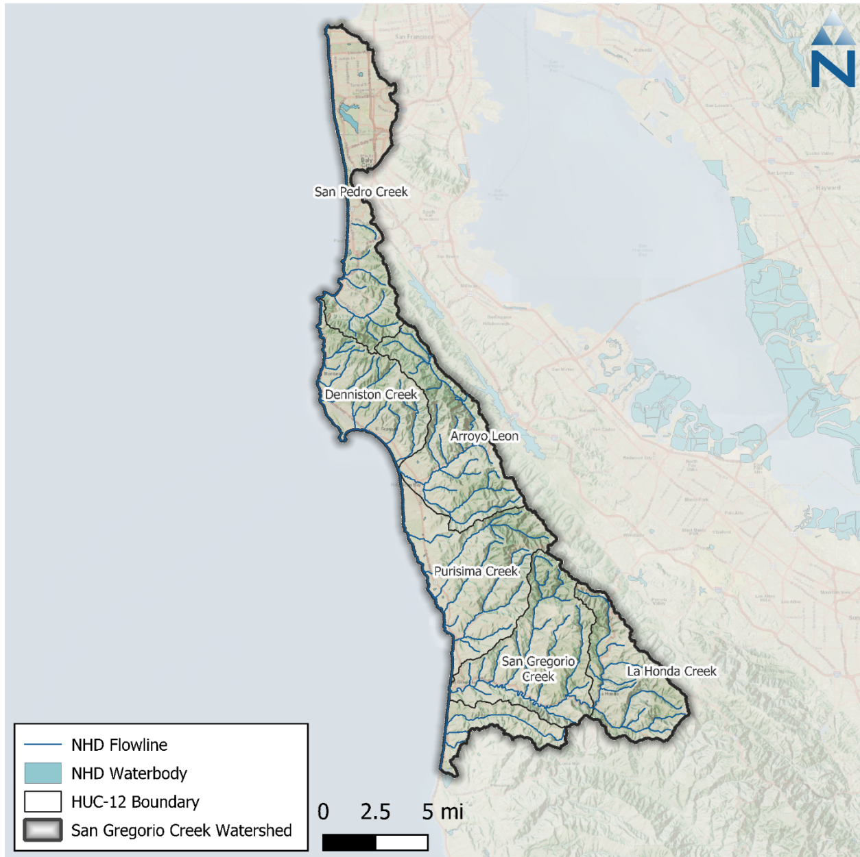
Figure 1-1. San Gregorio Creek watershed.
