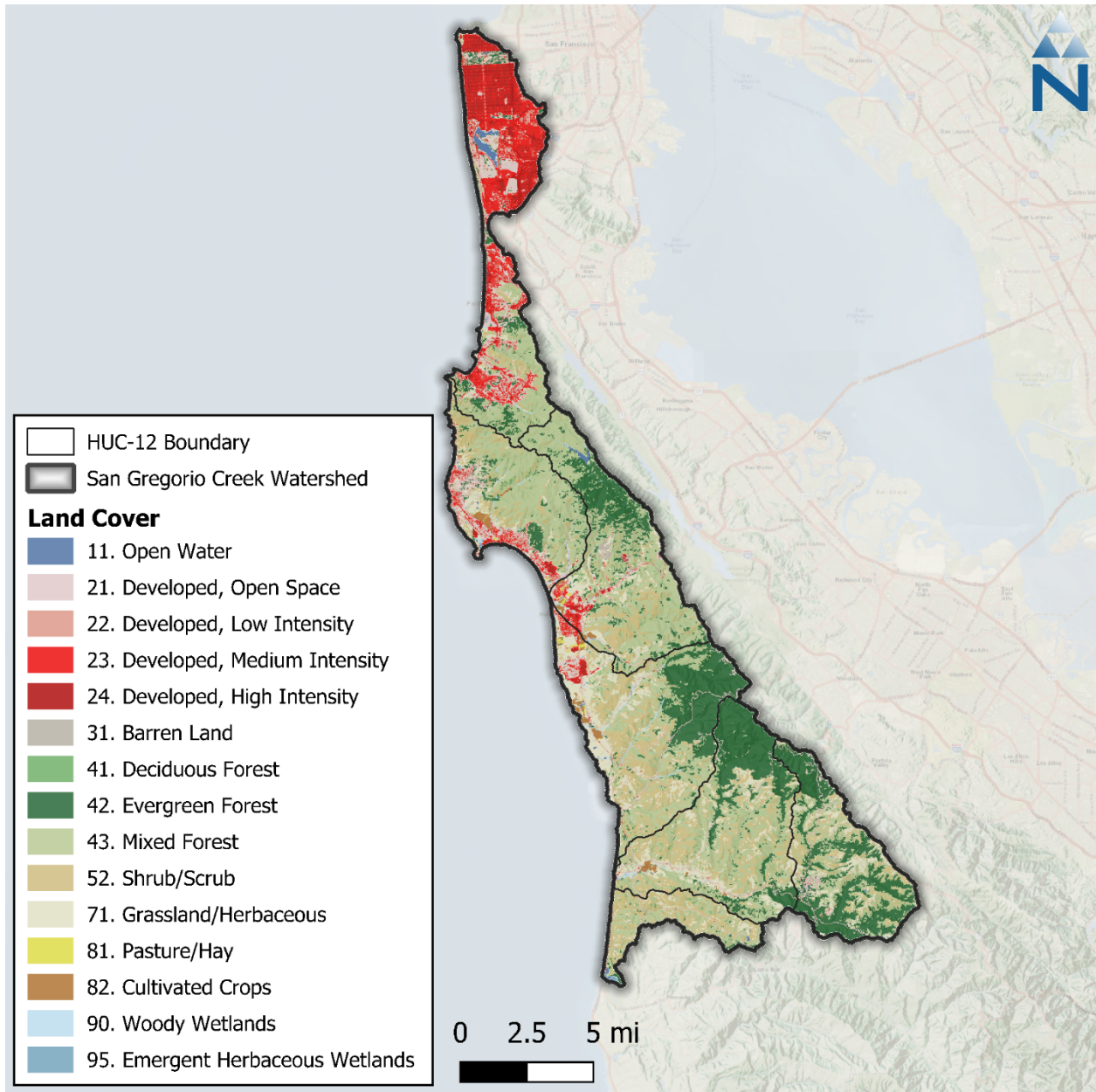
Figure 5-3. NLCD 2021 land cover within the San Gregorio Creek watershed.
