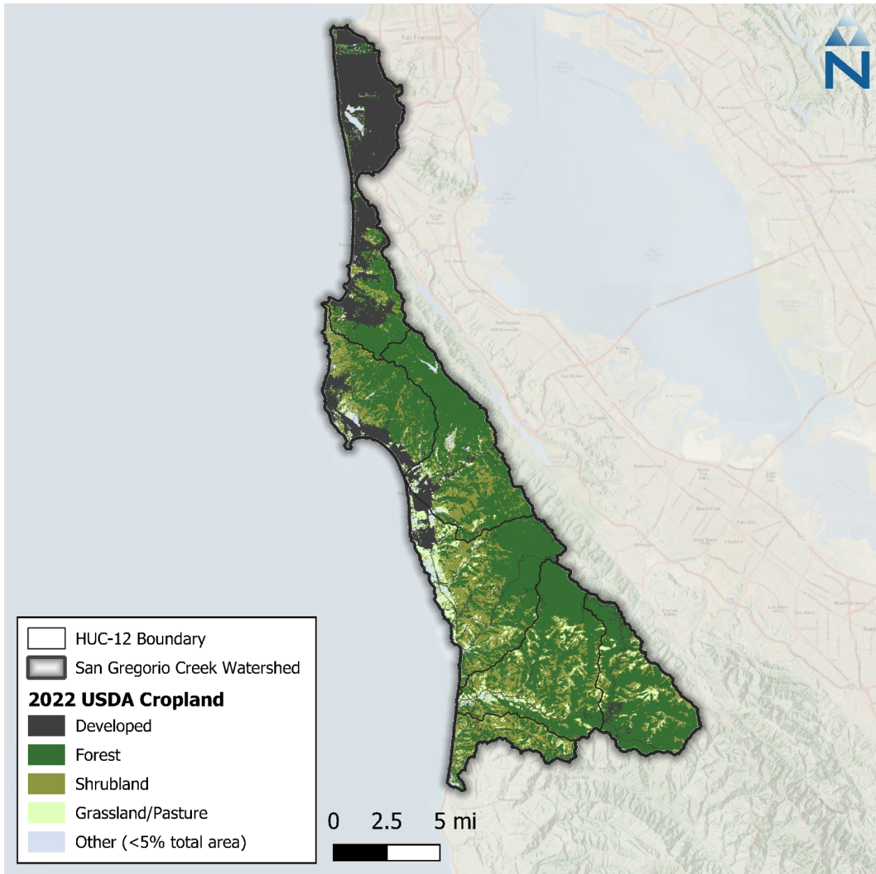
Figure 5-4. USDA 2022 Cropland Data within the San Gregorio Creek watershed
