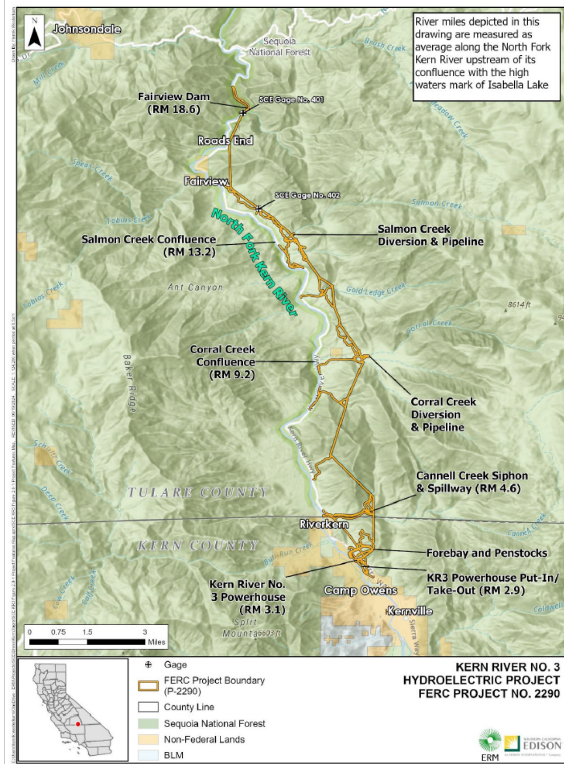
Kern River No. 3 Hydroelectric Project Location Map
