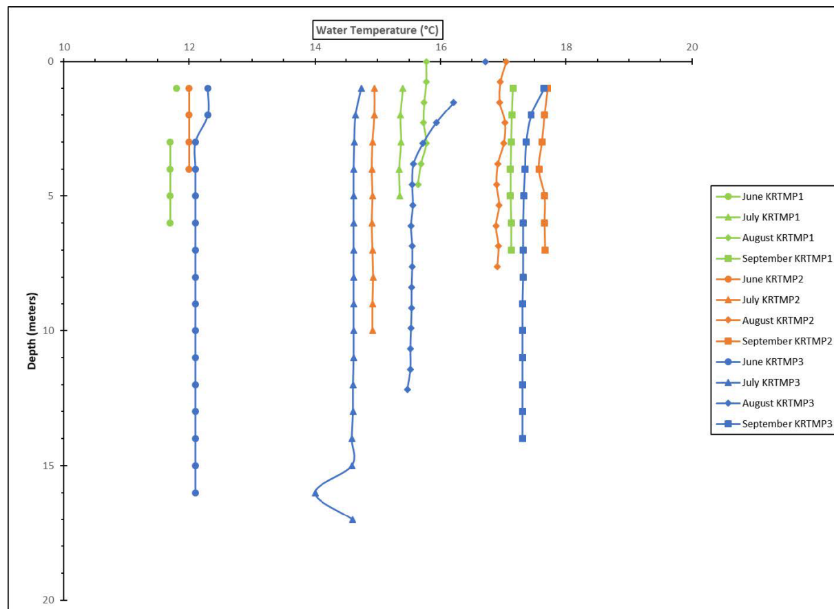
Figure 4.11-10: Water Temperature Profile Measured Monthly in Kerckhoff Reservoir at Stations KRTMP-1, KRTMP-2, and KRTMP-3 during June through September 2019
