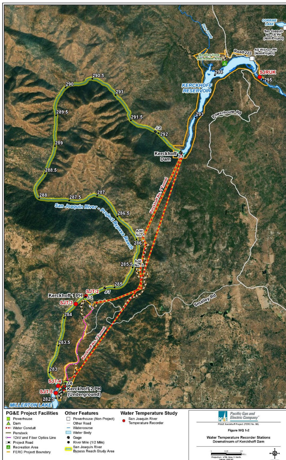
Figure 4.11-7: Study WQ 1 Water Temperature Monitoring Stations in the PBR
