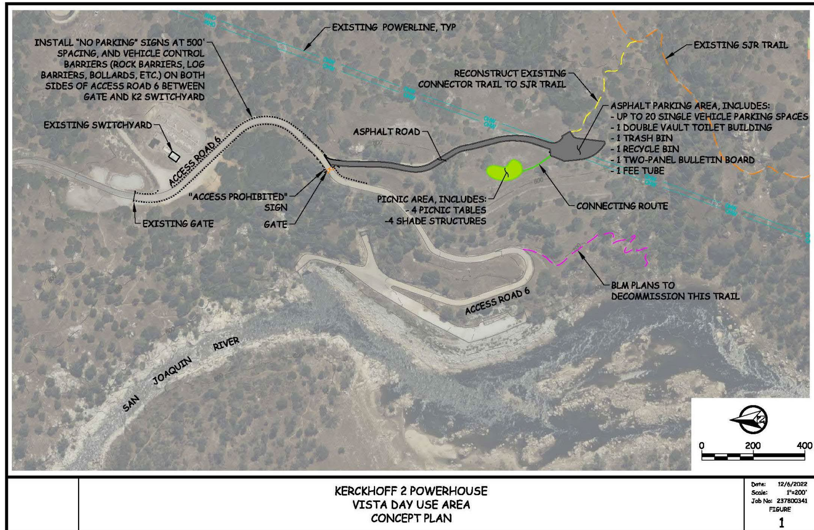
Figure 4.17-7: Conceptual Drawing for Planned Vista Day Use Area
