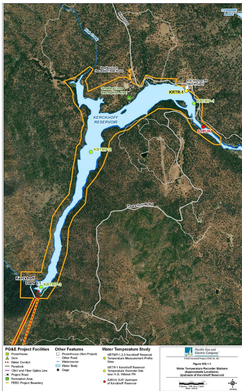
Figure 4.11-6: Study WQ 1 Water Temperature Monitoring Stations in Kerckhoff Reservoir
