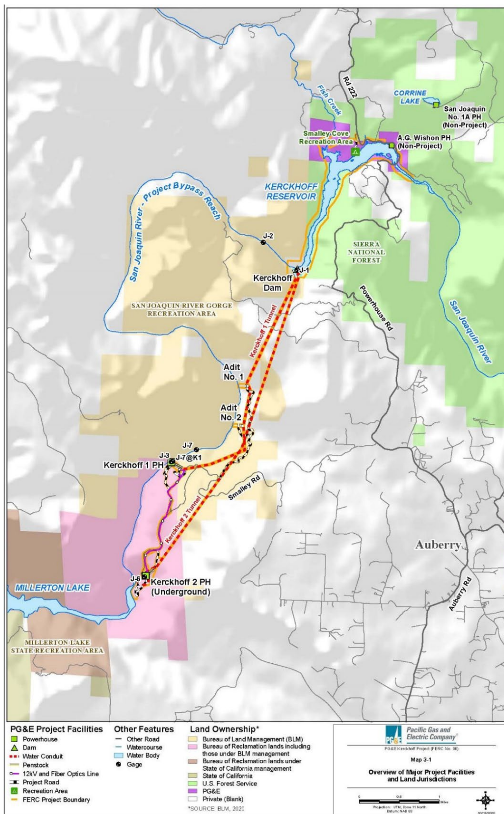
Figure 2.2-3: Overview of Major Project Facilities and Land Jurisdiction
