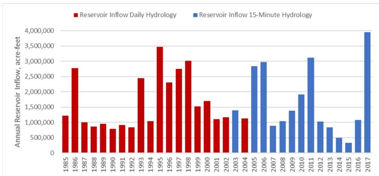
Figure 4.11-3: Annual Inflow with LTOR to Kerckhoff Reservoir under Baseline Conditions
