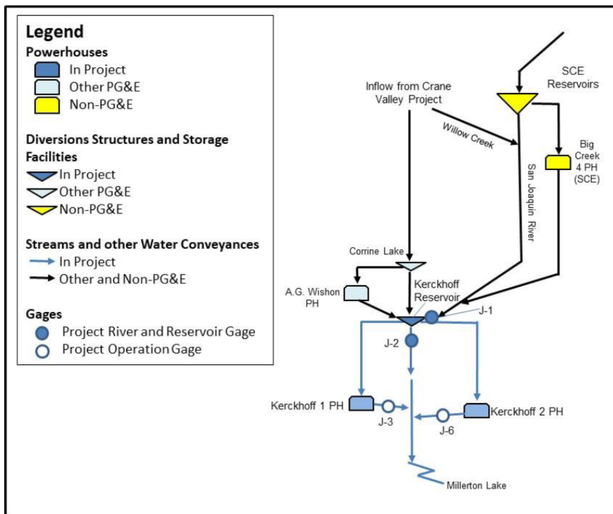
Figure 2.2-2: Project Schematic of Regional Flow and Gages
